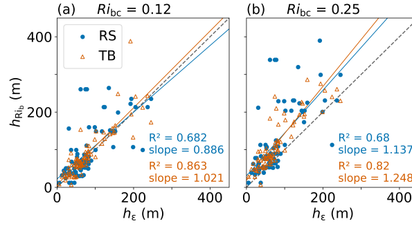
Figure 8. SML height comparisons between the bulk Richardson number approach h_{Rib} and turbulence h_{\epsilon} based on tethered balloon (TB, orange) and radiosonde (RS, blue) profiles. For both data sets, two different critical bulk Richardson numbers are used: 0.12 (a), and 0.25 (b). The dashed line represents the 1:1 line. Solid lines are the least squares fits for tethered balloon (orange) and radiosonde (blue) profiles; R^2 and slope values are given for each fit.
