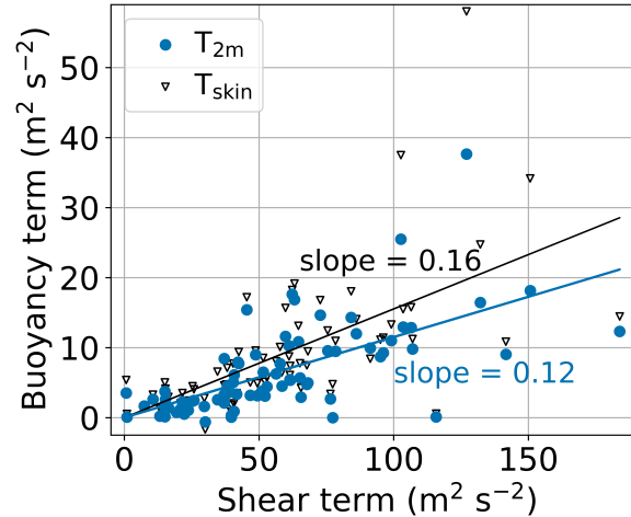
Figure 6. The buoyancy term versus shear term of the surface bulk Richardson number calculated according to Eq. 3 using the temperature at 2 m height T_{2\text{m}} (blue) and the skin temperature T_{\text{skin}} (black) as \theta_0 . The solid line indicates the least squares fit that is forced through the origin. The critical bulk Richardson number Ri_{\text{bc}} is equivalent to the slope of the fit. The critical values are 0.12 for T_{2\text{m}} and 0.16 for T_{\text{skin}} .
