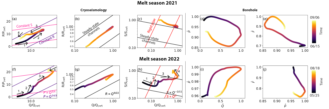
Figure 4. Relationships between two variables at the seasonal scale for the melt seasons 2021 and 2022. Color are scaled to the number of days in each melt seasons. (a) and (f) Relationships between scaled runoff ( Q/Q_{ref} ) and scaled turbulent-water-flow-induced seismic power ( P/P_{ref} ). The x -axis is in logarithmic scale. The superimposed lines show the relations derived by Gimbert et al. (2016) for a constant hydraulic gradient (pink lines, P \propto Q^{5/4} ) and for a constant hydraulic radius (purple curve, P \propto Q^{14/3} ). (b) and (g) Relationship between scaled runoff ( Q/Q_{ref} ) and scaled hydraulic radius ( R/R_{ref} ). Both x and y -axes are in logarithmic scale. Superimposed lines show the relations of steady-state preferential drainage axis evolution (Nanni et al. (2020), R \propto Q^{9/22} ). (c) and (h) Relationship between scaled runoff ( Q/Q_{ref} ) and scaled hydraulic gradient ( S/S_{ref} ). Both x and y -axes are in logarithmic scale. Superimposed lines show the relations of Nanni et al. (2020) for a preferential drainage axis at steady-state (black lines; S \propto Q^{-2/11} ) and for a preferential drainage axis evolving as a fixed cross sectional area channel referred to as rigid pipe (red line; S \propto Q^2 ). (d) and (i) Relationship between normalized water pressure and normalized runoff. (e) and (j) Relation between normalized force and normalized water pressure. Arrows indicate the direction of time and numbers refer to different periods described in the main text. The numbers do not correspond to the same periods between each panels and are unrelated to the periods identified by the circled numbers in Figure 3.
