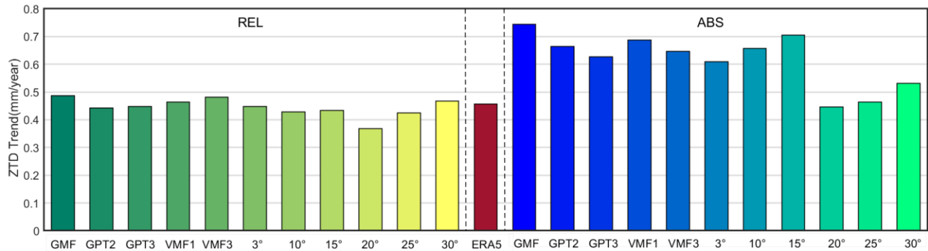
185 Figure 2: ERA5 trend (Red bar) and GPS ZTD trend derived from different processing strategies after ‘REL’ correction (Green bars) and ‘ABS’ correction (Blue bars) at STJO station.
