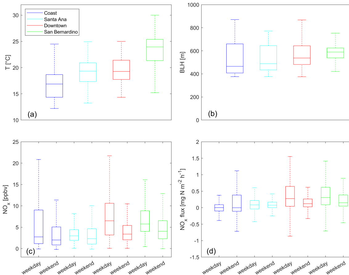
Figure 5. Boxplots for (a) the temperature, (b) the boundary layer height, (c) \text{NO}_x concentrations and (d) \text{NO}_x fluxes subdivided into four geographical sections according to Figure 1b (same color-code) and into weekday and weekend data. Blue colors represent the Coast, cyan colors the Santa Ana region, red colors Downtown Los Angeles and green colors the San Bernardino valley. Please note that outliers are not shown.
