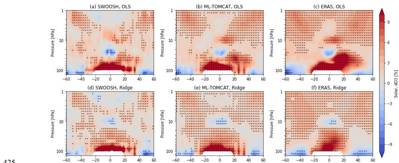
425 Figure 8: Latitude-pressure cross sections of solar cycle response in stratospheric ozone (%) derived from SWOOSH, ML-TOMCAT, and TOMCAT simulation ERA5 based on (a-c) OLS and (d-f) Ridge regression methods. The stippling indicates regions that are significant at the 95 % level.
