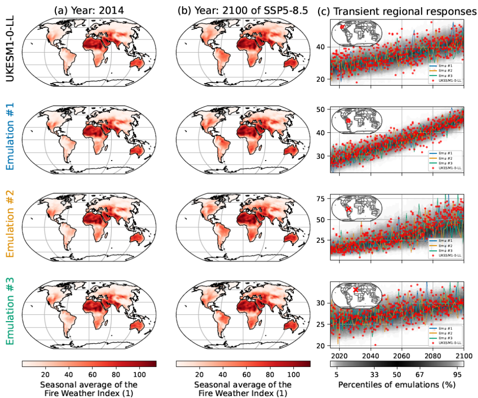
285 Figure 2: Examples of results for the emulations of the seasonal average of the FWI ( FWI_{sa} ) under UKESM1-0-LL. The left column (a) represents maps of FWI_{sa} in 2014 according to UKESM1-0-LL on the first row, while the three following rows correspond to three emulations chosen randomly in the full set. The middle column (b) reproduces the same structure, although in 2100 of SSP5-8.5. The third 290 column (c) shows time series of UKESM1-0-LL, the three emulations used for maps, but also the full spread of the emulations (shaded area). The rows correspond from top to bottom to the West of North America, the North of South America, a grid point in Amazonia close to Manaus and a grid point in Portugal close to Lisbon.
