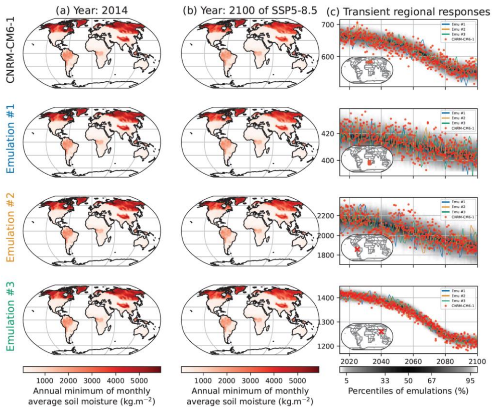
555 Figure 12: Similar to Figure 2 , although for the annual minimum of the monthly average of soil moisture ( SMmm ) under CNRM-CM6-1. The rows correspond from top to bottom to the West & Central Europe, the West of South Africa, a grid point in the west of Brazil in Acre and a grid point in Sichuan close to Chengdu.
