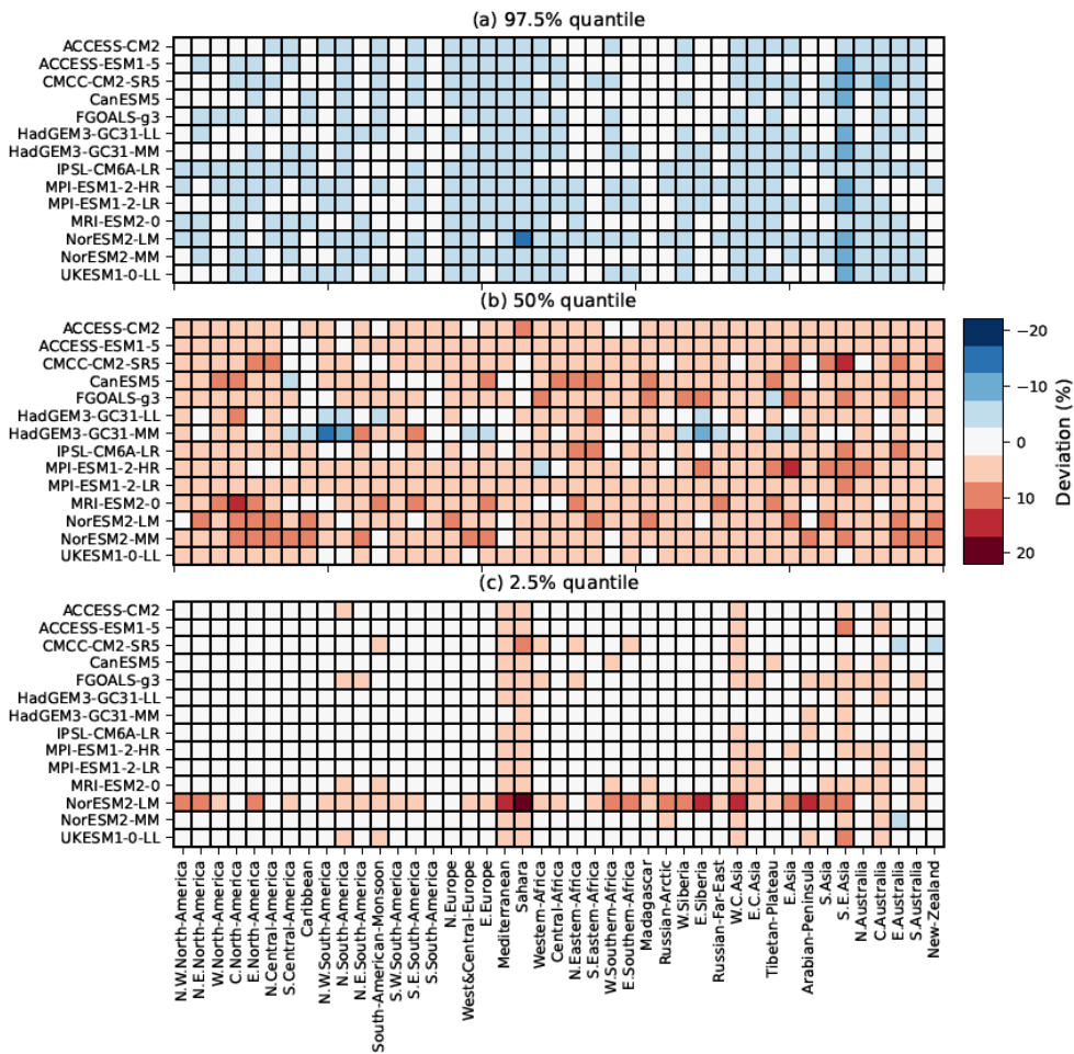
400 Figure 6: Similar to Figure 3 , although for the number of days with extreme fire weather ( FW1xd ).
