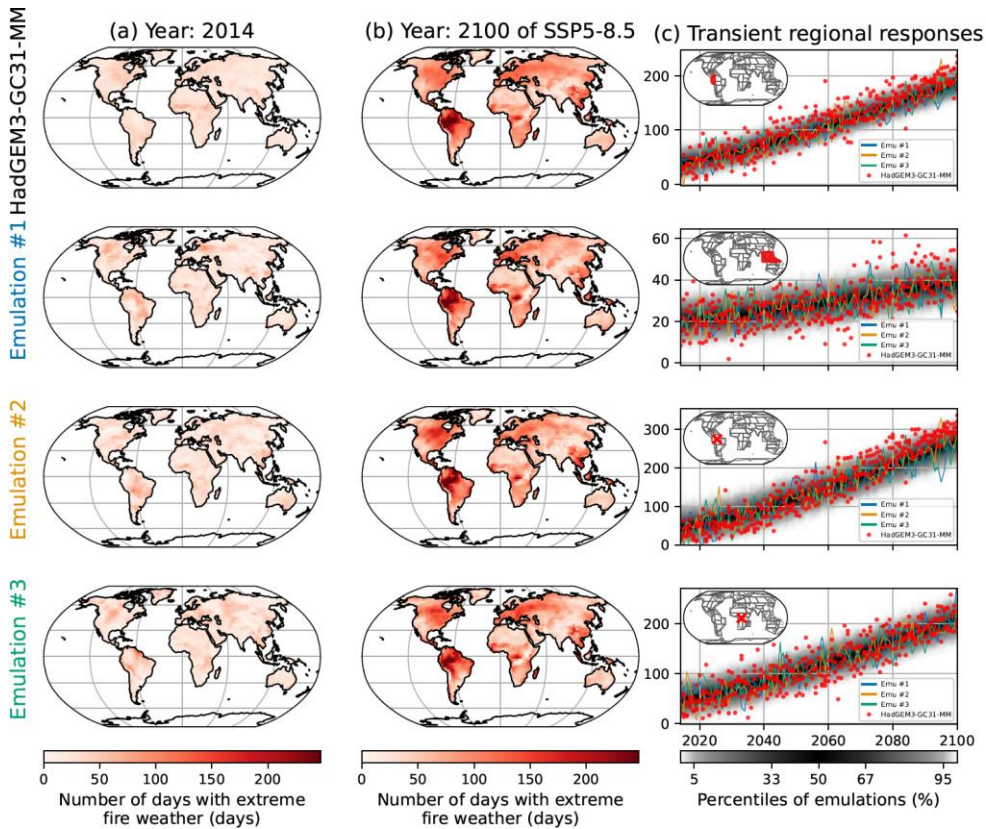
Figure 5: Similar to Figure 2 , although for the number of days with extreme fire weather ( FWIxd ) under HadGEM3-GC31-MM. The rows correspond from top to bottom to the North-West of South America, South-East Asia, a grid point in Amazonia encompassing the Jaú National Parc and a grid point in Democratic Republic of Congo encompassing the Salonga National Park.
