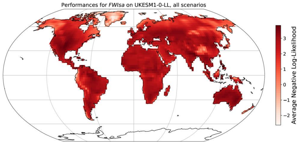
690 Figure A. 7: Negative log-likelihood obtained during training of MESMER-X on FWI_{sa} using the configuration presented in equation (10) and for the ESM used in Figure 2 .
