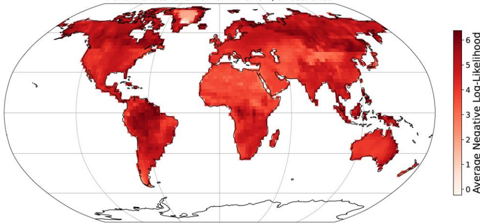
Figure A. 9: Negative log-likelihood obtained during training of MESMER-X on SM using the configuration presented in equation (12) and for the ESM used in Figure 9 Figure-9 .
