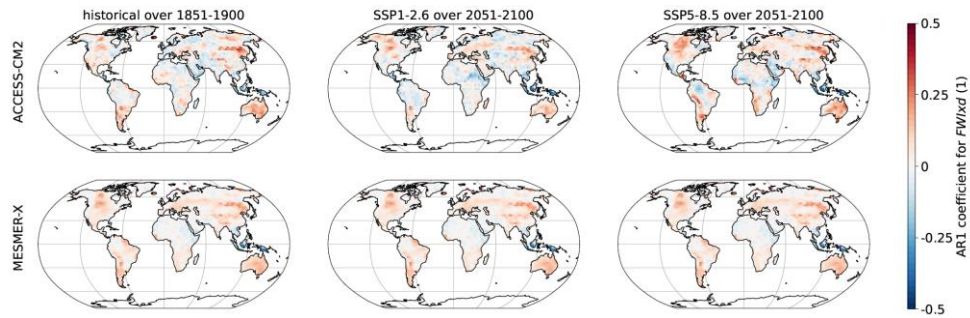
660 Figure A. 3: First order coefficient of a temporal auto-regressive process for FWI_{xd} with ACCESS-CM2 and MESMER-X using the configuration presented in equation (11).
