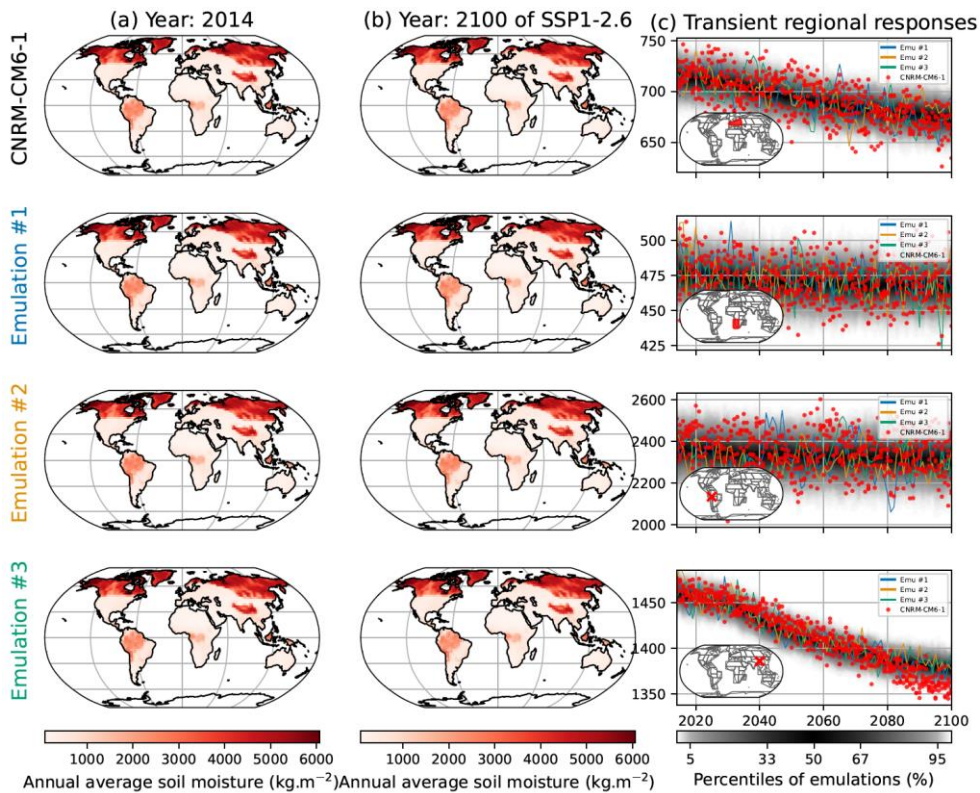
745 Figure A. 16: Similar to Figure 9 , although with the low warming scenario SSP1-2.6.
