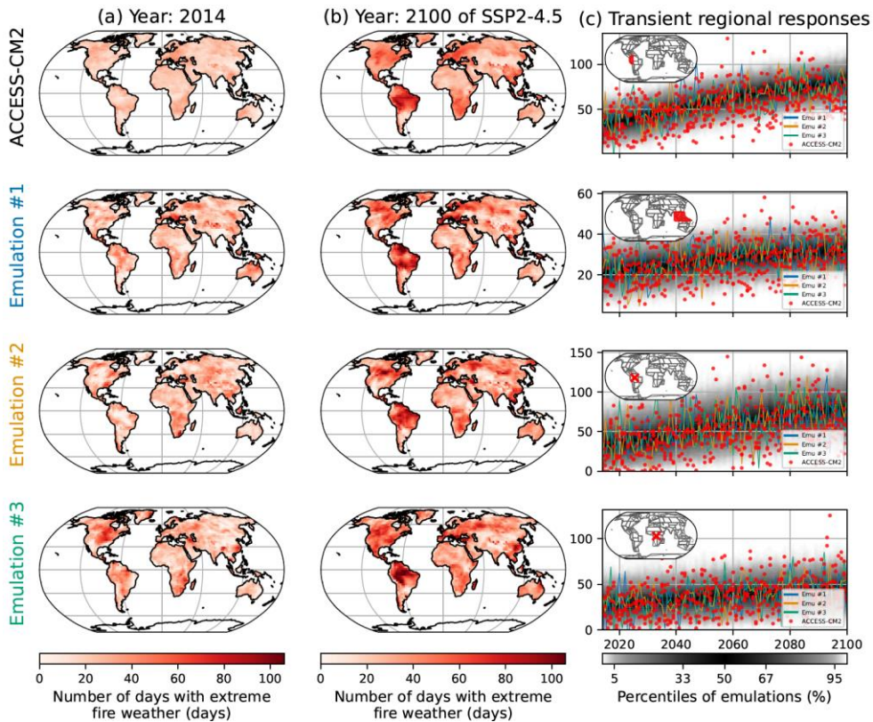
725 Figure A. 13: Similar to Figure 5 , although with ACCESS-CM2 and the mid warming scenario SSP2-4.5.
