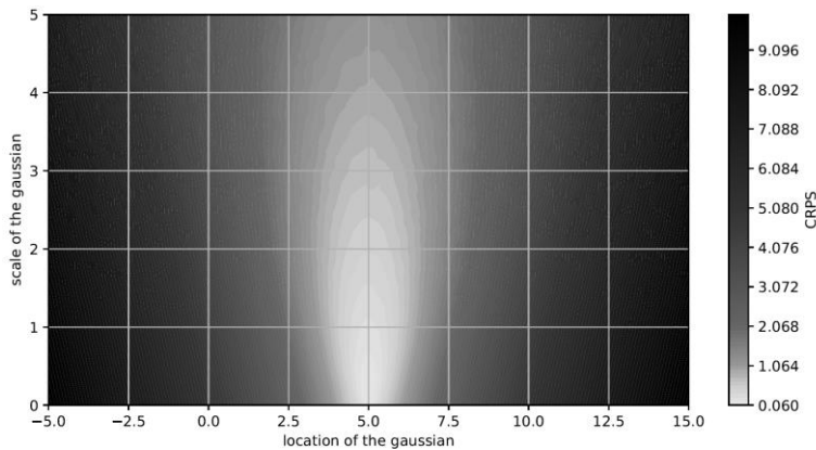
680 Figure A. 6: CRPS obtained with an observed value of 5 and gaussian distributions sampled over 10.000 members over different values of its parameters.
