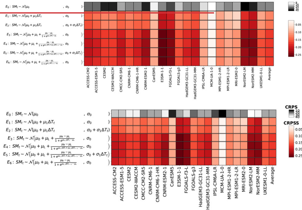
Figure 8: Similar to Figure 1 , although for the annual average soil moisture ( SM ).
