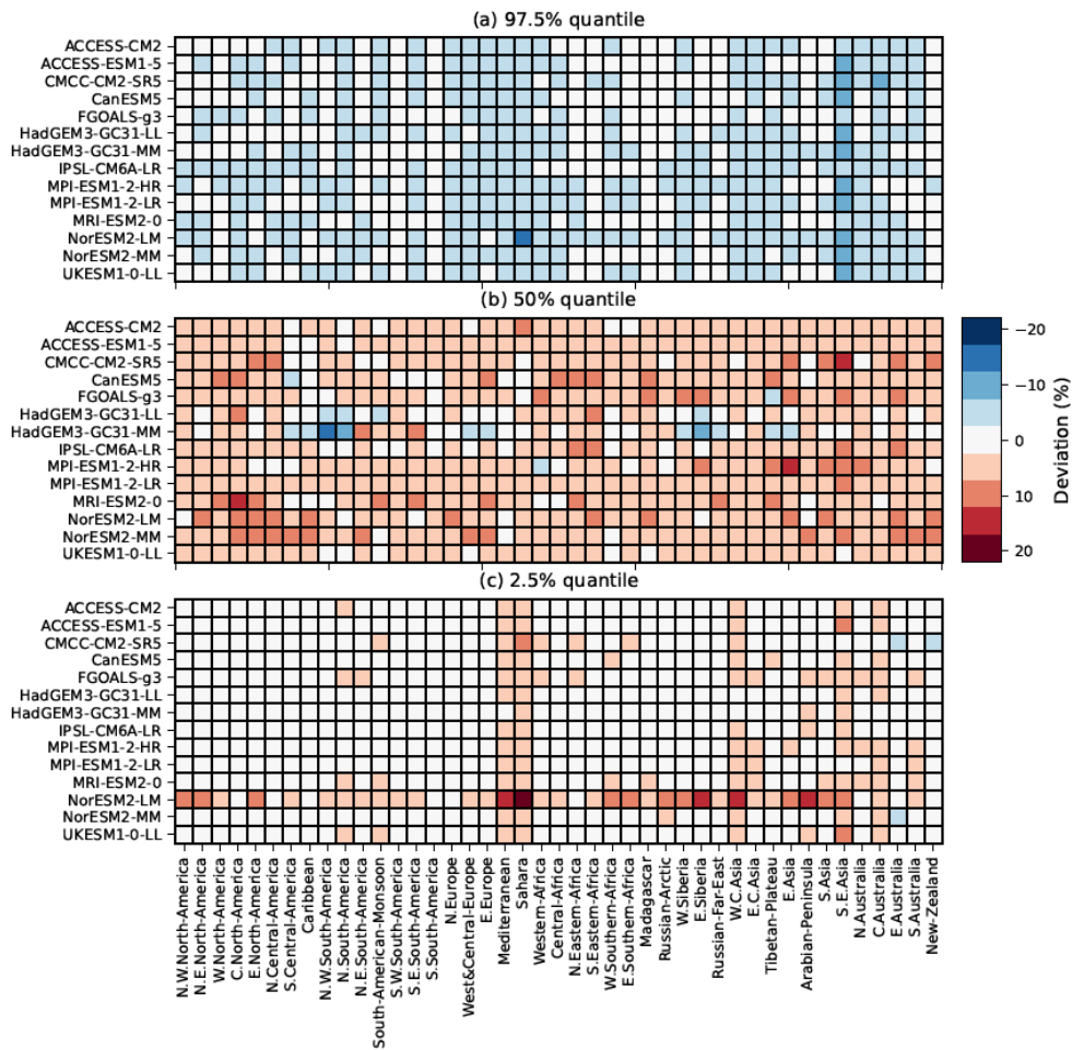
395 | Figure 6: Similar to Figure 3 , although for the number of days with extreme fire weather ( FW1xd ).
