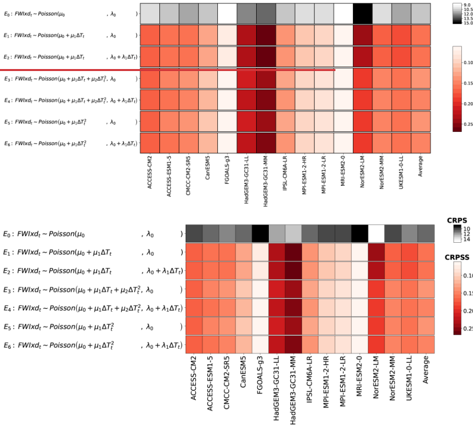
Figure 4: Similar to Figure 1, although for the number of days with extreme fire weather ( FWIXd ).
