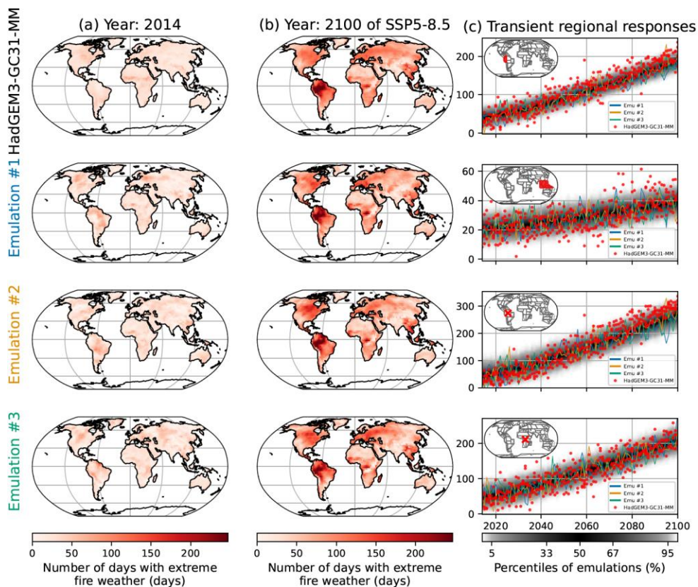
360 Figure 5: Similar to Figure 2 , although for the number of days with extreme fire weather ( FWIxd ) under HadGEM3-GC31-MM. The rows correspond from top to bottom to the North-West of South America, South-East Asia, a grid point in Amazonia encompassing the Jaú National Parc and a grid point in Democratic Republic of Congo encompassing the Salonga National Park.
