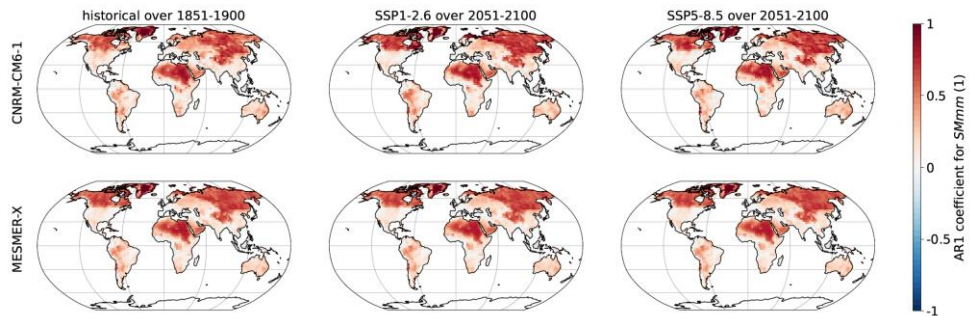
665 Figure A. 5: First order coefficient of a temporal auto-regressive process for SMmm with CNRM-CM6-1 and MESMER-X using the configuration presented in equation (13).
