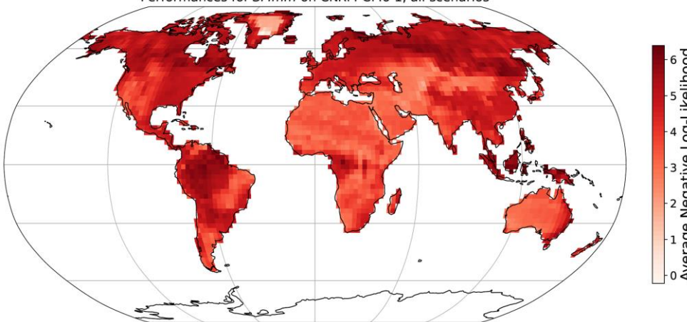
Figure A. 10: Negative log-likelihood obtained during training of MESMER-X on SMmm using the configuration presented in equation (13) and for the ESM used in Figure 12.
