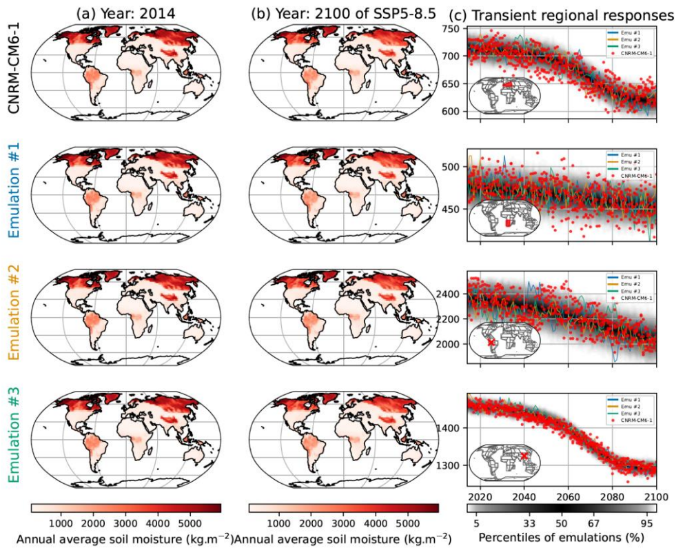
490 Figure 9: Similar to Figure 2 , although for the annual average soil moisture ( SM ) under CNRM-CM6-1. The rows correspond from top to bottom to the West & Central Europe, the West of South Africa, a grid point in the west of Brazil in Acre and a grid point in Sichuan close to Chengdu.
