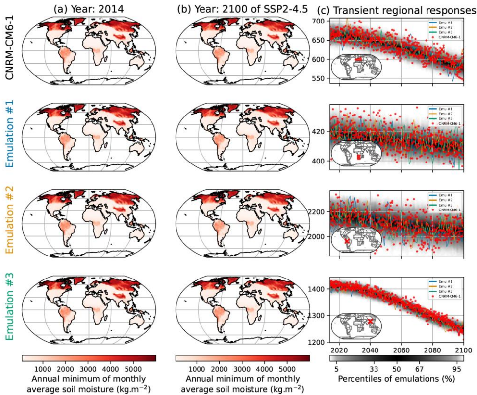
755 Figure A. 17: Similar to Figure 12, although with the mid warming scenario SSP2-4.5,
