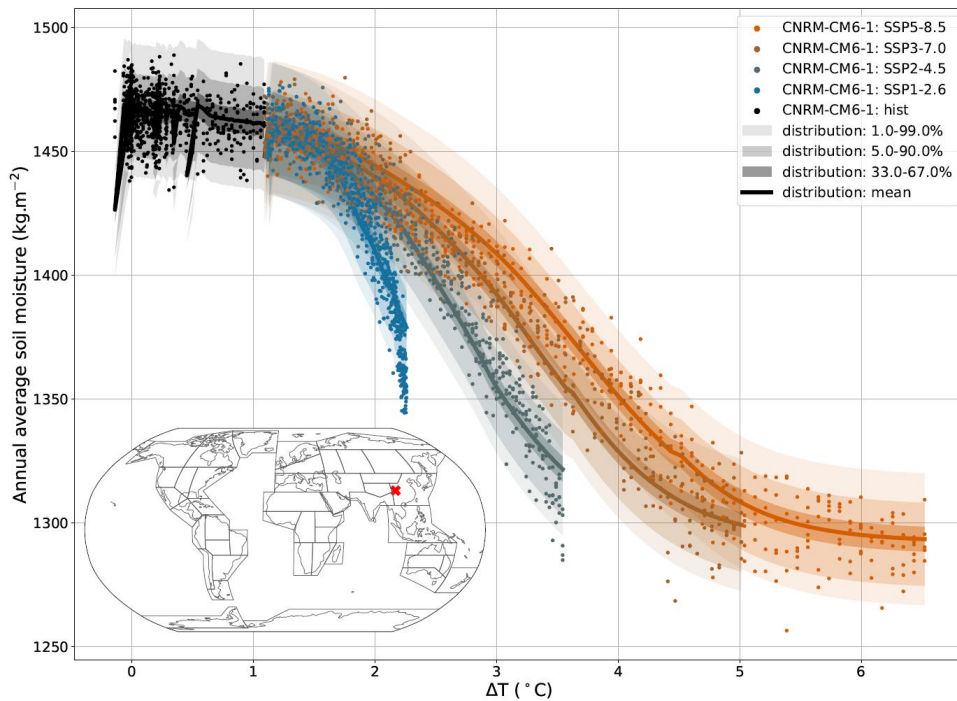
Figure 7: Example of local response of the annual average soil moisture ( SM ) to \Delta T under CNRM-CM6-1. The grid point is in Sichuan, in the vicinity of Chengdu, the same one shown in Figure 9 , column (c), fourth row. The distribution shown follows the configuration E_4 described in equation (12).
