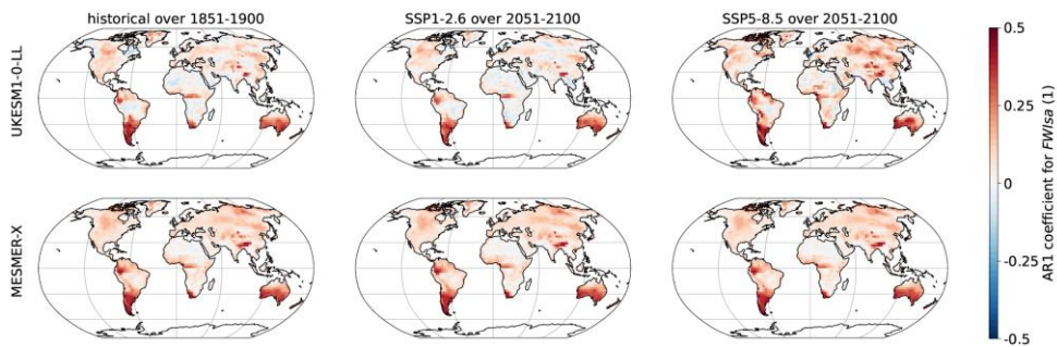
Figure A. 2: First order coefficient of a temporal auto-regressive process for FWIsa with UKESM1-0-LL and MESMER-X using the configuration presented in equation (10).
