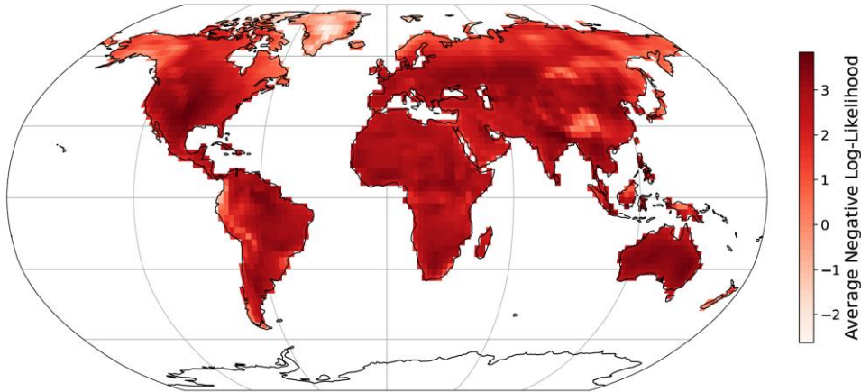
Figure A. 7: Negative log-likelihood obtained during training of MESMER-X on FWI_{sa} using the configuration presented in equation (10) and for the ESM used in Figure 2.
