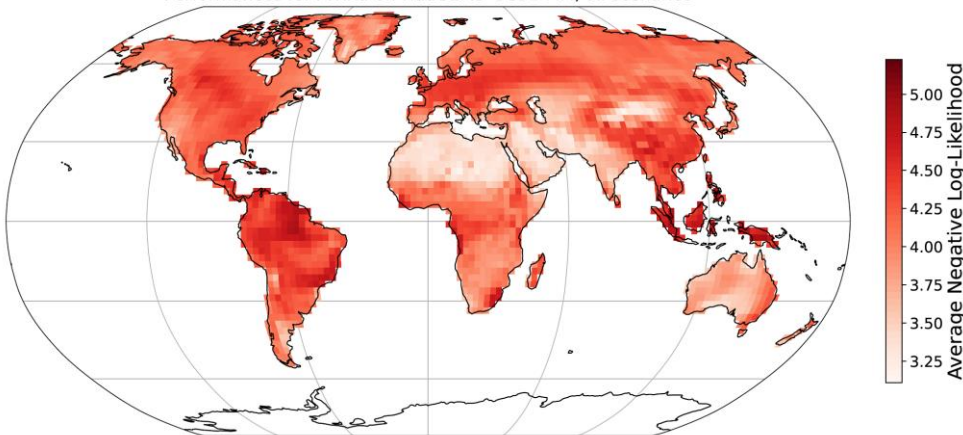
Figure A. 8: Negative log-likelihood obtained during training of MESMER-X on FWI_{xd} using the configuration presented in equation (11) and for the ESM used in Figure 5.
