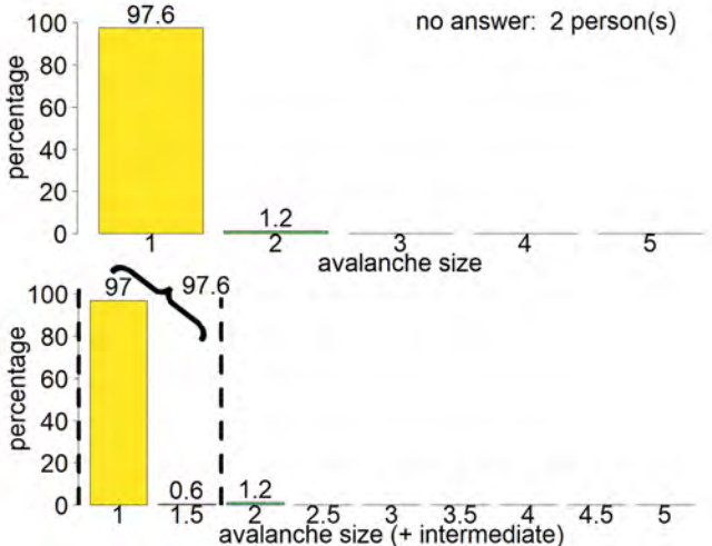
Figure 3. Distribution of the size classes and the intermediate sizes assigned to avalanche avalanches / picture pictures (gd) to (jf) in the survey.
