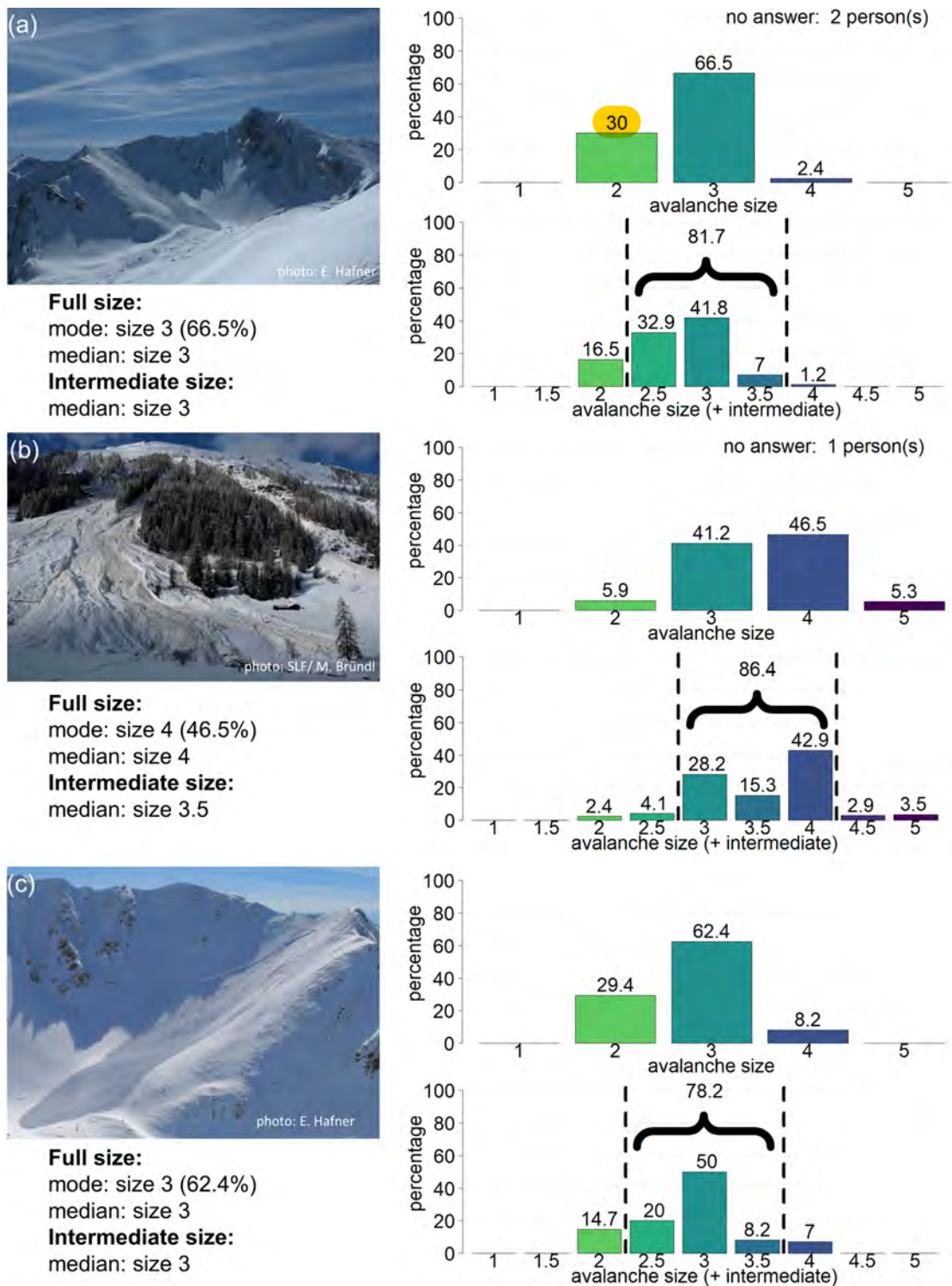
Figure 2. Distribution of the size classes and the intermediate sizes assigned to avalanche avalanches / picture pictures (a) to (f) in the survey.
