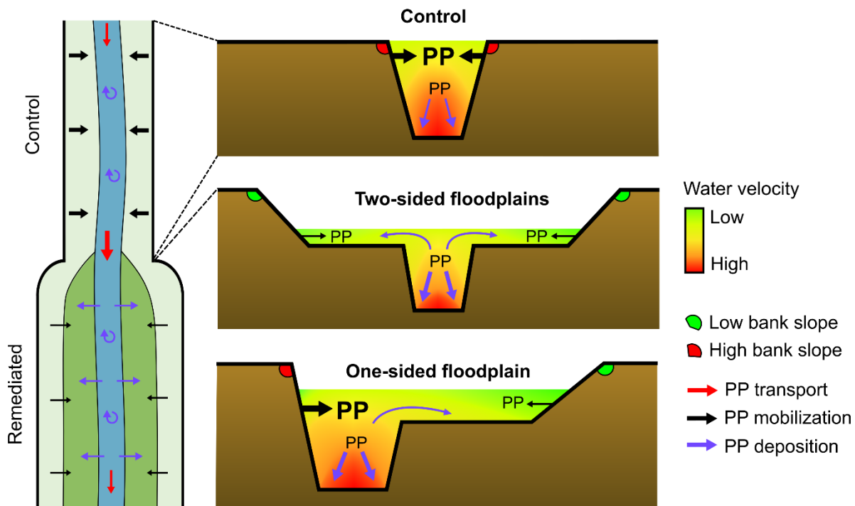
610 Fig. 1. Conceptual model of fluvial processes that determine particulate phosphorus (PP) export in remediated vs. control streams. Deposition of PP occur on channel beds predominantly during lower flows when transport capacity are lower than sediment delivery. During inundation, PP deposition dominates on floodplains, due to lower water velocities. In two-sided floodplains, streambanks are stabilized during higher flows due to their lower slopes and lower shear stress from water forces compared to the inset channel. In 615 one-sided designs, one streambank is steeper and exposed to higher water velocities in the channel, resulting in higher mobilization and transport of PP.
