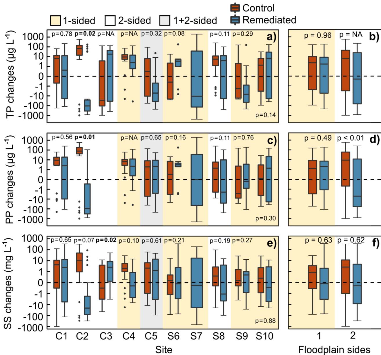
640 Fig. 3. Changes in TP, PP and SS concentrations (note log 10 y-axis) between start and end of control streams (red boxes) and start 645 and end of remediated streams (blue boxes) from April 2020 to June 2022. Changes in concentrations are shown a, c, e) by each site (C1–5 and S6–10) and b, d, f) sites grouped by number of floodplain sides along inset channel. When comparing floodplain sides, two sites were excluded due to lack of control stream (S7) and a combination of one- and two-sided floodplains along the reach (C5). P-values of permuted unpaired t-tests are shown within the panels. P-values of parametric and, when necessary, permuted paired t-tests are shown within the panels. P values = NA refers to non-normal and autocorrelated data that prevent reliable computation of t-tests. Bold font denotes significant difference ( p < 0.05 ) between locations.
