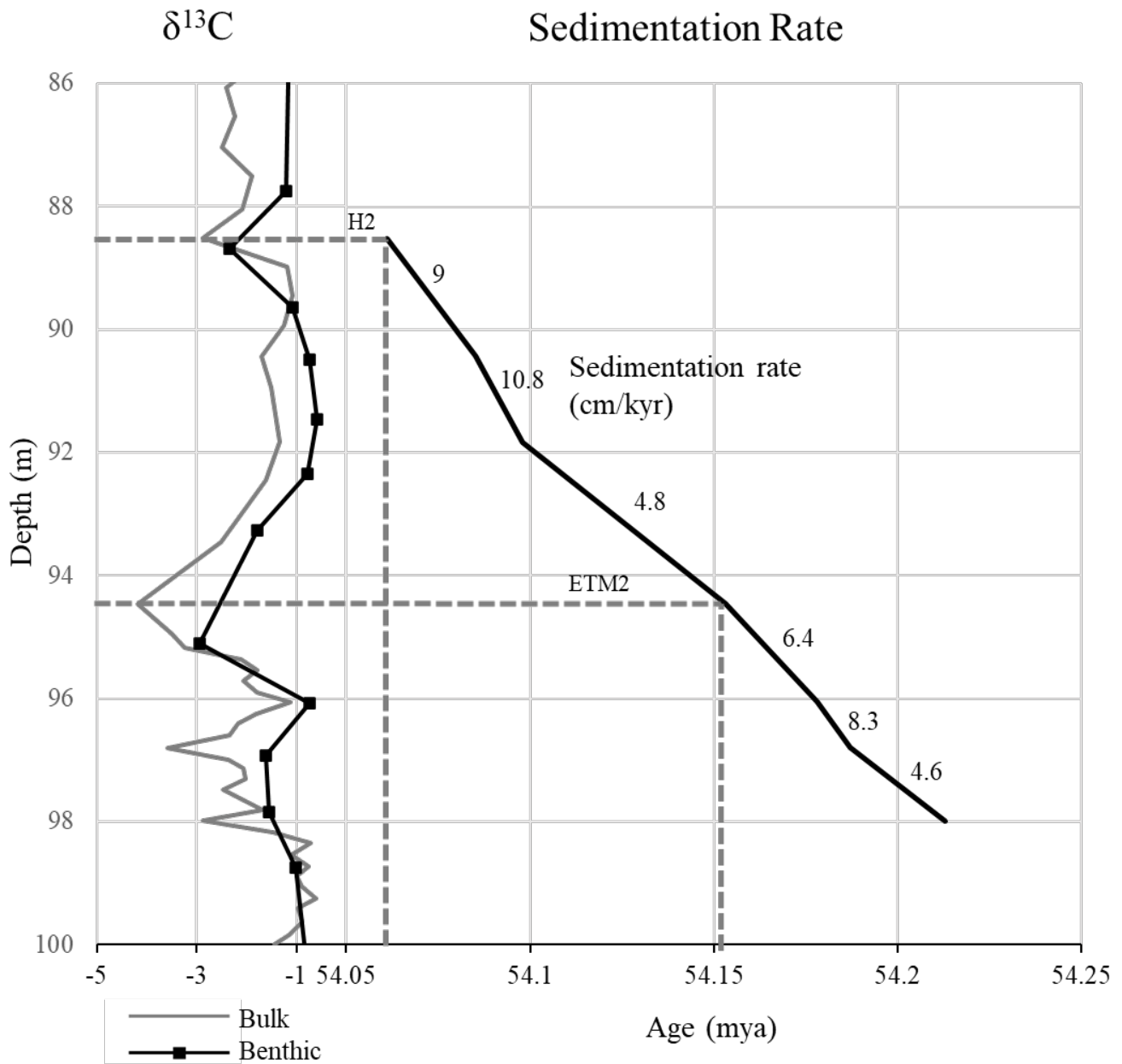
850 Figure 6: Sedimentation rates in the Knapps Narrows core based on correlations of \delta^{13}\text{C} inflection points to the age model of Lauretano et al., 2015 at Walvis Ridge Site 391. Sedimentation rates in cm/kyr. Note relative consistency compared to orders of magnitude changes that were documented during the PETM in Stassen et al. (2012b), with moderate increases beginning at 91.8 m, consistent with cyclostratigraphy.
