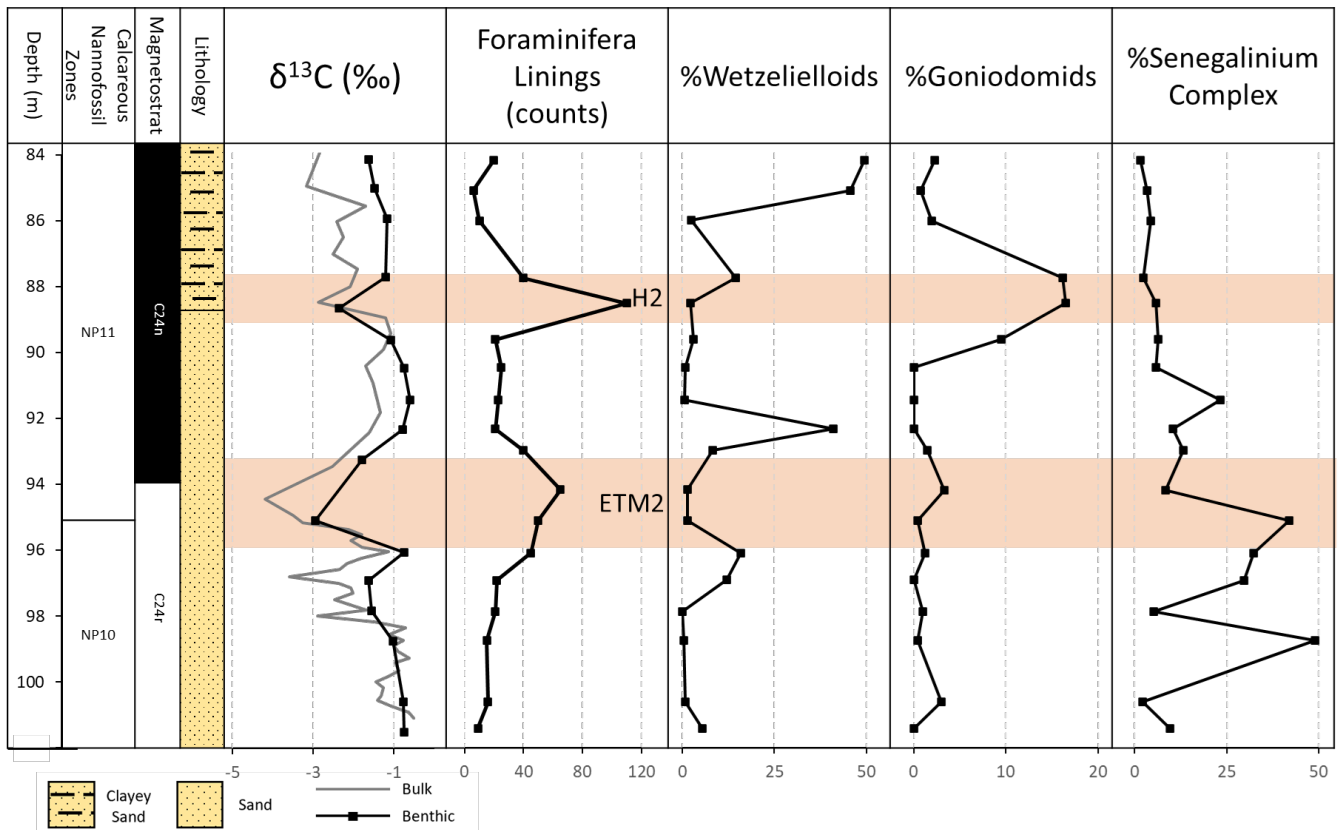
840 Figure 5: Knapps Narrows core site, from left to right: depth, nanofossil zones, magnetochrons, lithology, carbon isotopes, foraminifera lining counts, relative abundance of Wetzeliellids, relative abundance of Goniodomids, and relative abundance of the Senegalinium Complex. Foraminifera linings can be used to infer periods of rapid or low siliciclastic influx. Wetzeliellids are associated with periods of high productivity, Goniodomids are associated with high temperatures and strong salinity stratification, 845 from relatively fresh conditions at the base of the core to more saline conditions upsection. Rapid changes in abundance of Wetzeliellids suggests disconformities, periods of non-deposition, or condensed sections.
