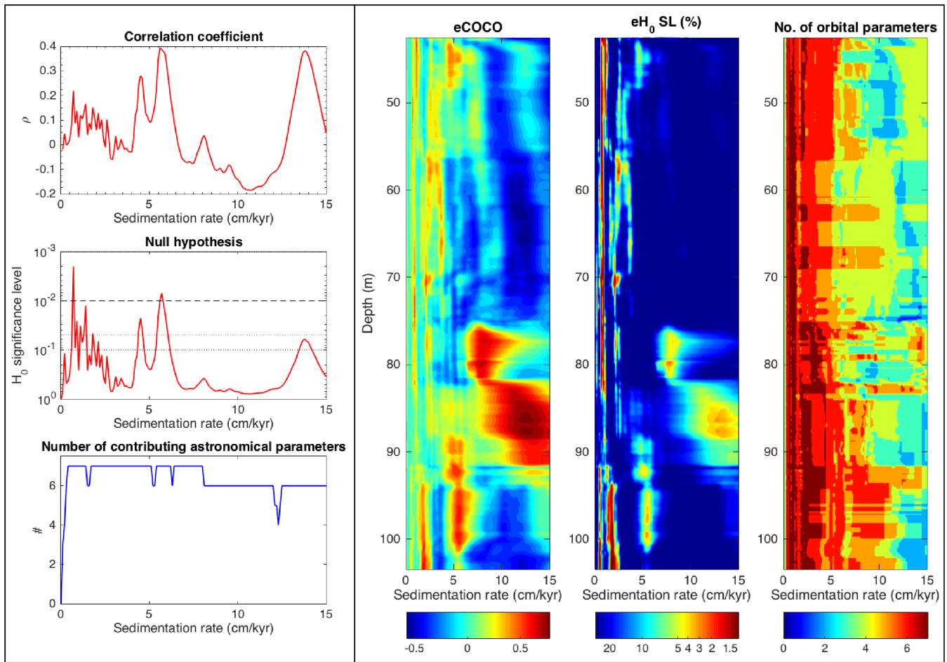
830 Figure 4: COCO (left panel) and eCOCO (right panel) analysis of the wireline gamma-ray log (42.5 m - 103.5 m). Studied interval lies between 84 m and 102 m. In the COCO plots, three clusters of high- \rho sedimentation rates accompanied with low H_0 significance level and relatively more (# 6-7) of contributing astronomical parameters are identified, i.e., at ~1 cm/kyr, ~5 cm/kyr, and ~13 cm/kyr. For the eCOCO analysis, the sliding window is 18 m using 0.2-m step. The target astronomical solution is La2004 at 53 Ma (with 7 astronomical cycles at 405, 125, 95, 39.2, 23.1, 21.9, and 18.8 kyr, respectively). All periodograms were analyzed with the AR(1) red 835 noise model removed. The number of Monte Carlo simulations is 2000. The tested sedimentation rates range from 0 to 15 cm/kyr with a step of 0.1 cm/kyr. Note that from depth of ~82 m – 90 m that covers the studied interval, a change of sedimentation rates exists from ~5 cm/kyr to ~13 cm/kyr. The evolutionary power spectrum (Supplementary figure 5) of this interval also indicates a distortion of cyclicity.
