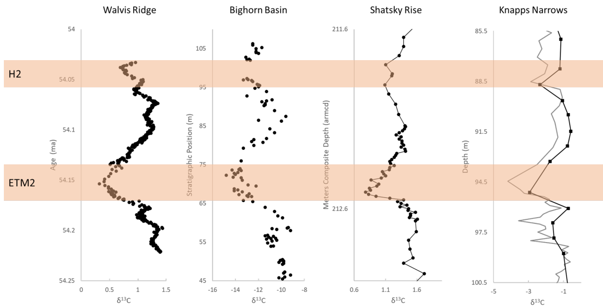
825 Figure 3: Carbonate \delta^{13}\text{C} records of ETM2 and H2 at Walvis Ridge (bulk), Bighorn Basin (pedogenic nodules), Shatsky Rise (benthic), and Knapps Narrows (this study). For Knapps Narrows, bulk carbonate values are in gray and benthic values are in black. Knapps Narrows at 94.5 m was nearly barren of foraminifera. Walvis Ridge data from Stap et al., (2010), age model from Lauretano et al., (2015), Bighorn Basin from Abels et al., (2015), and Shatsky Rise from Westerhold et al., (2018).
