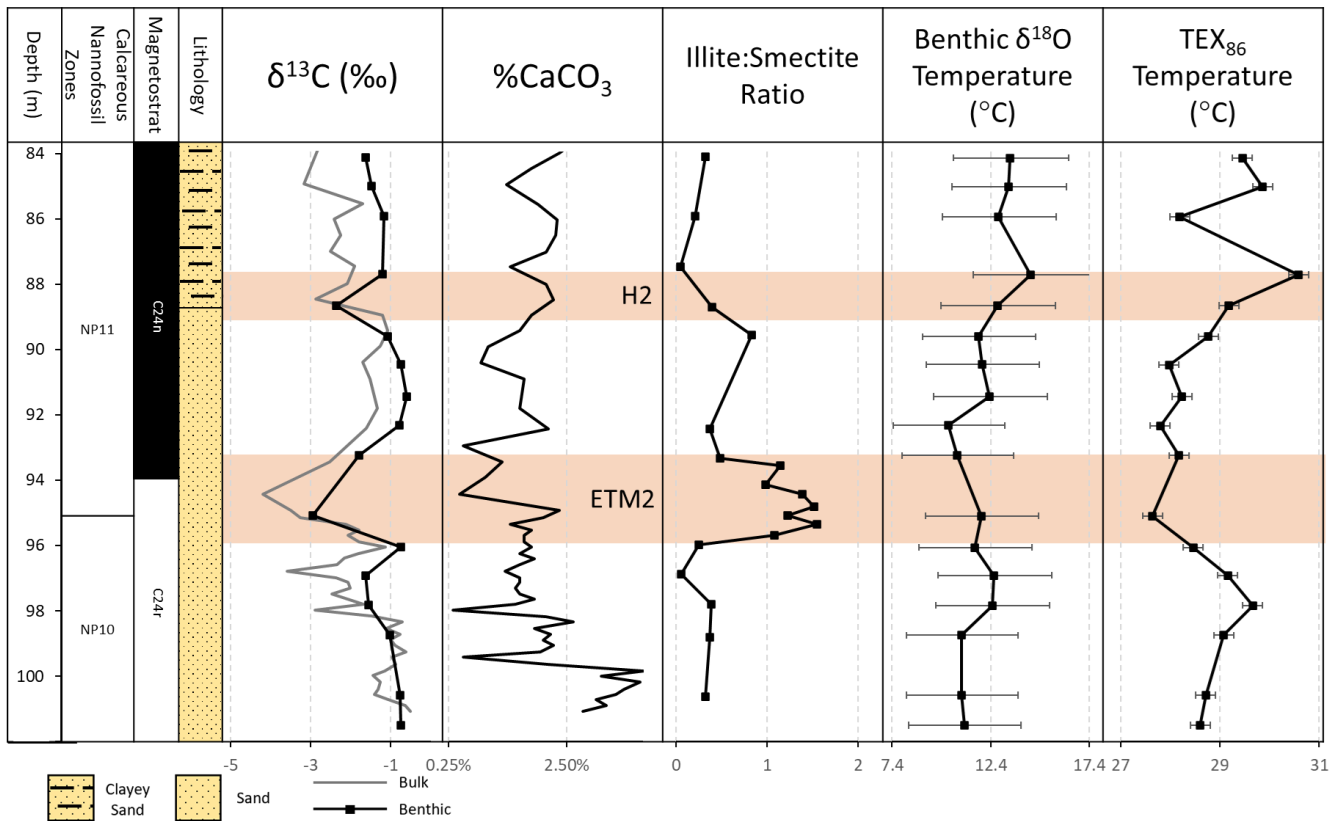
Figure 2: Knapps Narrows core site, from left to right: depth, nanofossil zones, magnetostrat, lithology, carbon isotopes, % carbonate, clay mineralogy, benthic \delta^{18}\text{O} temperatures, and TEX 86 sea surface temperatures over the ETM2 and H2 interval at Knapps Narrows. TEX 86 temperatures use linear calibration from O'Brien et al., (2017). Note logarithmic scale for % carbonate and low carbonate interval at ETM2, spike in illite-smectite ratio at ETM2, agreement between benthic and sea surface temperatures, as well as offsets in timing between carbon isotopes, clay mineralogy, and temperature proxies.
