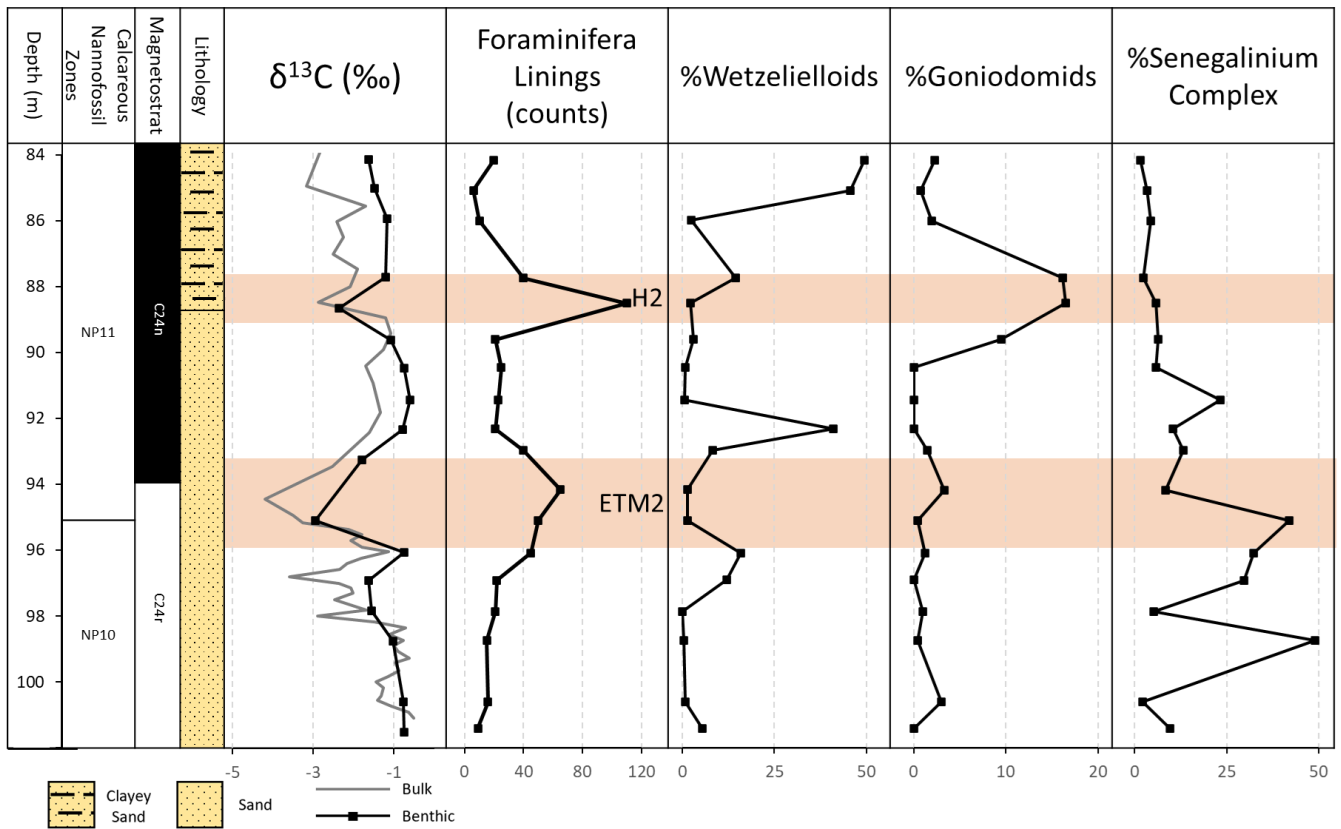
840 Figure 5: Knapps Narrows core site, from left to right: depth, nannofossil zones, magnetochrons, lithology, carbon isotopes, foraminifera lining counts, relative abundance of Wetziellids, relative abundance of Goniodomids, and relative abundance of the Senegalinium Complex. Foraminifera linings can be used to infer periods of rapid or low siliciclastic influx. Wetziellids are associated with periods of high productivity, Goniodomids are associated with high temperatures and strong salinity stratification, and the Senegalinium complex is associated with low salinity (Frieling and Sluijs, 2018). Of note is a long-term increase in salinity 845 Wetziellids suggests disconformities, periods of non-deposition, or condensed sections.
