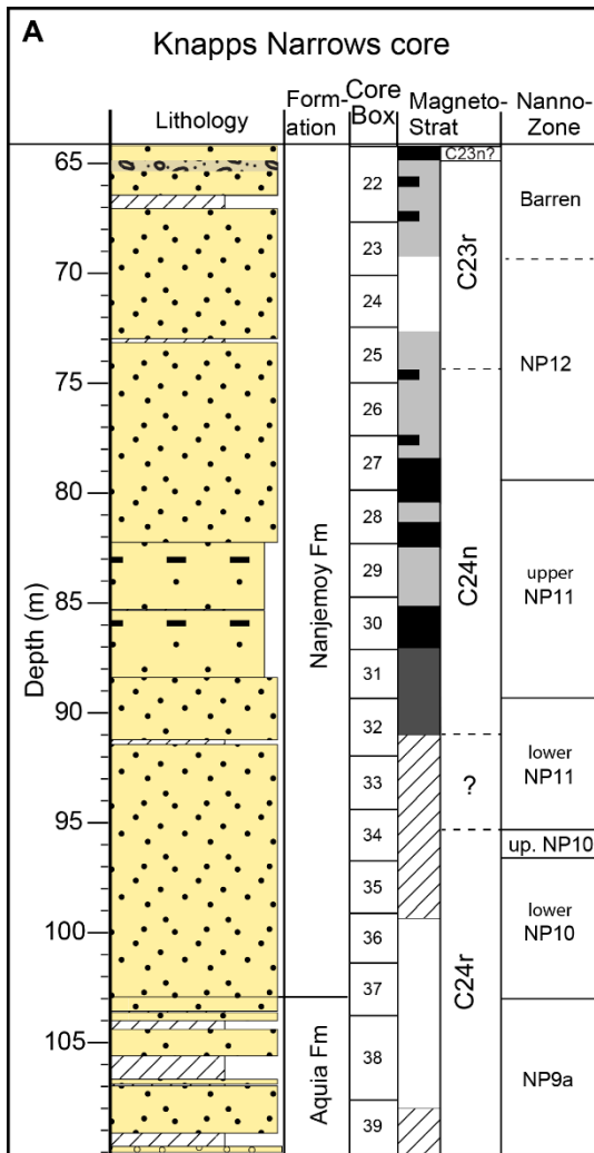
Appendix 2: A) The magnetostratigraphy and calcareous nannofossil zones (nanno-zone) of Knapps Narrows core. Note that the C24r/C24n reversal boundary was not well determined due to a sampling gap, but was well constrained to the interval, where the question mark was placed, based on nannofossils. B) The latest Paleocene to earliest Eocene time scale from GTS2020 (Gradstein et al., 2020) showing the geomagnetic polarity scale, the calcareous nannofossil zones and the composite carbon-13 isotope curve (major carbon-13 excursions and events are also marked). The excursion of ETM2 aligns with the C24r/C24n reversal.
