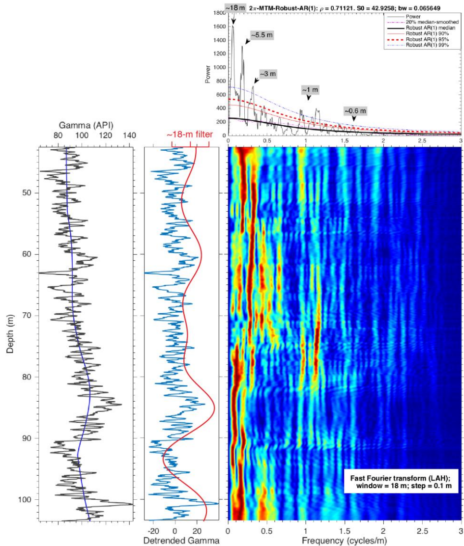
880 Appendix 5: Spectral analysis of the detrended gamma data of Knapps Narrows core (43.5 m – 103.5 m). From left to right shows, the raw gamma data (solid black line) with the ca. 21-m LOWESS trend (solid blue line), the detrended gamma data overlaid by the ~18-m filter (Gaussian bandwidth at 0.055 \pm 0.025 ), and spectral analysis of the detrended series. An interpolation of 0.03 m is applied before the spectral analysis. Evolutionary power spectrum (Fast Fourier transform; Kodama and Hinnov, 2015) uses an 18-m window. The 2\pi MTM power spectrum shows that the dominant cycles have wavelengths of ~18 m, ~5.5 m, 3 m, ~1 m and 0.6 m, respectively.
