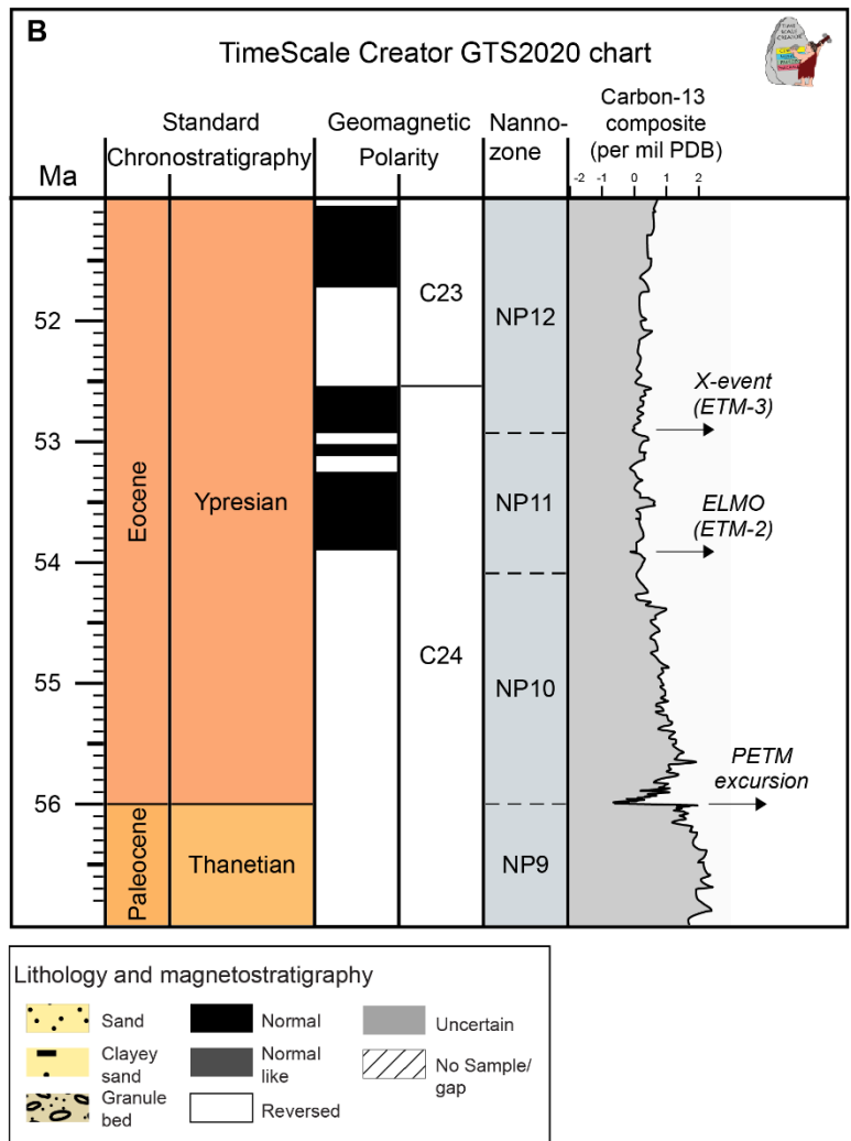
Appendix 2: A) The magnetostratigraphy and calcareous nannofossil zones (nanno-zone) of Knapps Narrows core. Note that the C24r/C24n reversal boundary was not well determined due to a sampling gap, but was well constrained to the interval, where the question mark was placed, based on nannofossils. B) The latest Paleocene to earliest Eocene time scale from GTS2020 (Gradstein et al., 2020) showing the geomagnetic polarity scale, the calcareous nannofossil zones and the composite carbon-13 isotope curve (major carbon-13 excursions and events are also marked). The excursion of ETM2 aligns with the C24r/C24n reversal.
