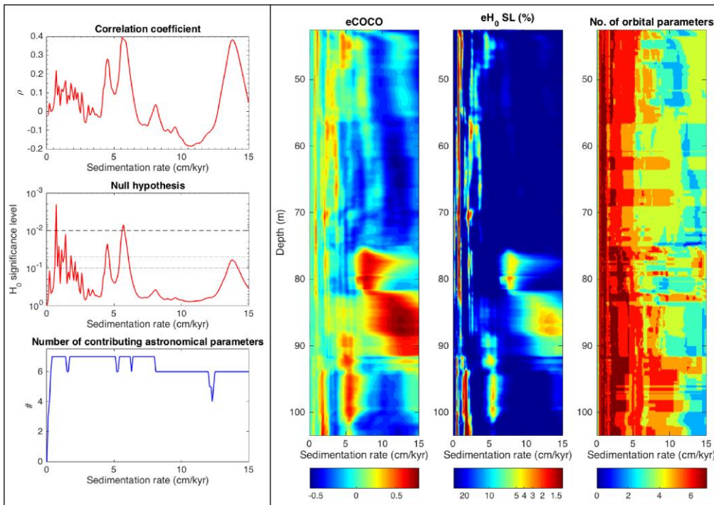
865 Figure 4: COCO (left panel) and eCOCO (right panel) analysis of the wireline gamma-ray log (42.5 m - 103.5 m). Studied interval lies between 84 m and 102 m. In the COCO plots, three clusters of high- \rho sedimentation rates accompanied with low H_0 significance level and relatively more (# 6-7) of contributing astronomical parameters are identified, i.e., at \sim 1 cm/kyr, \sim 5 cm/kyr, and \sim 13 cm/kyr. For the eCOCO analysis, the sliding window is 18 m using 0.2-m step. The target astronomical solution is La2004 at 53 Ma (with 7 astronomical cycles at 405, 125, 95, 39.2, 23.1, 21.9, and 18.8 kyr, respectively). All periodograms were analyzed with the AR(1) red noise model removed. The number of Monte Carlo simulations is 2000. The tested sedimentation rates range from 0 to 15 cm/kyr with a step of 0.1 cm/kyr. Note that from depth of \sim 82 m - 90 m that covers the studied interval, a change of sedimentation rates exists from \sim 5 cm/kyr to \sim 13 cm/kyr. The evolutionary power spectrum (Supplementary figure 5) of this interval also indicates a distortion of cyclicity. 870
