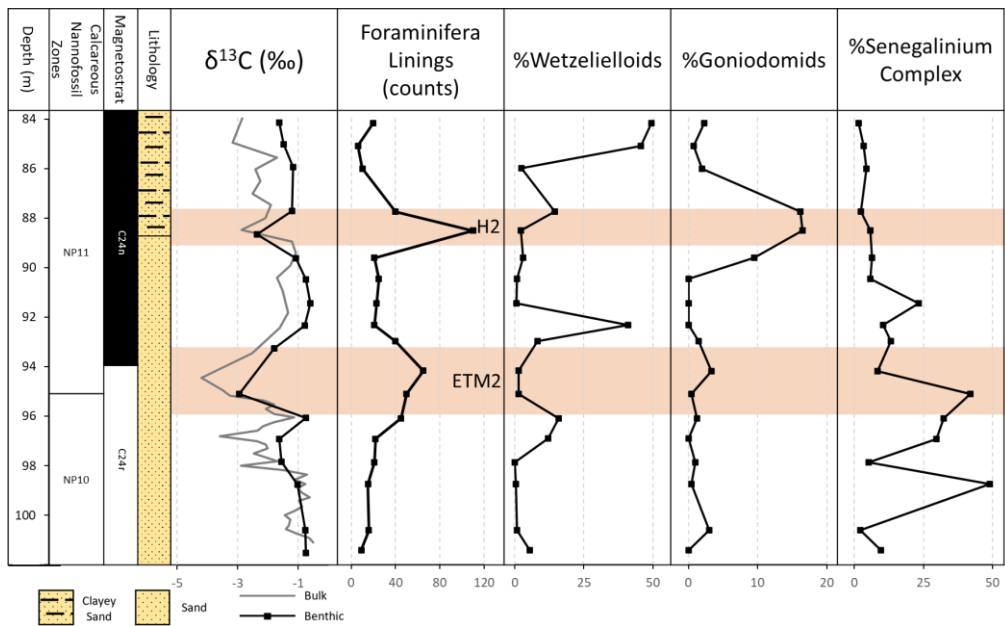
Figure 5: From Knapps Narrows core site, from left to right: depth, nannofossil zones, magnetochrons, lithology, carbon isotopes, foraminifera lining counts, relative abundance of Wetzeliioids, relative abundance of Goniodomids, and relative abundance of the Senegalinium Complex. Foraminifera linings can be used to infer periods of rapid or low siliciclastic influx. Wetzeliioids are associated with periods of high productivity, Goniodomids are associated with high temperatures and strong salinity stratification, and the Senegalinium complex is associated with low salinity (Frieling and Sluijs, 2018). Of note is a long-term increase in salinity from relatively fresh conditions at the base of the core to more saline conditions upsection. Rapid changes in abundance of Wetzeliioids suggests disconformities, periods of non-deposition, or condensed sections.
