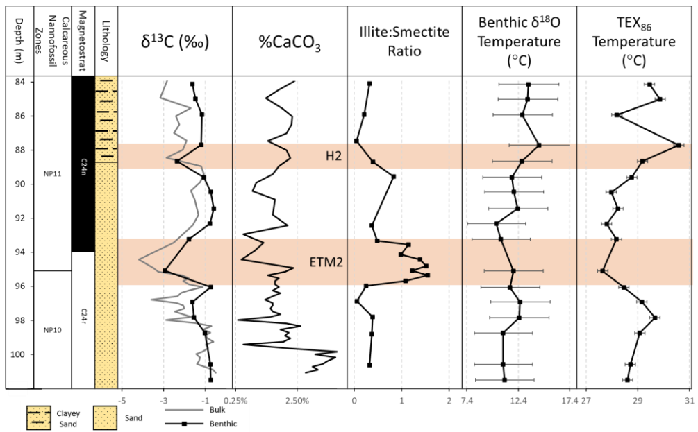
Figure 2: Knapps Narrows core site, from left to right: depth, nannofossil zones, magnetostrat, lithology, carbon isotopes, % carbonate, clay mineralogy, benthic \delta^{18}\text{O} temperatures, and TEX 86 sea surface temperatures over the ETM2 and H2 interval at Knapps Narrows. TEX 86 temperatures use linear calibration from O'Brien et al., (2017). Note logarithmic scale for % carbonate and low carbonate interval at ETM2, spike in illite-smectite ratio at ETM2, agreement between benthic and sea surface temperatures, as well as offsets in timing between carbon isotopes, clay mineralogy, and temperature proxies.
