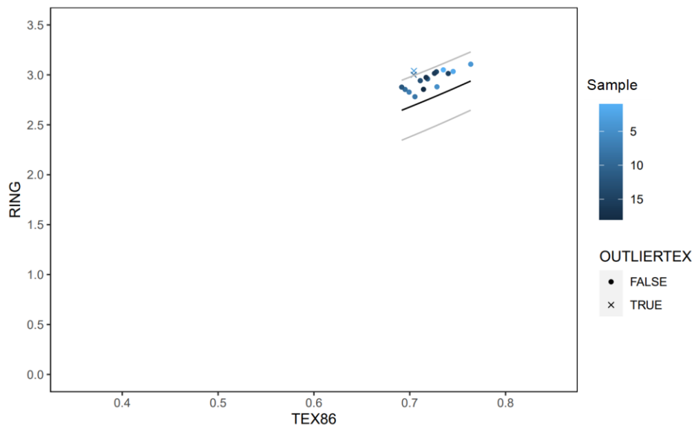
Appendix 3: Ring index (Zhang et al., 2016) plotted against \text{TEX}_{86} values for Knapps Narrows. Values generally fall within the acceptable range, indicating little non-thermal overprint. The temperature reconstructions obtained from the outliers were in line with independent measurements from \delta^{18}\text{O} . Moreover, the cut-off to identify anomalous values is rather conservative (Y.G. Zhang, written comm 2022). Therefore, we included these data points in the figures.
