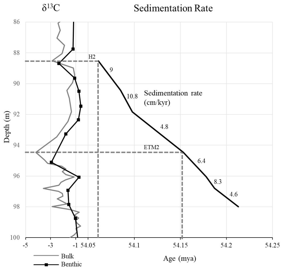
885 Figure 6: Sedimentation rates in the Knapps Narrows core based on correlations of \delta^{13}\text{C} inflection points to the age model of Lauretano et al., 2015 at Walvis Ridge Site 391. Sedimentation rates in cm/kyr. Note relative consistency compared to orders of magnitude changes that were documented during the PETM in Stassen et al. (2012b), with moderate increases beginning at 91.8 m, consistent with cyclostratigraphy.
