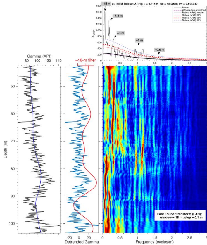
915 Appendix 5: Spectral analysis of the detrended gamma data of Knapps Narrows core (43.5 m – 103.5 m). From left to right shows, the raw gamma data (solid black line) with the ca. 21-m LOWESS trend (solid blue line), the detrended gamma data overlaid by the ~18-m filter (Gaussian bandwidth at 0.055 \pm 0.025 ), and spectral analysis of the detrended series. An interpolation of 0.03 m is applied before the spectral analysis. Evolutionary power spectrum (Fast Fourier transform; Kodama and Hinno, 2015) uses an 18-m window. The 2\pi MTM power spectrum shows that the dominant cycles have wavelengths of ~18 m, ~5.5 m, 3 m, ~1 m and 0.6 m, respectively. 920
