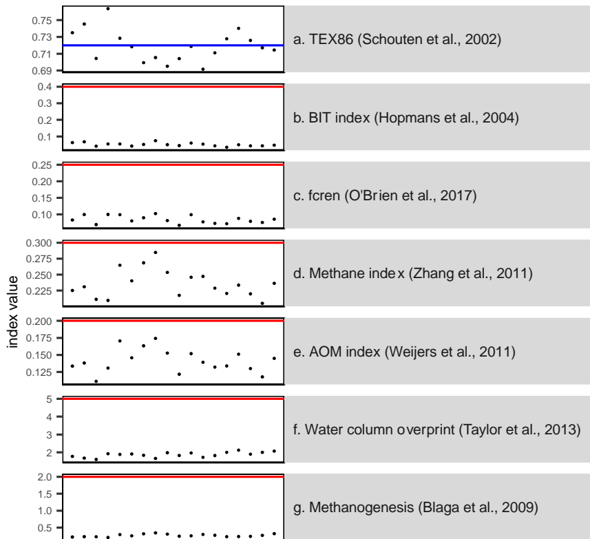
Appendix 4: Analysis of potential confounding factors for TEX86 paleothermometry for all samples. The red line indicates the cutoff value; red crosses indicate samples exceed the cutoff (a) TEX86, with the blue line indicating the maximum modern core-top value (~ 0.72). (b) Low BIT index values indicate insignificant supply of terrestrial GDGTs (c) fcren' shows no non-thermal contribution of crenarchaeol isomer. (d) Methane index values imply no contribution by methane metabolizing archaea (e) AOM ratio values show no contribution by anaerobic methane oxidizers (f) GDGT-2/3 values show no contributions of deep-dwelling archaea (g) low GDGT-0/Cren values show no contribution by methanogenic archaea.
