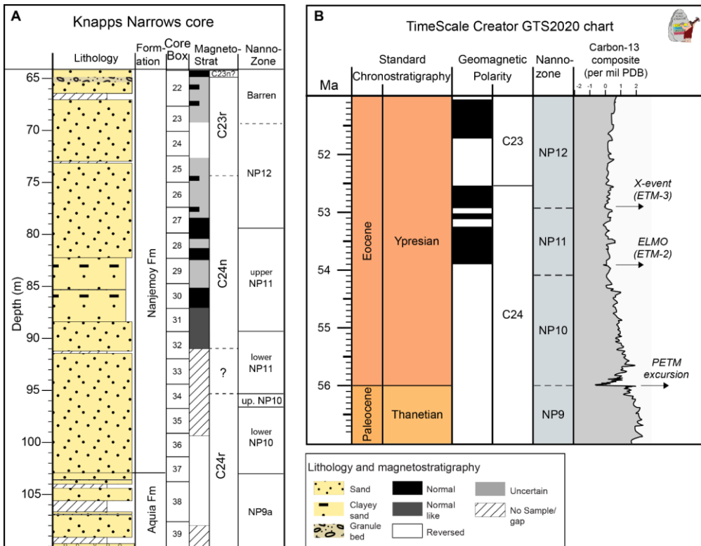
895 Appendix 2: A) The magnetostratigraphy and calcareous nannofossil zones (nanno-zone) of Knapps Narrows core. Note that the C24r/C24n reversal boundary was not well determined due to a sampling gap, but was well constrained to the interval, where the question mark was placed, based on nannofossils. B) The latest Paleocene to earliest Eocene time scale from GTS2020 (Gradstein et al., 2020) showing the geomagnetic polarity scale, the calcareous nannofossil zones and the composite carbon-13 isotope curve (major carbon-13 excursions and events are also marked). The excursion of ETM2 aligns with the C24r/C24n reversal.
