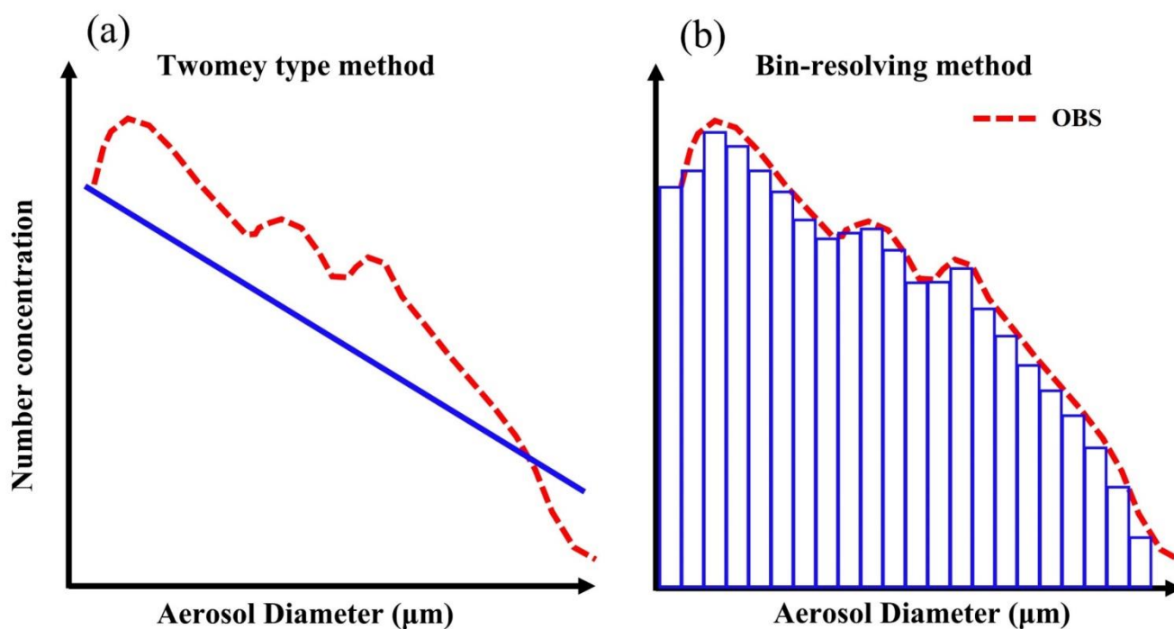
415 Figure 1: The schematic illustrates two methods for determining aerosol size distribution: (a) the Twomey method is used in WDM6, and (b) the bin-resolving method is used in WDM6-NCU. The blue line and bars present two different methods that model simulation describes the CCN size distribution, and the red dashed line shows as the observational CCN size distribution.
