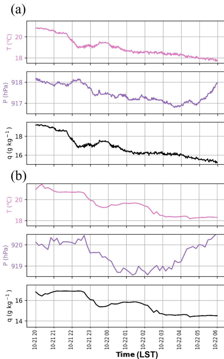
Figure 7: Time series (LST) of temperature, pressure, and water vapour mixing ratio based on (a) observation and (b) model simulation in the Dongyan mountain site before cloud seeding was conducted.
