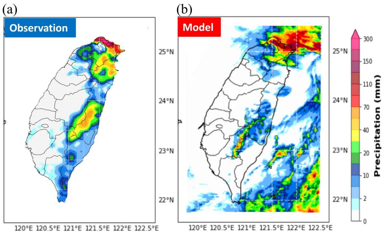
Figure 5: Cumulative rainfall based on (a) observation data and (b) model simulation from 21 October, 2020 12:00 UTC to 22 October, 2020 12:00 UTC.
