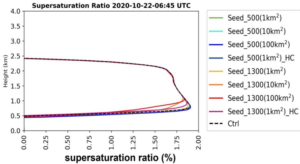
495 Figure 13: Vertical profile of averaged supersaturation ratio in the Shihmen region 15 min after cloud seeding.
