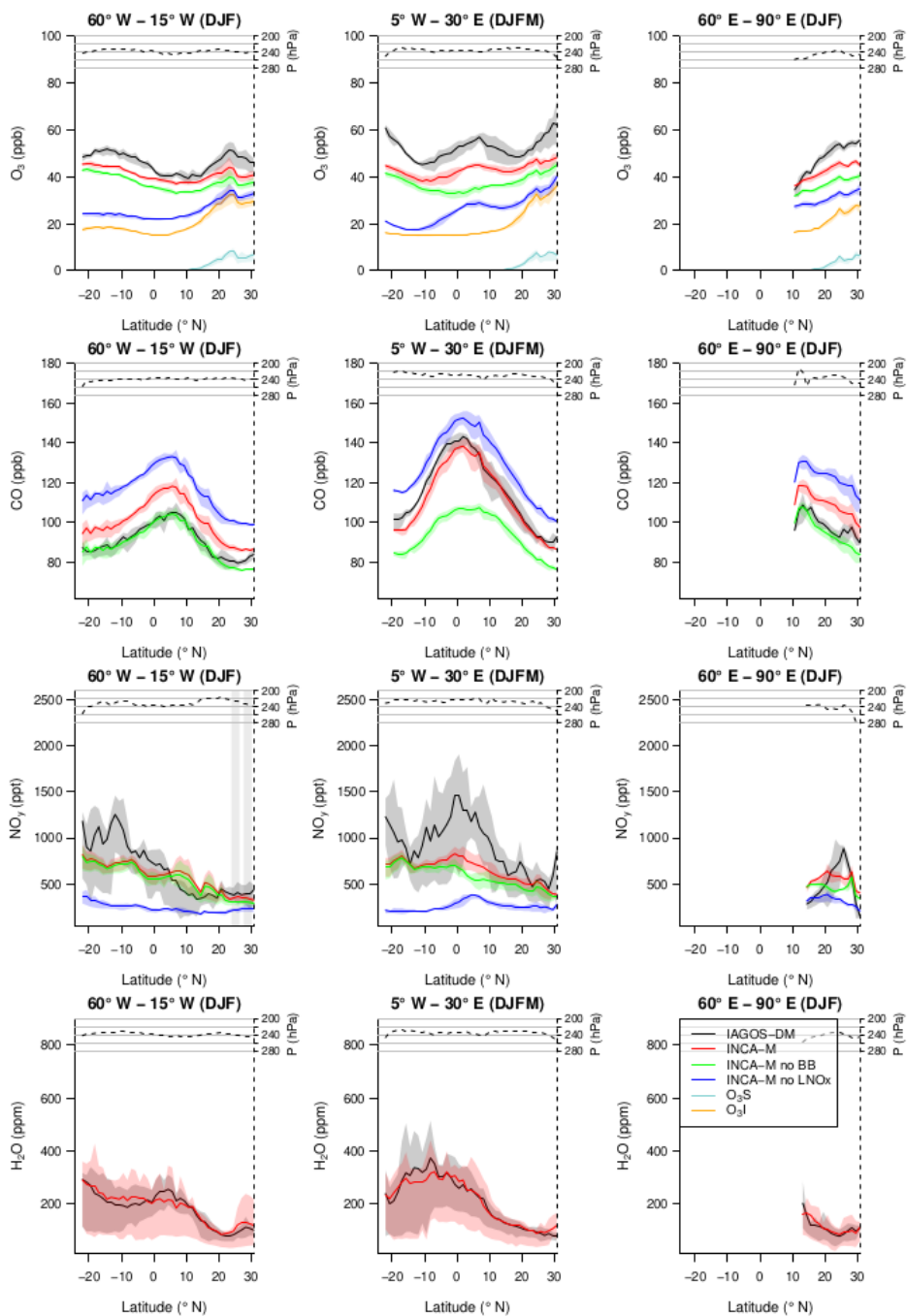
Figure 7. Zonal cross sections between 25^{\circ} S and 30^{\circ} N from December until February or March. Each row represents a measured variable, and each column represents a longitude interval from which the zonal means have been derived. As the season's definition, they are indicated in the title of each graphic. The uncertainties shown here correspond to the spatial variability, defined as the interval between the quartiles 1 and 3. The solid black line corresponds to IAGOS-DM, whereas the red, blue and green lines correspond respectively to the INCA-M reference simulation, and to the INCA-M simulations without emissions from lightning and from biomass burning. In the ozone panels, the orange and light-blue lines show the O_3I and O_3S stratospheric tracers. The dashed line at the top of each graphic shows the mean pressure derived from observations. The latter's values are reported on the right axis.
