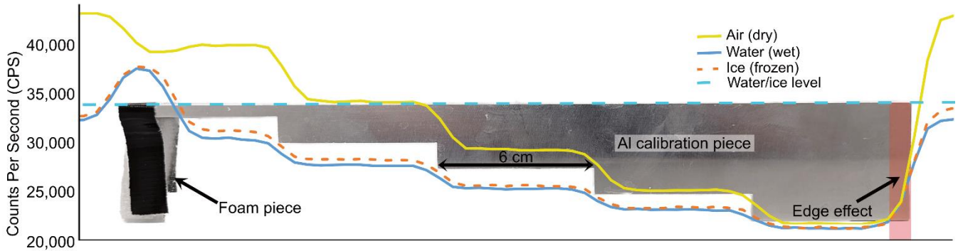
Figure 2: Comparison of the wet, frozen (ice) and dry calibration of gamma density.
