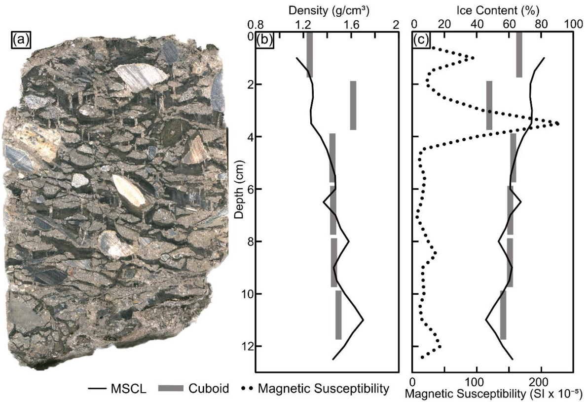
510 Figure 8: (a) MSCL image of diamicton core; (b) frozen bulk density comparison between gamma attenuation and cuboid data; (c) estimated volumetric ice content from gamma attenuation frozen bulk density, cuboid ice content and magnetic susceptibility data.
