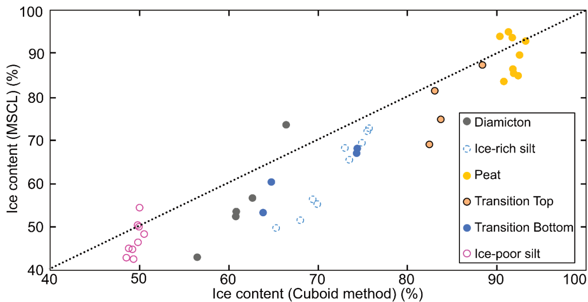
530 Figure 14: Comparison between discrete sample based volumetric ice content results from the cuboid and estimates from the MSCL. The black dotted line represents the regression line between the destructive cuboid method and the non-destructive MSCL method.
