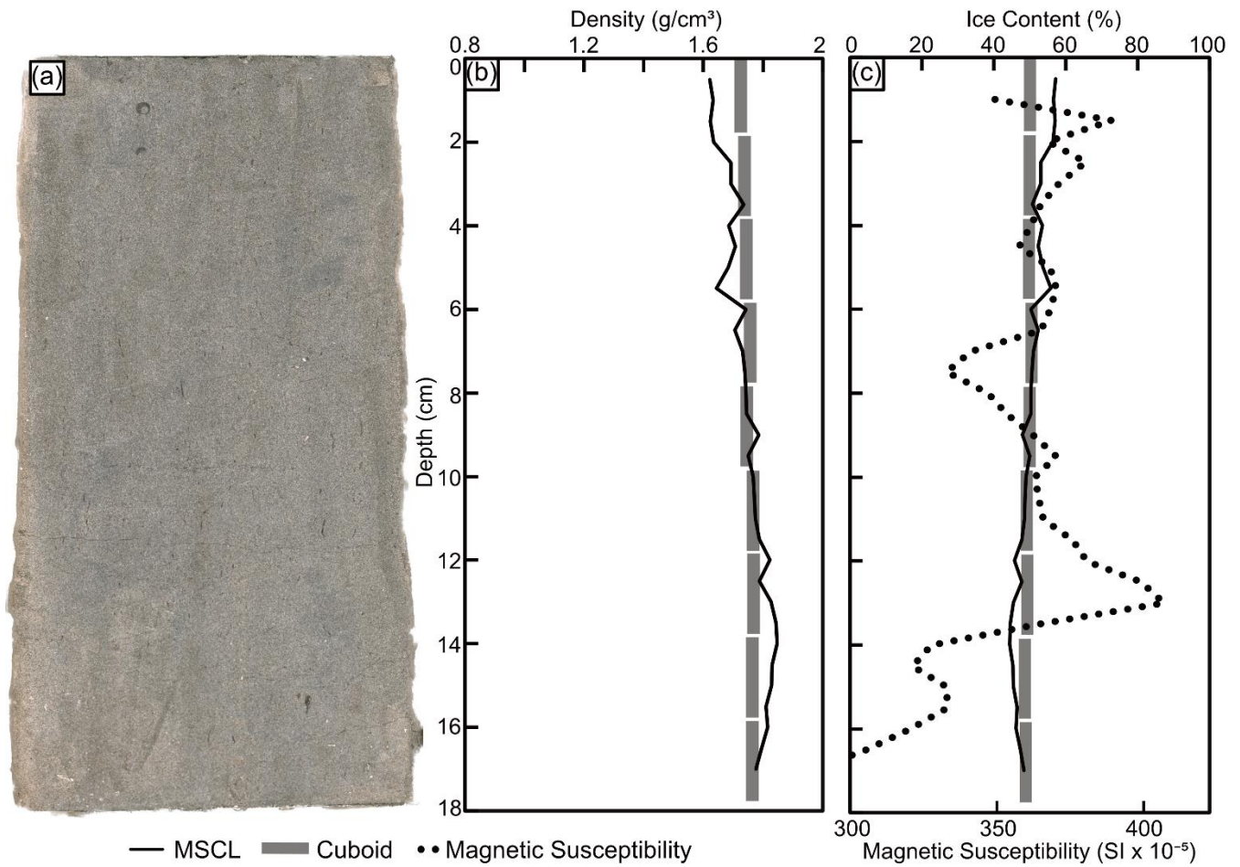
Figure 9: (a) MSCL image of ice-poor silt core; (b) frozen bulk density comparison between gamma attenuation and cuboid data; (c) estimated volumetric ice content from gamma attenuation frozen bulk density, cuboid ice content and magnetic susceptibility data.
