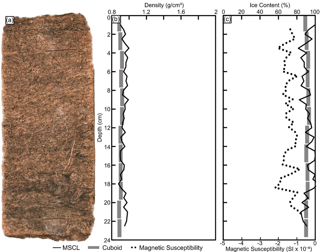
Figure 10: (a) MSCL image of peat core; (b) frozen bulk density comparison between gamma attenuation and cuboid data; (c) estimated volumetric ice content from gamma attenuation frozen bulk density, cuboid ice content and magnetic susceptibility data.
