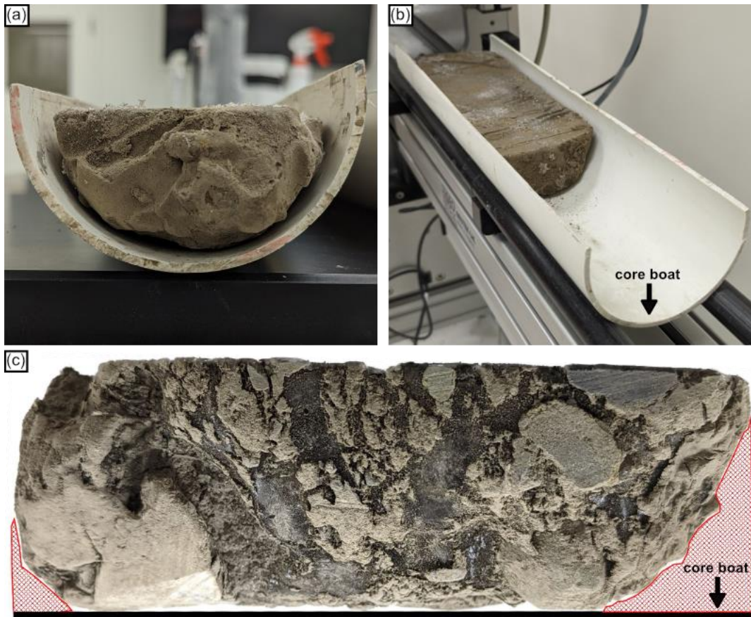
Figure 15: The MSCL core boat and core positioning examples; (a) down core view of a core in the core boat with minimal air gaps; (b) photo of core in the core boat on the MSCL track; (c) diamicton core (BS19-3-6) side profile to highlight the thickness variation not visible to the MSCL laser.
