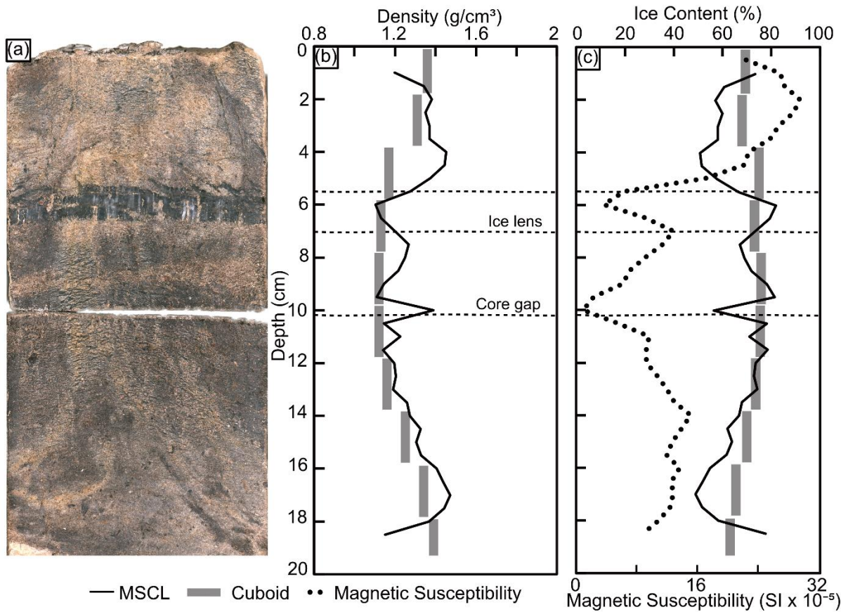
505 Figure 6: (a) MSCL image of ice-rich silt core; (b) frozen bulk density comparison between gamma attenuation and cuboid data; (c) estimated volumetric ice content from frozen bulk density and cuboid, and magnetic susceptibility data.
