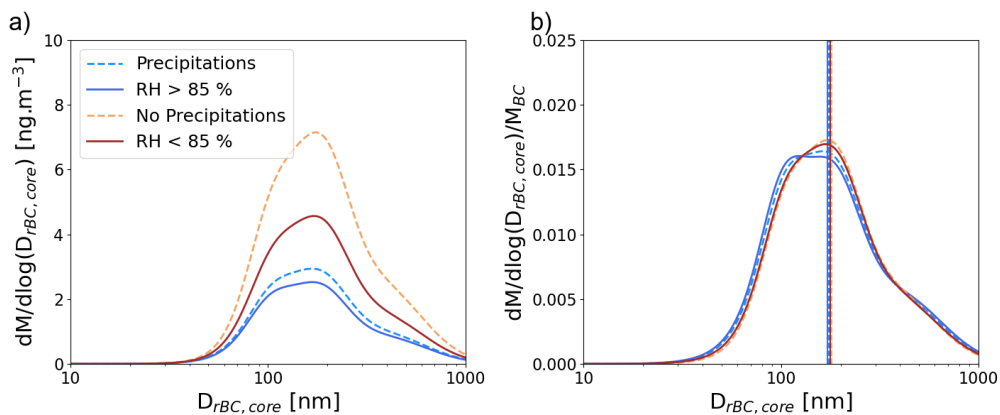
Figure 9. a) Mass size distributions and b) normalized mass size distributions of rBC core measured by the SP2 as a function of the presence or not of precipitation along the path of airmasses arriving at PDM, and whether the relative humidity was over 85 % or not. The normalization was done with the total rBC measured mass. Vertical lines show the geometric mean rBC core diameter colored by the criteria described in the legend.
