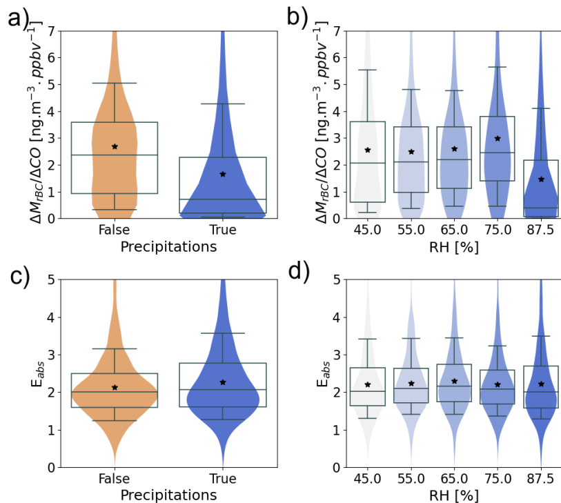
Figure 8. \Delta_{rBC/\Delta CO} emission ratio and E_{\text{abs}} vs. a) and c) precipitation along the air mass back trajectory calculated with HYSPLIT model and b) and d) Relative Humidity measured at PDM. Violin plots represent the probability density function of each parameter. Statistics of the boxplots are the same as Fig. 7. PBL conditions were filtered before analysis.
