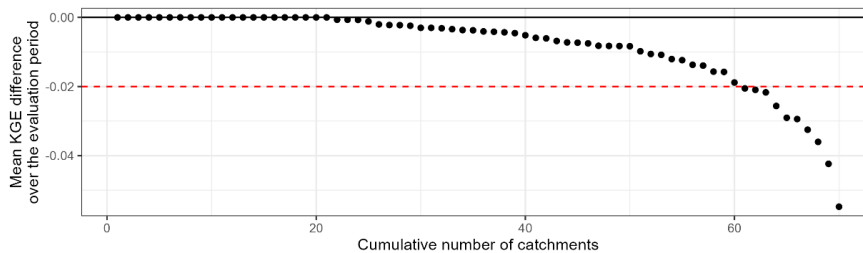
620 Figure 1919: Ranked performance difference curve obtained for the evaluation periods on each catchment by the best downstream model with an a priori choice on upstream simulation or not. The black line indicates the equivalence between both modelling frameworks. A negative value indicates a decline in performance due to the a priori choice of upstream simulations injected.
