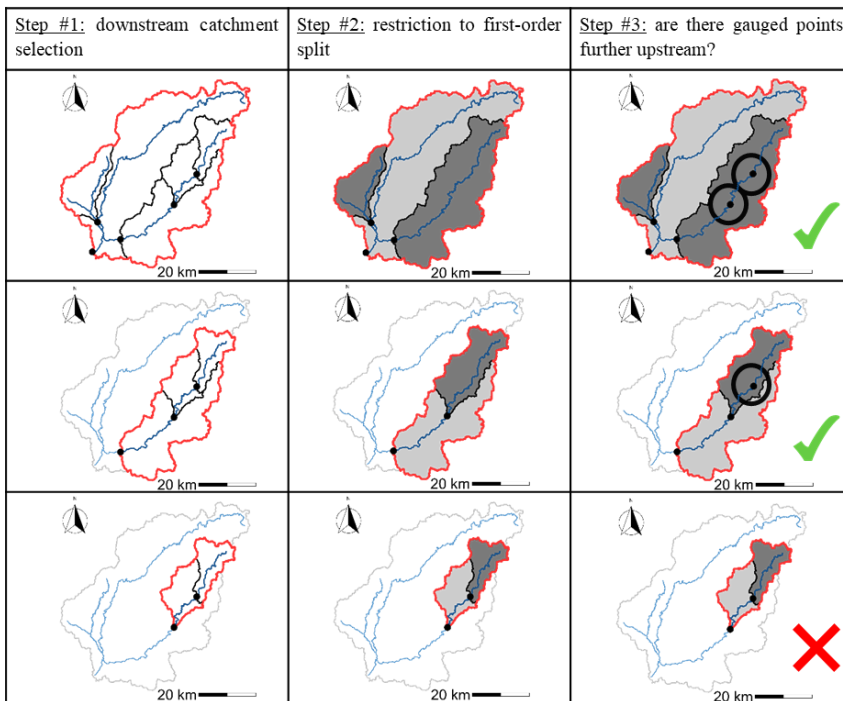
190 Figure 22: Illustration of the Matryoshka dolls approach to the Vézère River at Larche. The steps of the method are in column, the discretization levels in row. From this initial catchment (top left), three semi-distributed configurations were obtained (number of rows). For each semi-distributed configuration, the boundary of the catchment considered is in red, the first-order upstream catchments are filled in dark grey while the downstream catchment is in light grey.
