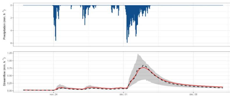
Figure 1049: Hydrograph of November–December 2003 of the Dore River at Saint-Gervais-sous-Meymont (K287191001). The grey shading shows the interval between the 10% and 90% quantiles generated by the 78 modelling options. The red line highlights the best MMM combination. The dashed black line refers to the observed streamflow.
