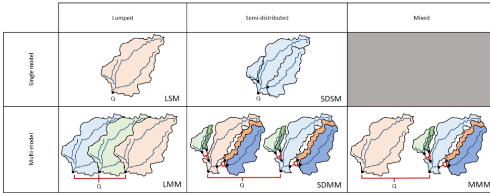
Figure 33: Summary of the different approaches tested. Q is the target streamflow at the main catchment outlet; black dots show gauging stations used. The different colours represent different model structures. The variations of the same colour indicate different parameterizations. Red links represent the combination of streamflow.
