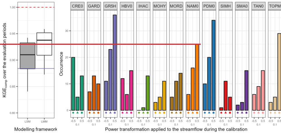
Figure 88: Distribution of the performance ( KGE_{comp} score) of the best lumped multi-models (LMM) over the 121 catchments (left part) and model occurrence within this selection (right part). The boxplots represent the 10%, 25%, 50%, 75% and 90% quantiles. The dashed red line represents the optimal KGE value. The benchmark corresponds to a one-size-fits-all approach with the GR5H structure calibrated with a generalist objective function Q^{0.1} over the whole catchments set. The dashed red line represents the optimal KGE value while the purple line refers to the median performance of the one-size-fits-all model (i.e. GR5H calibrated with a generalist objective function Q^{0.1} over the whole catchments set). The benchmark is the choice of the best lumped single model on each catchment and is represented by a grey box.
