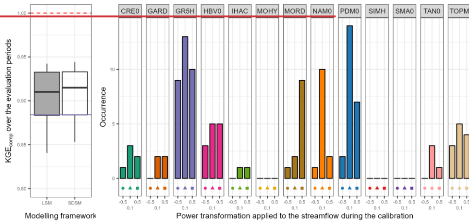
Figure 77: Distribution of the performance ( KGE_{comp} score) of the best semi-distributed single models (SDSM) over the 121 catchments (left part) and model occurrence within this selection (right part). The boxplots represent the 10%, 25%, 50%, 75% and 90% quantiles. The dashed red line represents the optimal KGE value. The benchmark corresponds to a one-size-fits-all approach with the GR5H structure calibrated with a generalist objective function Q^{0.1} over the whole catchments set. The dashed red line represents the optimal KGE value while the purple line refers to the median performance of the one-size-fits-all model (i.e. GR5H calibrated with a generalist objective function Q^{0.1} over the whole catchments set). The benchmark is the choice of the best lumped single model on each catchment and is represented by a grey box.
