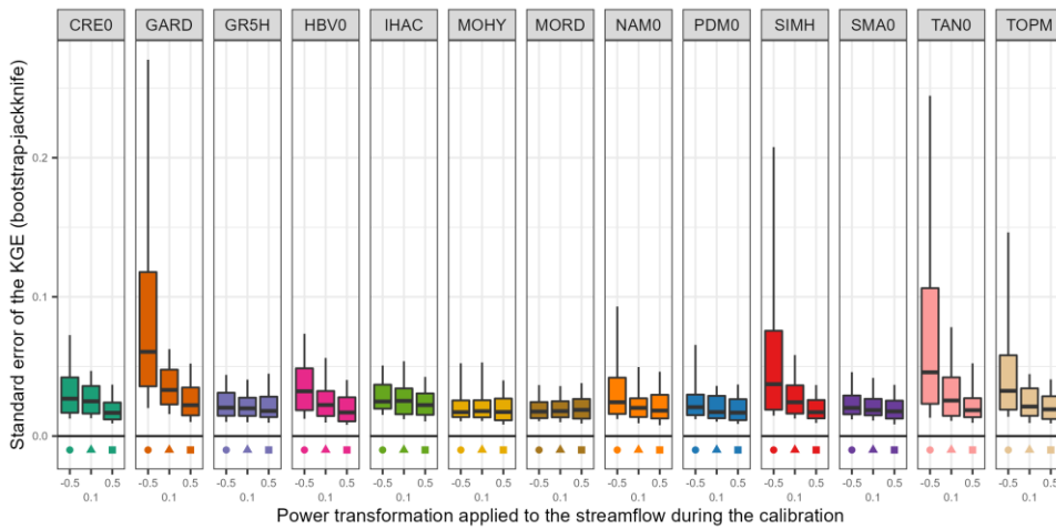
700 Figure C1: Distribution of standard error of the KGE obtained with bootstrap-jackknife methodology over the 121 catchments. The boxplots represent the 10%, 25%, 50%, 75% and 90% quantiles.
