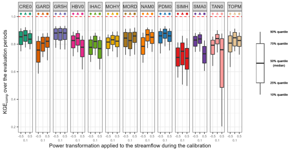
Figure 44: Distribution of the performance ( KGE_{comp} score) of the 39 lumped single models over the 121 catchments and over the evaluation periods. The boxplots represent the 10%, 25%, 50%, 75% and 90% quantiles. The dashed red line represents the optimal KGE value. Each colour represents a structure, and each geometric pattern represents the power transformation applied to the streamflow during the calibration.
