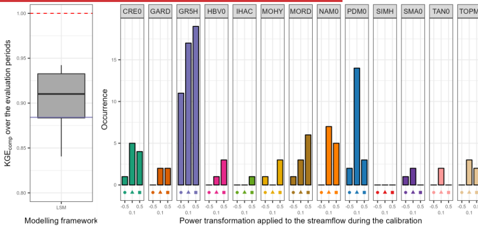
Figure 55: Distribution of the performance ( KGE_{comp} score) of the best lumped single models (i.e. the benchmark LSM) over the 121 catchments (left part) and model occurrence within this selection (right part). The boxplots represent the 10%, 25%, 50%, 75% and 90% quantiles. The dashed red line represents the optimal KGE value, while the purple line refers to the median performance of
