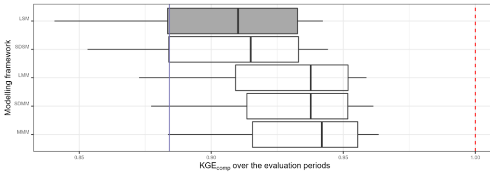
475 Figure 1242: Distribution of the performance ( KGE_{comp} score) of the best (multi-)models over the 121 catchments according to their modelling framework (LSM: lumped single model; SDSM: semi-distributed single model; LMM: lumped multi-model; SDMM: semi-distributed multi-model; MMM: mixed multi-model). The dashed red line represents the optimal KGE value while the purple line refers to the median performance of the one-size-fits-all model (i.e. GR5H calibrated with a generalist objective function Q^{+0.1} over the whole catchments set). The benchmark corresponds to a one-size-fits-all approach with the GR5H structure calibrated with a generalist objective function Q^{+0.1} over the whole catchments set. The benchmark is the choice of the best lumped single model on 480 each catchment and is represented by a grey box.
