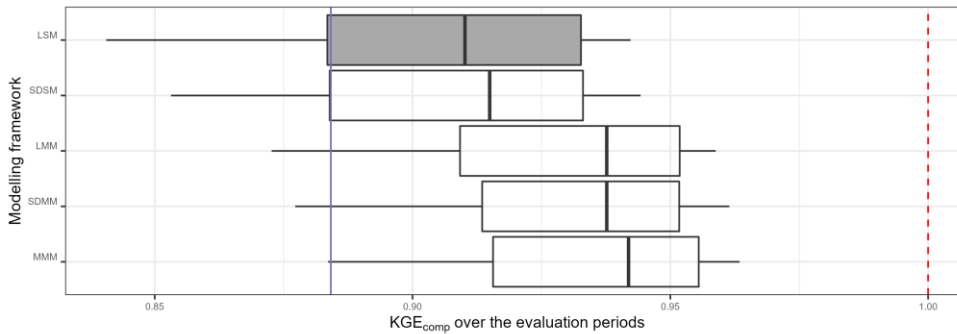
Figure 12: Distribution of the performance ( KGE_{comp} score) of the best (multi-)models (average of the three evaluation criteria) over the 121 catchments according to their modelling framework (LSM: lumped single model; SDSM: semi-distributed single model; LMM: lumped multi-model; SDMM: semi-distributed multi-model; MMM: mixed multi-model). The dashed red line represents the optimal KGE value while the purple line refers to the median performance of the one-size-fits-all model (i.e. GR5H calibrated with a generalist objective function Q^{+0.1} over the whole catchments set). The benchmark is the choice of the best lumped single model on each catchment and is represented by a grey box.
