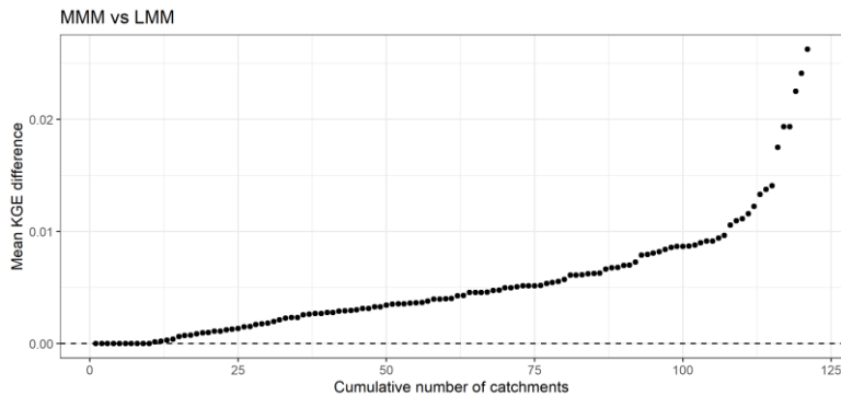
535 Figure 15: Ranked performance difference curve obtained for the evaluation periods between the best lumped and mixed multi-model on each catchment. The black line indicates the equivalence between the two modelling frameworks. The higher the value, the greater the benefit of a variable spatial framework.
