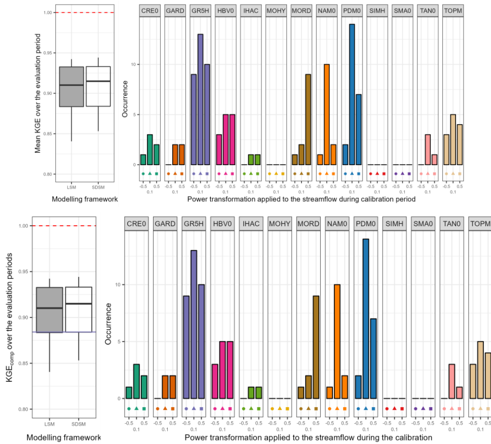
Figure 7: Distribution of the performance (average of the three evaluation criteria) KGE_{comp} score) of the best semi-distributed single models over the 121 catchments (left part) and model occurrence within this selection (right part). The boxplots represent the 10%, 25%, 50%, 75% and 90% quantiles. The dashed red line represents the optimal KGE value while the purple line refers to the median performance of the one-size-fits-all model (i.e. GR5H calibrated with a generalist objective function Q^{+0.1} over the whole catchments set). The benchmark is the choice of the best lumped single model on each catchment and is represented by a grey box.
