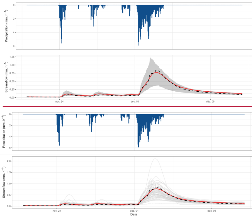
Figure 10: Hydrograph of November–December 2003 of the Dore River at Saint-Gervais-sous-Meymont (K287191001). The grey lines shading shows the interval between the 10% and 90% quantiles generated by the 78 modelling options simulation obtained in an LSM and a SDSM framework. The red line highlights the best MMM combination. The dashed black line refers to the observed streamflow.
