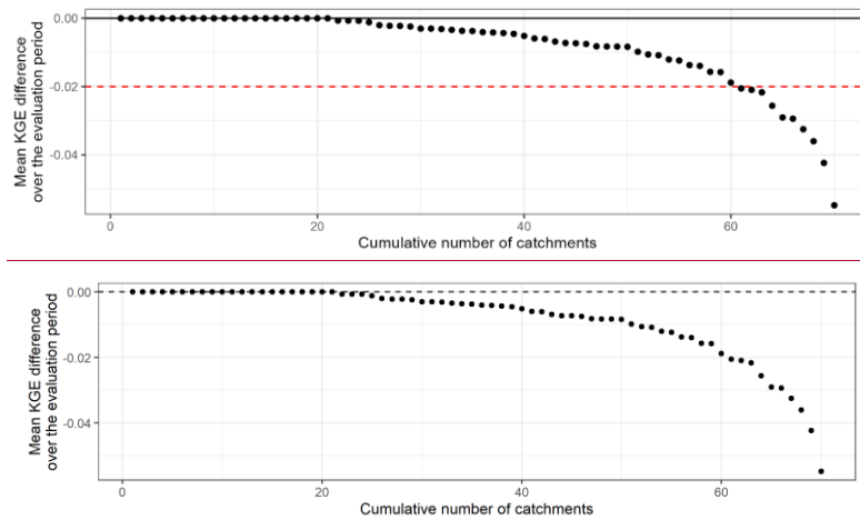
Figure 19: Ranked performance difference curve obtained for the evaluation periods on each catchment by the best downstream model with an a priori choice on upstream simulation or not. The black line indicates the equivalence between both modelling frameworks. A negative value indicates a decline in performance due to the a priori choice of upstream simulations injected.
