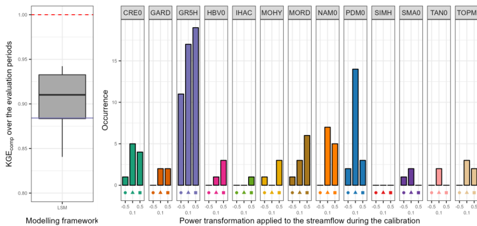
Figure 5: Distribution of the performance ( KGE_{comp} score) (average of the three evaluation criteria) of the best lumped single models (i.e. the benchmark) over the 121 catchments (left part) and model occurrence within this selection (right part). The boxplots represent the 10%, 25%, 50%, 75% and 90% quantiles. The dashed red line represents the optimal KGE value while the purple line refers to the median performance of the one-size-fits-all model (i.e. GR5H calibrated with a generalist objective function Q^{+0.1} over the whole catchments set).
