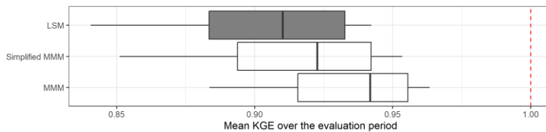
560 Figure 16: Distribution of the best simplified mixed multi-model, defined with a subset of four models, over the entire sample of catchments and over the evaluation periods. The boxplots represent the 10%, 25%, 50%, 75% and 90% quantiles. The benchmark is the choice of the best lumped single model on each catchment and is represented by a grey box. The dashed red line represents the optimal KGE value.
