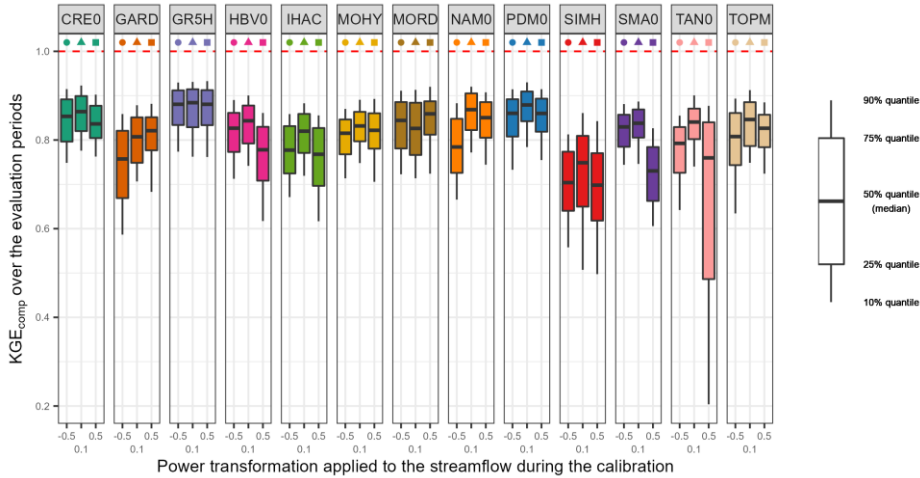
Figure 4: Distribution of the performance ( KGE_{comp} score) of the 39 lumped single models (average of the three evaluation criteria) over the 121 catchments and over the evaluation periods. The boxplots represent the 10%, 25%, 50%, 75% and 90% quantiles. The dashed red line represents the optimal KGE value. Each colour represents a structure and each geometric pattern represents the power transformation applied to the streamflow during the calibration period.
