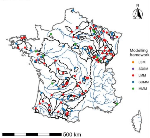
490 Figure 13: Maps of the best modelling framework on each catchment (top) and the simplest modelling framework among the best frameworks (bottom). The epsilon value corresponds to the performance deviation allowed from the best performance. If the drop between the evaluation performances is lower than or equal to epsilon, then the simplest modelling framework is selected.
