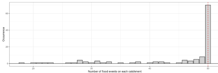
Figure A2: Distribution of the number of flood events on each catchment over the whole catchment set . The red line shows the maximum number allowed.
