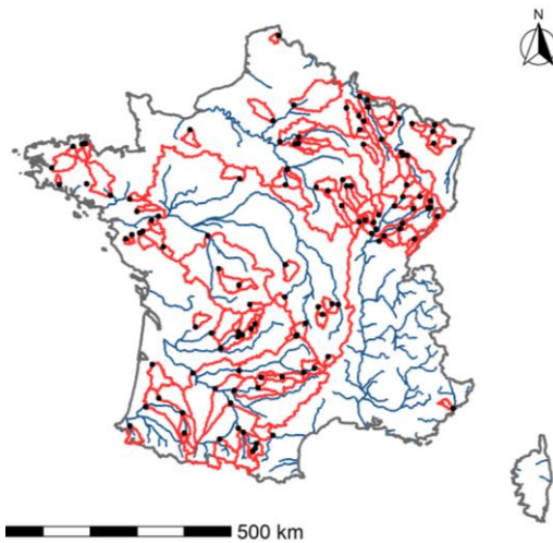
165 Figure 1: Boundaries (in red) and outlets (black dots) of the 121 catchments selected for this study.
