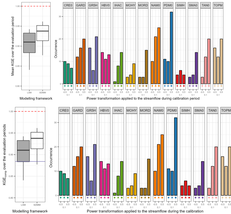
440 Figure 9: Distribution of the performance (KGE comp score) of the best semi-distributed multi-models (average of the three evaluation criteria) over the 121 catchments (left part) and model counts on the downstream catchment within this selection (right part). The boxplots represent the 10%, 25%, 50%, 75% and 90% quantiles. The dashed red line represents the optimal KGE value while the purple line refers to the median performance of the one-size-fits-all model (i.e. GR5H calibrated with a generalist objective function O^{0.1} over the whole catchments set). The benchmark is the choice of the best lumped single model on each catchment and is represented by a grey box.
