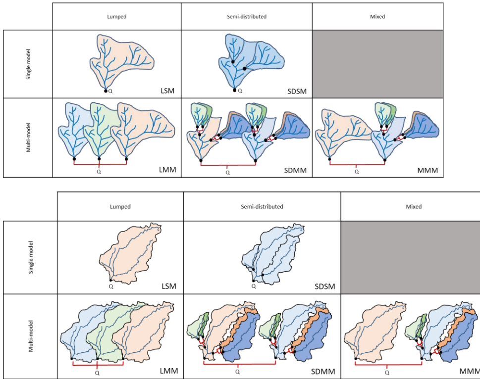
Figure 3: Summary of the different approaches tested. Q is the target streamflow at the main catchment outlet; black dots show gauging stations used. The different colours represent different model structures. The variations of the same colour indicate different parameterizations. Red links represent the combination of streamflow.
