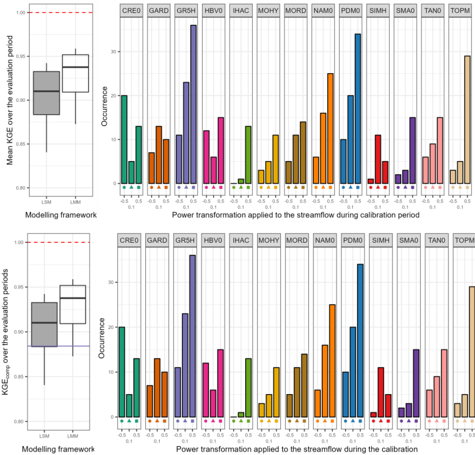
Figure 8: Distribution of the performance ( KGE_{comp} score) of the best lumped multi-models (average of the three evaluation criteria) over the 121 catchments (left part) and model occurrence within this selection (right part). The boxplots represent the 10%, 25%, 50%, 75% and 90% quantiles. The dashed red line represents the optimal KGE value while the purple line refers to the median performance of the one-size-fits-all model (i.e. GR5H calibrated with a generalist objective function Q^{0.1} over the whole catchments set). The benchmark is the choice of the best lumped single model on each catchment and is represented by a grey box.
