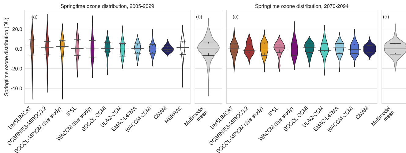
Figure 1. Probability density distributions calculated based on kernel density estimation of stratospheric partial ozone column (30-70 hPa) in spring (March-April) normalized by the mean ozone of the respective time period in the early (2005-2029, a, b) and late (2070-2094, c, d) 21st century in CCMI-1 models for RCP8.5. Whiskers show 20th and 80th percentile of the distributions. The multi-model mean shows the distributions over all models (excluding MERRA2) containing each ensemble member with equal weight. Similar Figs. for RCP2.6 and CCMI-2022 can be found in the supplementary material (Figs. A2 and A3).
