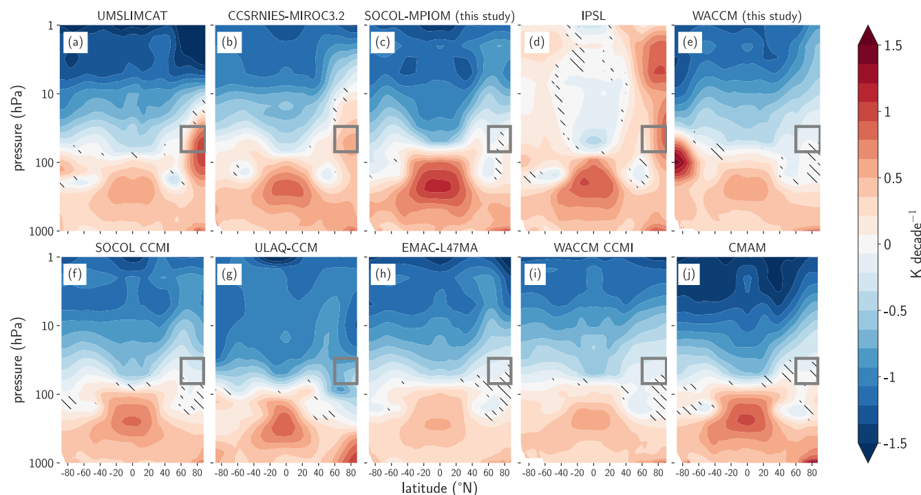
Figure 5. Temperature trend of the 20% coldest winters/springs (January – April mean) in a 25-year running window over the course of the 21st century in CCMI1 models for RCP8.5. Stippling marks regions which are not significant on a 5% level. The grey square marks the region of interest (60-90°N polar cap, 30-70 hPa).
