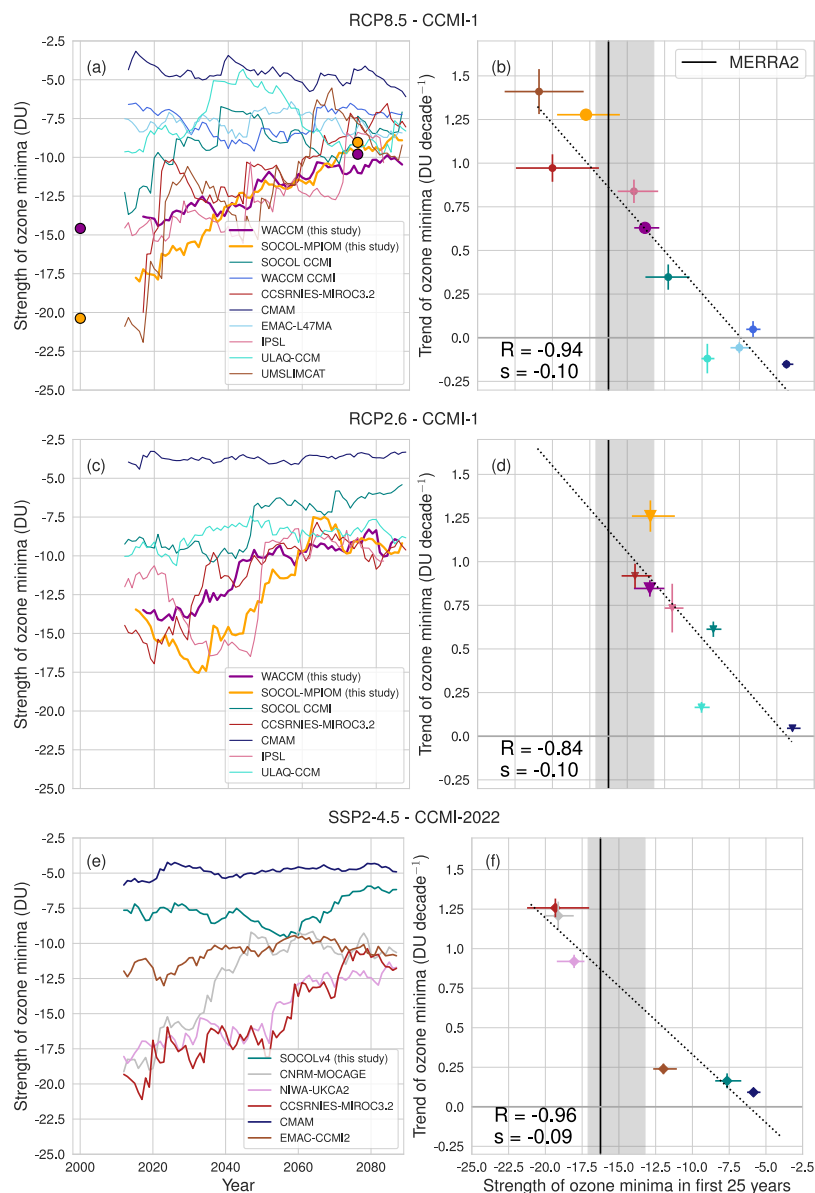
Figure 2. Development of the strength of Arctic ozone minima in CCMI-1 models under RCP8.5 (a) and RCP2.6 (c), as well as for CCMI-2022 models under SSP2-4.5 (e). Correlation of the trend in ozone minima strength and the strength of the ozone minima in the first 25 years defined by the mean ozone anomaly of the 20th percentile (5 out of 25 strongest ozone minima in running window, normalized by ozone climatology of running window). The mean strength of ozone minima in MERRA2 from 1980-2020 is given by the solid black line. The grey shading shows the uncertainty of the MERRA2 ozone minima strength, as explained in the methods section. Circles in (a) show the ozone minima strength of the WACCM and SOCOL-MPIOM timeslice simulations for the years 2000 and 2075, respectively.
