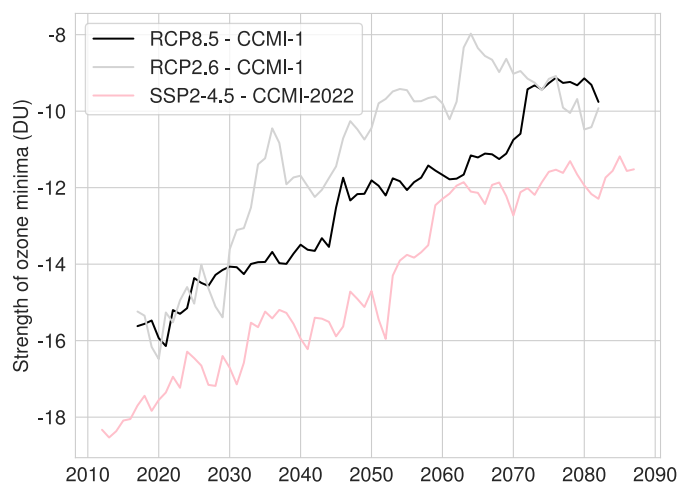
Figure A5. The weighted arithmetic mean for the development of the ozone minima strength in the three scenarios considered.
