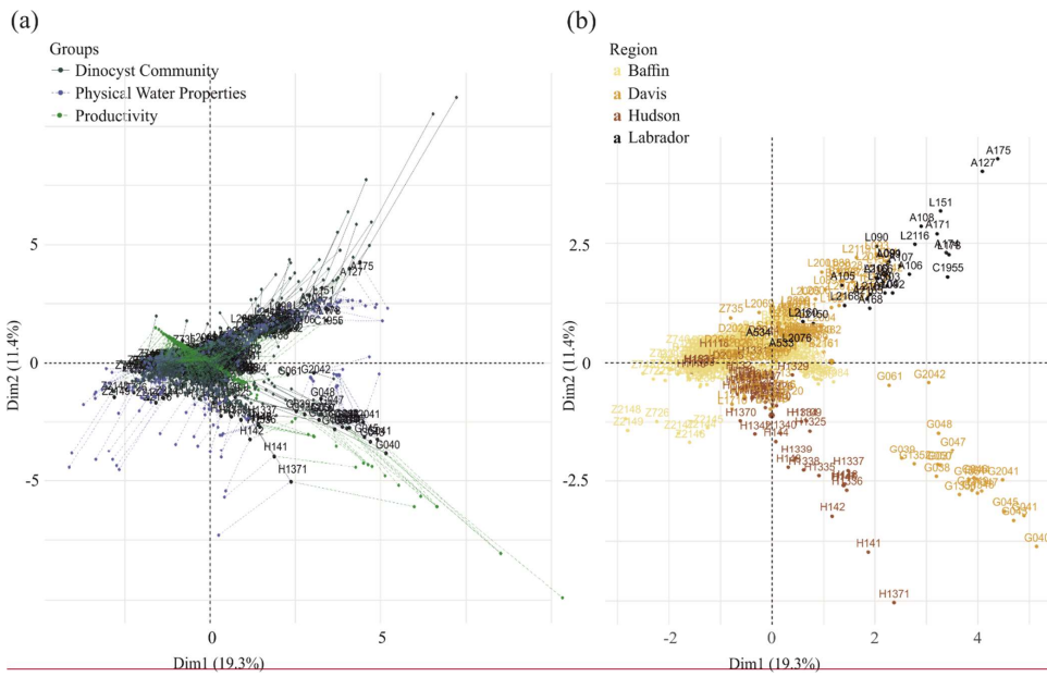
360 Figure 4: Sample sites within the first two dimensions of the MFA. (a) Sample site scores according to the pooled MFA with 421 data points (large black dots) and single PCAs depicting how much sample sites contribute to the variance in the data matrix in respect to the three groups. (b) Sample site scores relative to the first two dimensions of the global PCA. Sites with similar profiles are close to each other on the factor map.
