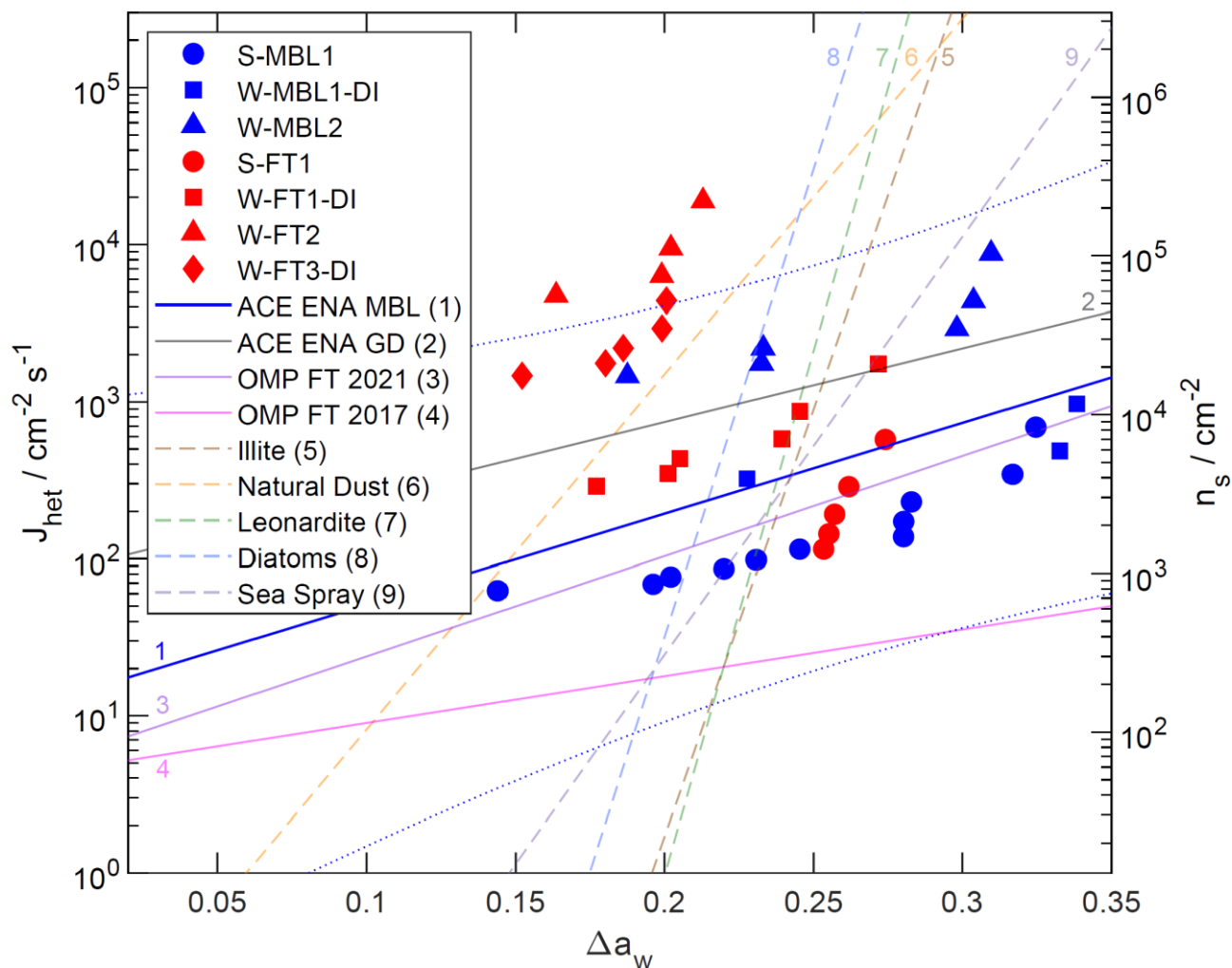
960 Figure 7: Immersion freezing (IMF) data of examined ACE-ENA particle samples (solid symbols) and of previous studies (colored 965 lines) as given in legend. Heterogeneous ice nucleation rate coefficients ( J_{\text{het}} ) and ice nucleation active sites (INAs) density ( n_s ) are presented as a function of the water activity criterion \Delta a_w . Corresponding error bars are given in Fig. S11. Blue solid line represents a linear regression to the newly derived MBL IMF data. Solid black, magenta, and purple lines represent J_{\text{het}} and n_s IMF derived from accompanying ACE-ENA ground site INP measurements (ACE-ENA GD), from the Observatory of Mountain Pico (OMP 970 FT 2017, 2021; (China et al., 2017; Lata et al., 2021)). Please note that only J_{\text{het}} was reported for OMP FT 2021 (Lata et al., 2021). Water activity-based IMF J_{\text{het}} and n_s for other INP types are given as dashed colored lines as indicated in legend.
