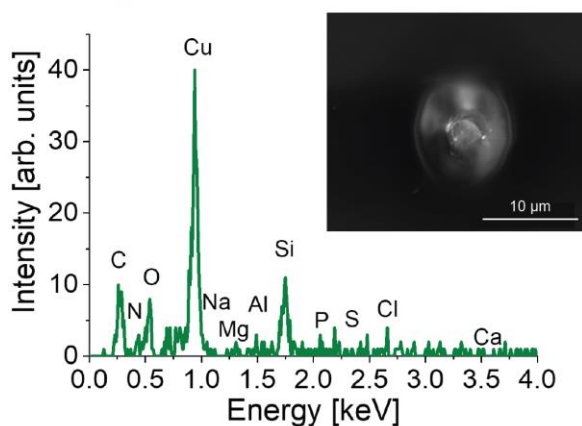
Figure S9: EDX spectra of identified INPs from particles samples collected during IOP1 under free troposphere (FT) conditions with corresponding SEM obtained particle image. Si and N signals stem from the substrate ( \text{Si}_3\text{N}_4 coated silicon wafer chips) and the chamber/holder (Al).
