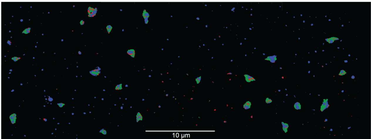
Figure S5: Representative particle mixing state analysis of particle samples collected in the marine boundary layer (MBL) where IN - inorganic, EC - elemental carbon, and OC - organic carbon. The scale bar holds for all panels.
