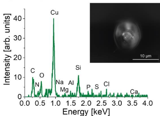
Figure S10: EDX spectra of identified INPs from particles samples collected during IOP2 under free troposphere (FT) conditions with corresponding SEM obtained particle image. Si and N signals stem from the substrate ( \text{Si}_3\text{N}_4 coated silicon wafer chips) and the chamber/holder (Al).
