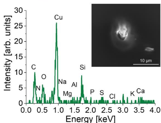
Figure S9: EDX spectra of identified INPs from particles samples collected during IOP1 under free troposphere (FT) conditions with corresponding SEM obtained particle image. Si and N signals stem from the substrate ( \text{Si}_3\text{N}_4 coated silicon wafer chips) and the chamber/holder (Al).
