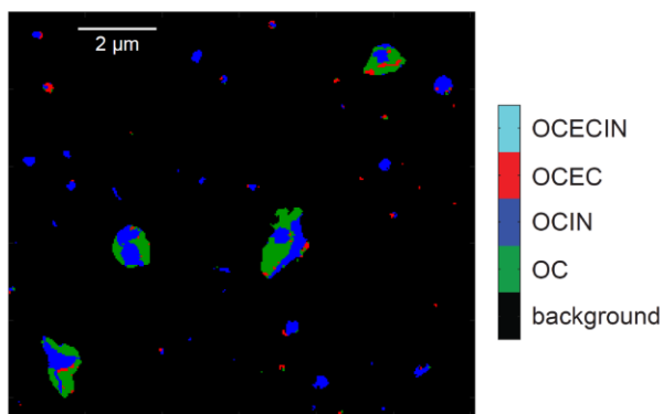
Figure 1: Representative STXM/NEXAFS analyses of marine boundary layer (MBL) particle samples as indicated by legends. From left to right: false-color particle maps that show particle mixing state composition where OCIN - organic carbonaceous-inorganic, OCEC - organic carbonaceous-elemental carbon, OC - organic carbonaceous. Normalized size-resolved mixing state analysis where IN - inorganic, EC - elemental carbon, OC - organic carbonaceous. Normalized size-resolved organic volume fraction (OVF) per particle where color green intensity represents OC fraction.
