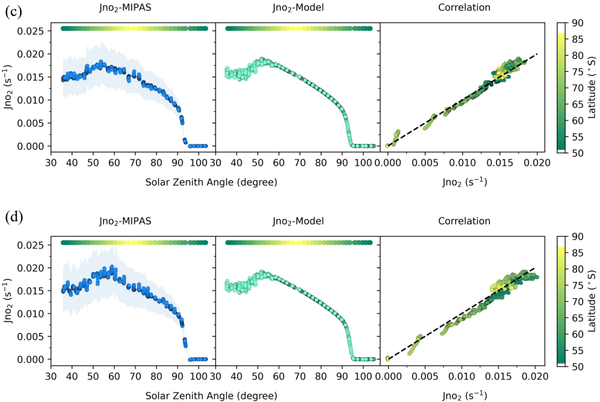
Figure 3. The J_{\text{NO}_2} in 50^{\circ} S- 90^{\circ} S from MIPAS and the model at different altitudes. (a) 23 km (b) 28 km (c) 33 km (d) 38km. The color bar represents the latitude of the data points at each solar zenith angle. In the correlation plots, the abscissa is J_{\text{NO}_2} -MIPAS and the ordinate is the J_{\text{NO}_2} -Model and the slope of dashed line is 1. To ensure clear visual distinction for each point, black outlines are applied around them.
