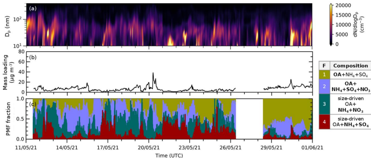
350 Figure 5. Time series of (a) particle size distribution ( dN/d\log D_p ) in \text{cm}^{-3} with logarithmic scale in particle size obtained from SMPS measurements, (b) total mass loading calculated from ACSM species concentration (using Tofware) in \mu\text{g m}^{-3} , and (c) reconstructed PMF fraction (stacked) from analysis in May 2021. Episodes of F4 and F3 coincide with relatively low total aerosol mass conditions and high fine particle concentrations. Similar figures for June and September 2021 can be found in Fig. S3.
