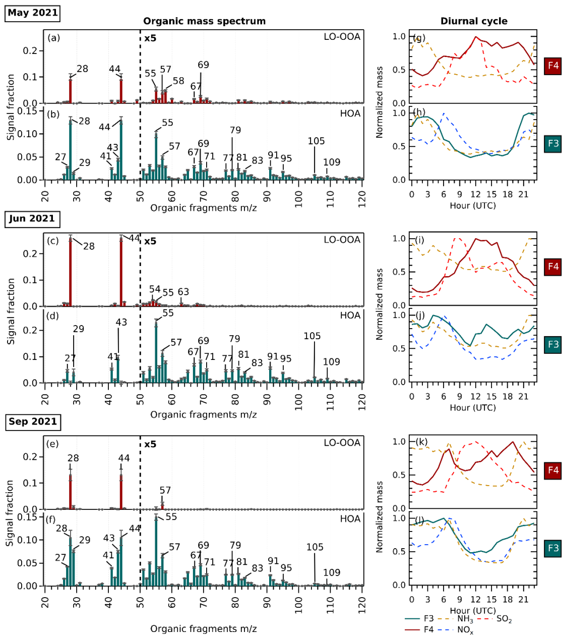
Figure 6. (a-f) Organic mass spectrum from m/z 20 to 120 (m/z < 20 not included) of F4 (maroon) showing LO-OOA factor profiles and F3 (turquoise) showing HOA factor profiles in May 2021, June 2021, and September 2021. The error bars in each m/z were generated from bootstrap run. (g-l) Diurnal cycles of corresponding factors and potential precursor gases. The diurnal cycles of F4, mainly composed of ammonium sulfate, are shown together with its precursors, NH 3 and SO 2 . The diurnal cycles of F3, mainly composed of ammonium nitrate, are shown together with its precursor, NH 3 and NO x .
