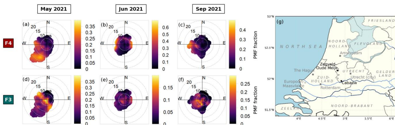
Figure 7. (a-f) Bivariate polar plots of size-driven factor mass fraction (F4 and F3) by wind speed and wind direction measured in Cabauw in May, June, and September 2021. We can observe that nucleation-mode particles (F4, a-c) fraction is largely correlated with air masses from the southwesterly-westerly sector where the urban and harbor areas of Rotterdam are located. The growth-mode particles (F3, d-f) fraction is distributed around the site and from southwesterly sector. Similar figures for composition-driven factors can be found in Fig. S7.
