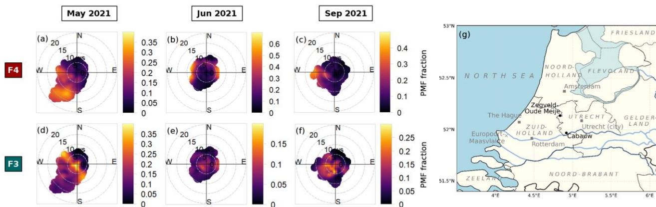
455 Figure 6. (a-f) Bivariate polar plots of size-driven factor mass fraction (F4 and F3) by wind speed and wind direction measured in Cabauw in May, June, and September 2021. We can observe that nucleation-mode particles (F4, a-c) fraction is largely correlated with air masses from the southwesterly-westerly sector where the urban and harbor areas of Rotterdam located. The growth-mode particles (F3, d-f) fraction is distributed around the site and from southwesterly sector. Similar figures for composition-driven factors can be found in Fig. S7.
