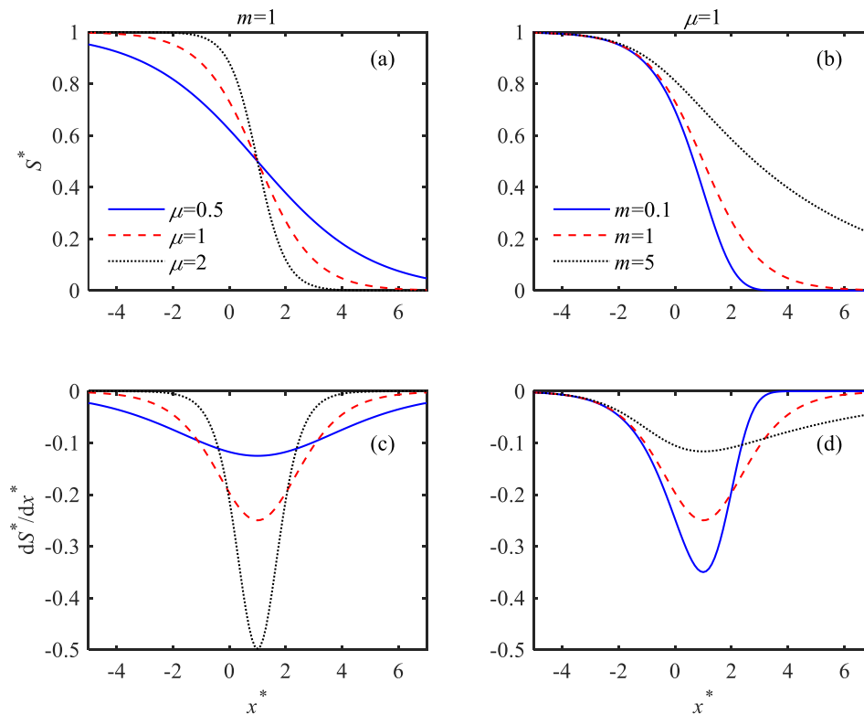
200 Figure 4. Sensitivity analysis of the dimensionless salinity S^* and its gradient dS^*/dx^* with regard to the recessing coefficient \mu and the rising coefficient m .
