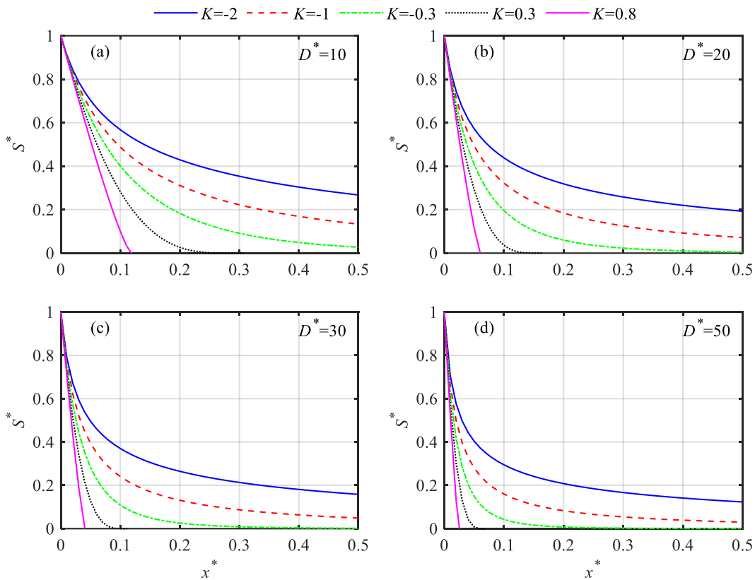
295 Figure 9. Longitudinal variation of the dimensionless salinity S^* computed using Eq. (18) along the estuary axis for different values of K and D^* when \gamma=1 .
