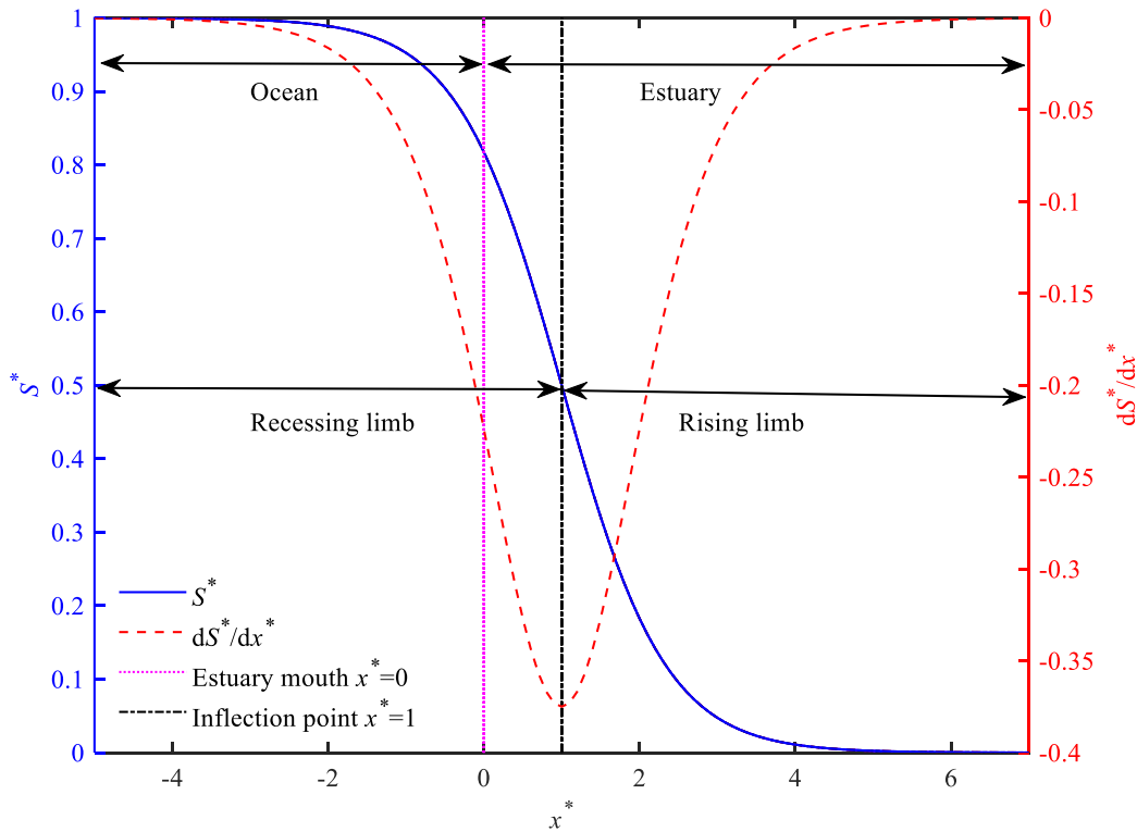
185 Figure 3. S-hydrograph S^* (salinity concentration) and its instantaneous UH dS^*/dx^* (salinity gradient) as a function of dimensionless distance x^* for given values of \mu=1.5 , m=1 .
