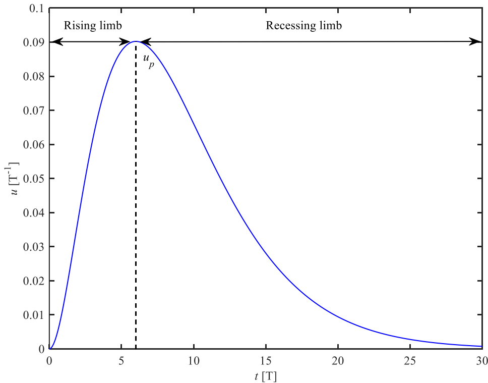
Figure 1. Illustration of the instantaneous UH analytically computed using Eq. (5) for given values of \alpha_1=\alpha_2=3 .
