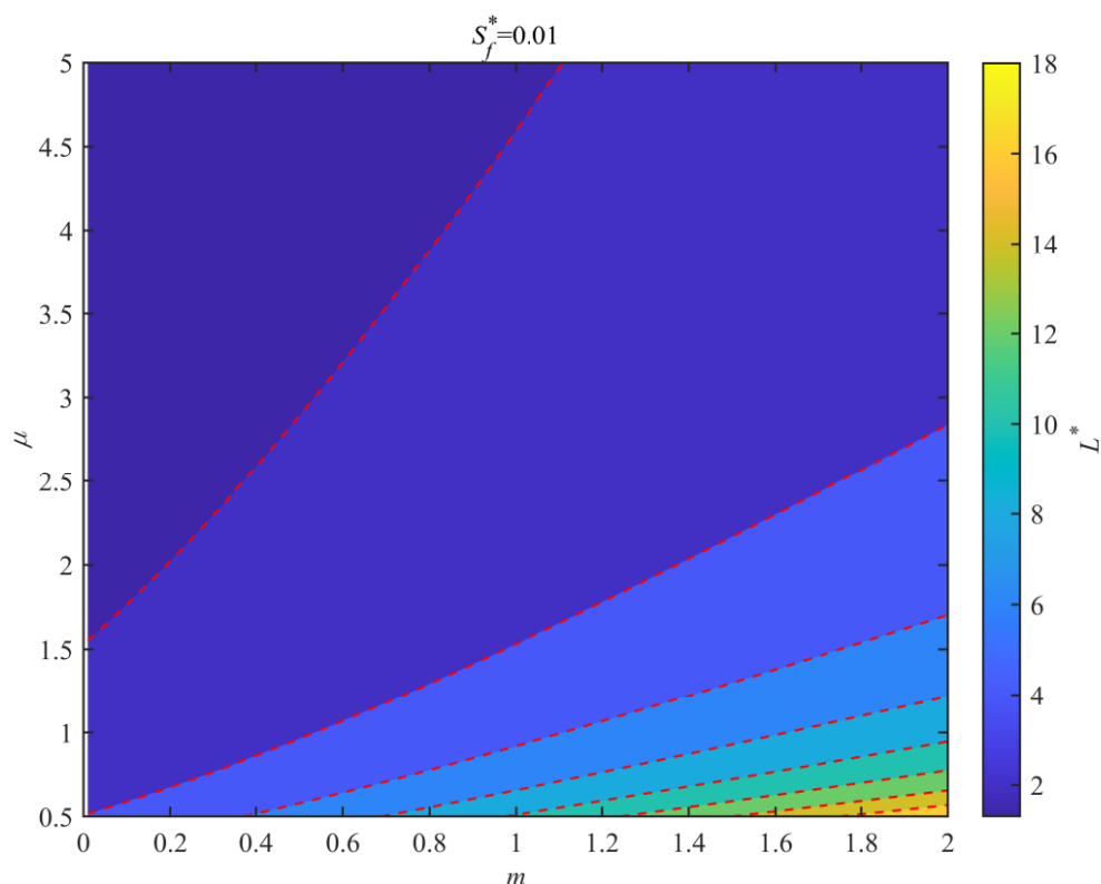
210 Figure 5. Response of salt intrusion length L^* to the dimensionless parameters \mu and m for a given salinity threshold S_f^*=0.01 .
