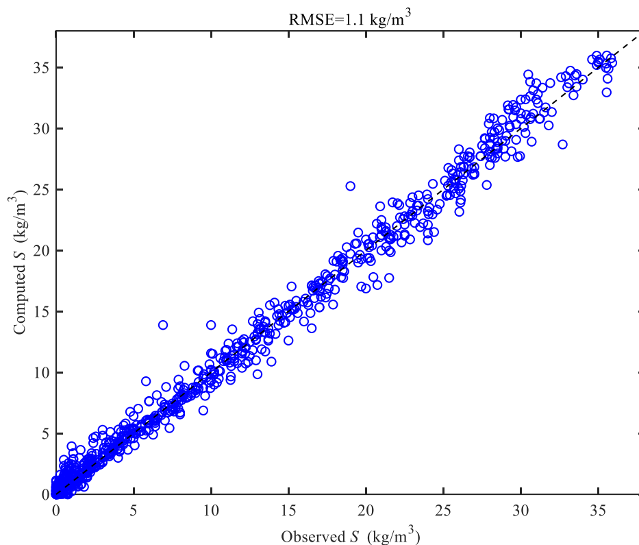
Figure 6. Comparison between analytically computed salinity concentrations and 89 observations in 21 estuaries worldwide.
