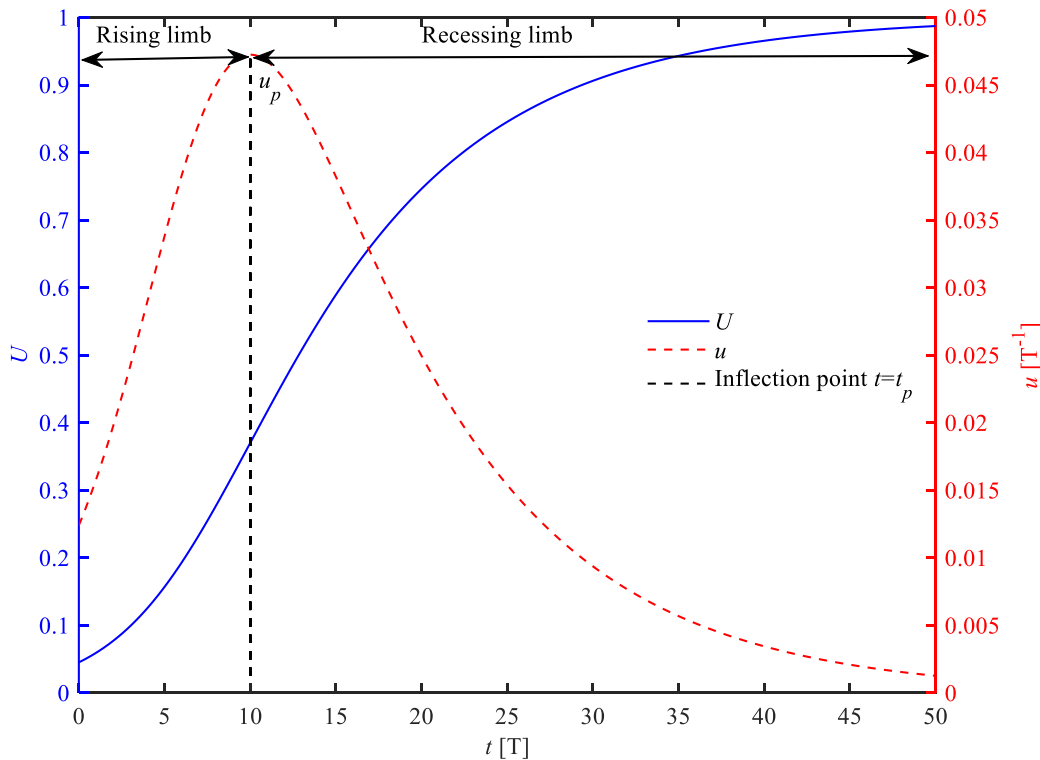
90 Figure 2. Illustration of the S-hydrograph and instantaneous UH analytically computed using Eqs. (6) and (8), respectively, for given values of \beta_1=\beta_2=3 and t_p=10 .
