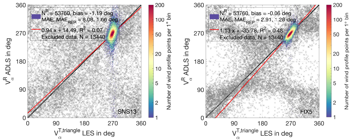
Figure B2. Histogram of ADLS retrieved wind direction compared to LES triangular volume input truth for the 2,5,10 and 15 \text{m s}^{-1} LES background wind cases and the standard SNS13 and FIX5 system flying in a crosswind direction. The 0 \text{m s}^{-1} background wind case is excluded as no meaningful wind direction can be defined for this case. Left panel: Results for SNS13 system. Right panel: Results for FIX5 system.
