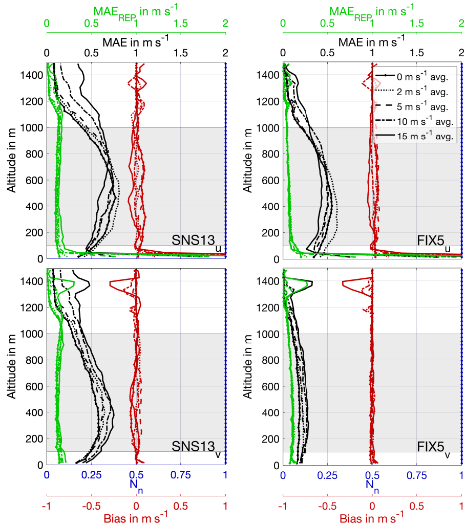
Figure 4. Retrieval quality parameters as a function of altitude for the standard SNS13 and FIX5 system flying in a crosswind direction. Left panels: SNS13 system. Right panels: FIX5 system. Top panels: Across-track (u) component. Lower panels: Along-track (v) component. Displayed are the quality metrics MAE_{REP} , MAE, N_n and Bias described in Sec. 2.5. The grey area illustrates the vertical section considered for overall quality analysis, system setup optimization and retrieval strategy.
