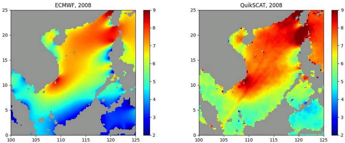
Figure A4: Sea surface wind speed ( \text{m s}^{-1} ) over the SCS averaged over the year 2008 computed from ECMWF 3-hourly analysis outputs (left) and daily QuikSCAT outputs (right).
