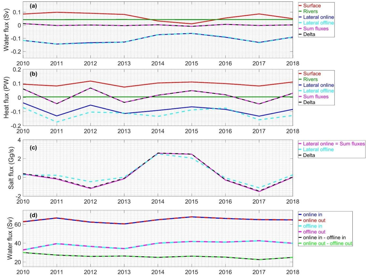
355 Figure 2 : Atmospheric (surface, red), river (green) and net lateral oceanic (blue online, cyan offline) annual fluxes of (a) water volume (Sv), (b) heat (PW) and (c) salt ( Gg.s^{-1} ) and their sum (magenta), and annual variations of water volume, heat and salt contents (black) over the period 2010 - 2018; (d) Annual lateral oceanic inflow (blue online, cyan offline) and outflow (red online, magenta offline) of water volumes (in absolute values) computed online and offline, and the difference online - offline (black for inflow, green for outflow).
