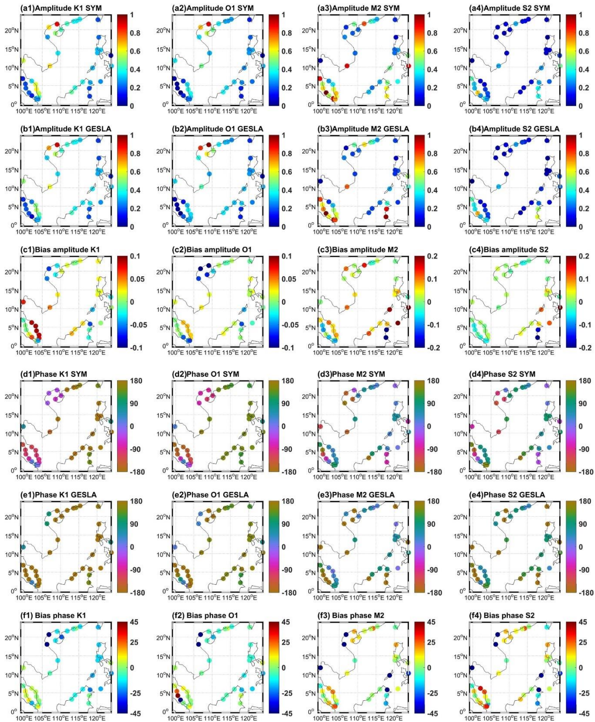
390 Figure 3 : Amplitude (m) and phase (degree) of four tidal components K1, O1, M2, S2 in SYM4 (SYM, a1-a4, d1-d4) and GESLA tide gauge dataset (b1-b4, e1-e4) and model bias compared to GESLA (c1-c4, f1-f4)
