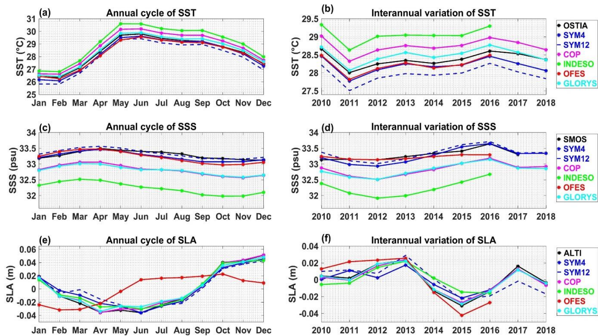
Figure 5 : Time series of climatological monthly mean (left, computed over 2010-2016, the period common to all models) and yearly mean (right, over 2010-2018 except for OFES and INDESO, available only until 2016) of SST ( ^{\circ}\text{C} , a, b), SSS (psu, c, d) and SLA (m, e, f) averaged over the SCS domain, computed from different models (SYM4, blue; SYM12 blue dashed line, COPERNICUS, magenta; INDESO, green; OFES, red; GLORYS, cyan) and from satellite observations (OSTIA, SMOS and ALTI, black).
