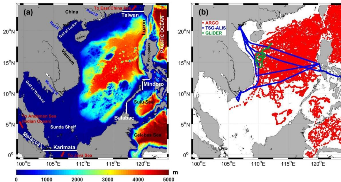
150 Figure 1: (a) Computational domain bathymetry (m) and interocean straits (white lines). (b) Maps of Argo float trajectories in the SCS from January 2009 to December 2018 (red), TSG from R/V Alis trajectory from May to July 2014 (blue), and Glider trajectory from January to May 2017 (green).
