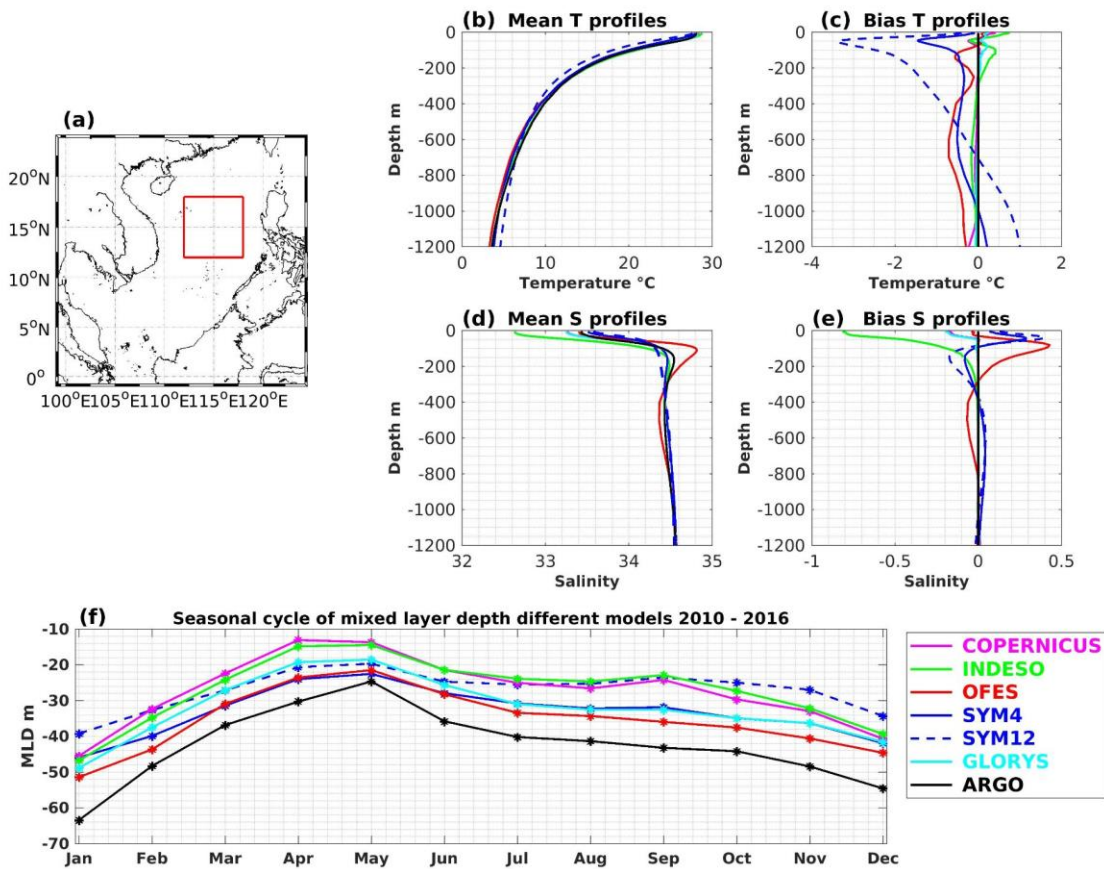
625 Figure 10 : (a) Comparison zone ( red box, 112-118°E, 12-18°N); Simulated (SYM4, SYM12, COPERNICUS, INDESO, GLORYS and OFES) and observed (Argo) temperature (b, °C) and salinity (d, psu) profiles averaged over the comparison zone and 2010-2016 and their biases (c,e) compared to Argo; (f) Climatological monthly time series of simulated and observed mixed layer depth over the comparison zone and the period 2010 - 2016.
