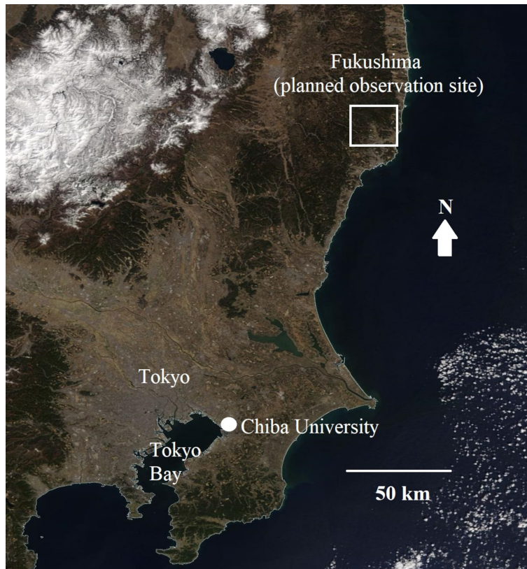
Figure 1. Location of Chiba University, the current observation site, with respect to Tokyo and Tokyo Bay. The next planned observation site will be in Fukushima. ( https://worldview.earthdata.nasa.gov/ ).
