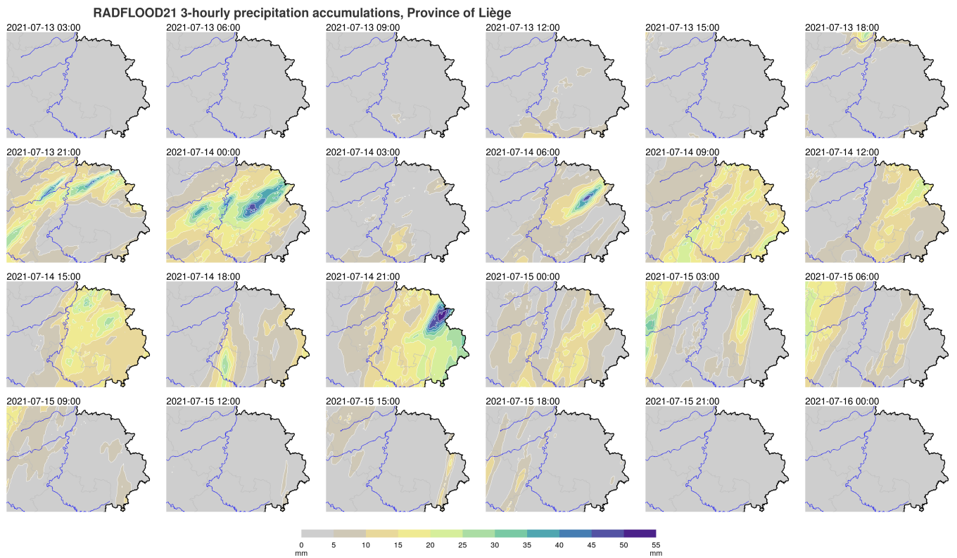
Figure E3. 3-hourly precipitation accumulations in the Province of Liège derived from 5-min radar product data. The timestamp on top of each map indicates the end of the 3-hour period in UTC.
