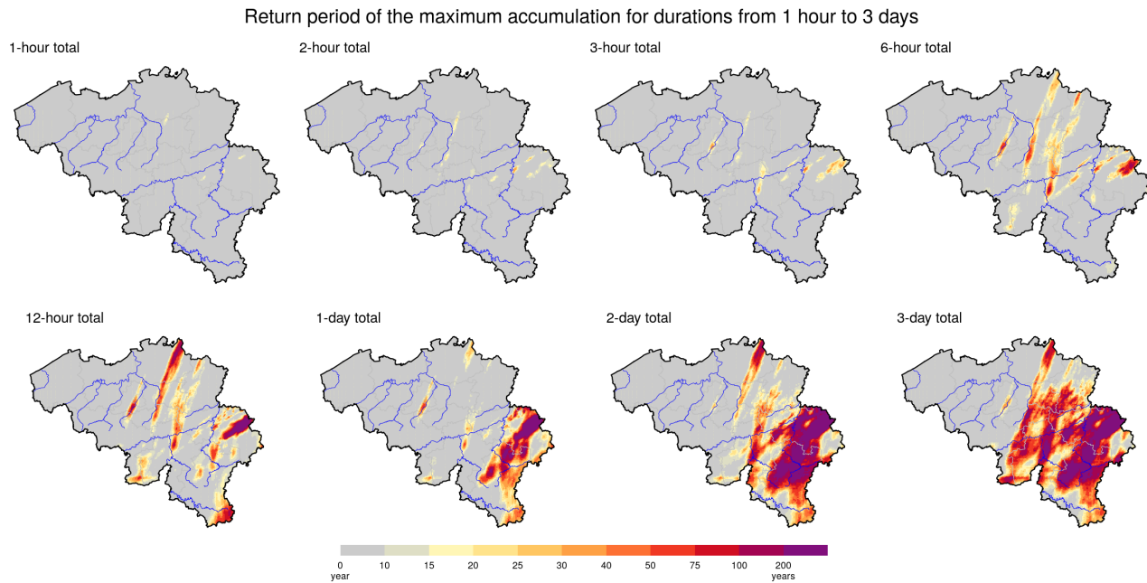
Figure E1. Return period estimated for the maximum precipitation accumulation between 13th July 06:00 UTC to 16th July 2021 06:00 UTC for durations from 1 hour to 3 days. The maximum accumulations are derived from hourly (resp. daily) radar product data for durations till 12 hours (resp. of 1, 2 or 3 days).
