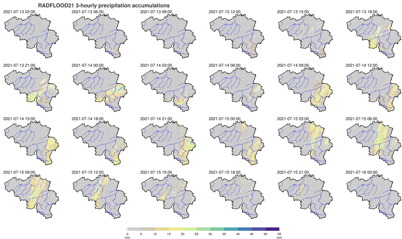
Figure E2. 3-hourly precipitation accumulations in Belgium derived from 5-min radar product data. The timestamp on top of each map indicates the end of the 3-hour period in UTC.
