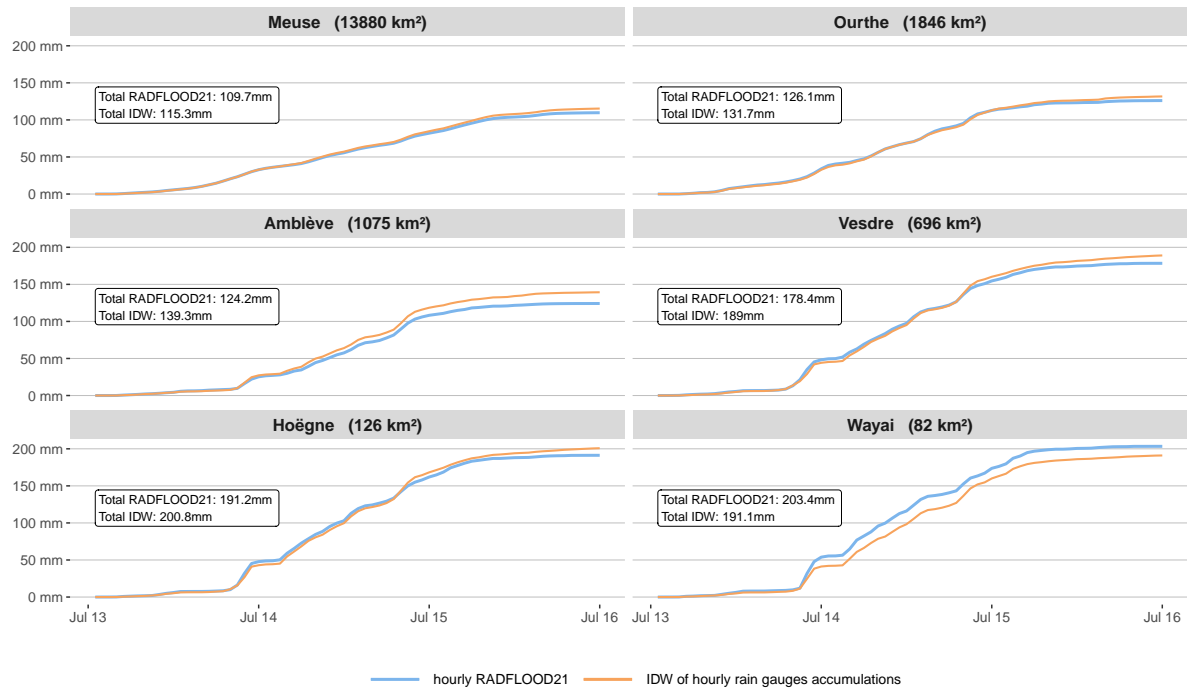
Figure E4. Cumulative precipitation sums derived from the hourly timeseries of areal rainfall averages illustrated for 6 selected catchments in Figure 12.
