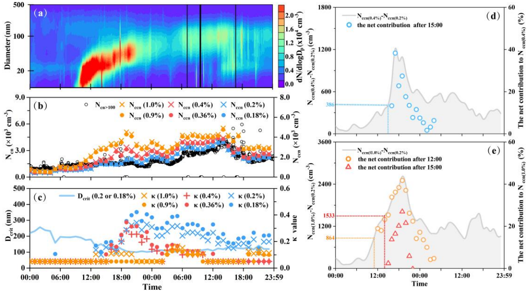
Figure 5. The contour plots of particle number size distribution (a); Time series for N_{cn>100} , N_{cn} at the lab-calibrated 0.2%, 0.4% SS, and the on-site approximated N_{cn} at 0.18%, 0.36% SS (b); Time series for D_{crit} at 0.2% or 0.18% SS, \kappa values at the lab-calibrated 0.2%, 0.4% SS, and the on-site approximated \kappa values at 0.18%, 0.36% SS (c); Time series of (N_{cn(0.4\%)} - N_{cn(0.2\%)}) and ratios of (N_{cn(0.4\%)} - N_{cn(0.2\%)})/N_{cn(0.4\%)} (d); Time series of (N_{cn(1.0\%)} - N_{cn(0.2\%)}) ratios of (N_{cn(1.0\%)} - N_{cn(0.2\%)})/N_{cn(1.0\%)} (e) on 1–2 July.
