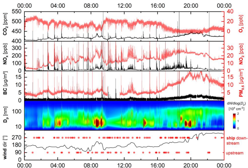
Figure 3: Exemplary time series for CO 2 , O 3 , NO x , NO 2 , BC, PM 0.5 (in this study similar to PM 1 and PM 2.5 ), dN/d\log(D_p) with number concentration N and particle diameter D_p , wind direction and ship travelling direction at BRI for 10 December 2021.
