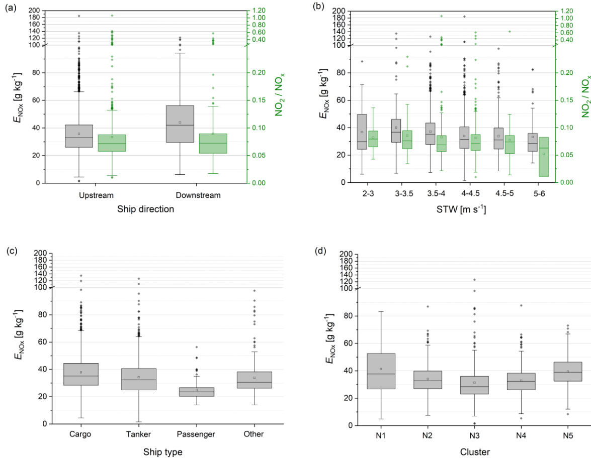
Figure 6: Influence of ship parameters on NO_x emission factor ( E_{NO_x} ) and NO_2 -to- NO_x ratio: (a) travelling direction, (b) speed through water (STW), (c) ship type and (d) clusters based on engine characteristics (see Table 3). For better readability the scaling of the y-axis was adapted for E_{NO_x} > 100\ g\ kg^{-1} respectively NO_2/NO_x > 0.25 .
