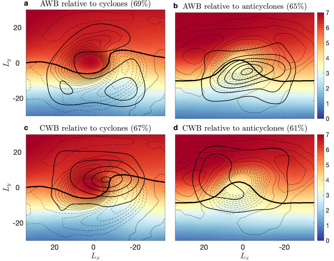
Figure 6. Composites of cyclones and anticyclones in the North-Atlantic. Upper-level (250 hPa) total PV (colors, in PVU) and PV anomaly (thin contours) centered on cyclones (a,c) and anticyclones (b,d) in the North-Atlantic region (30N-60N and 80W-20E) at the time of maximum intensity. The black contours show the PDF of AWB (a,b) and CWB (c,d) relative to the center of the surface weather systems, with lowest contour equal to 0.5 and the contour intervals are 0.2. The PDF values denote the number of events per bin area (which is 0.6^\circ in longitude and 0.6^\circ in latitude in this case). L_y and L_x denote the relative latitudinal and longitudinal distance (in degrees), respectively, from the center of the weather systems. The thick black line denotes the 4.5 PVU contour in panels (a) and (c), while it denotes the 5.5 PVU contour in panels (b) and (d). The percentages in each panel denote the percentage of systems in each composite with the corresponding RWB sense occurring sometime during their lifetime.
