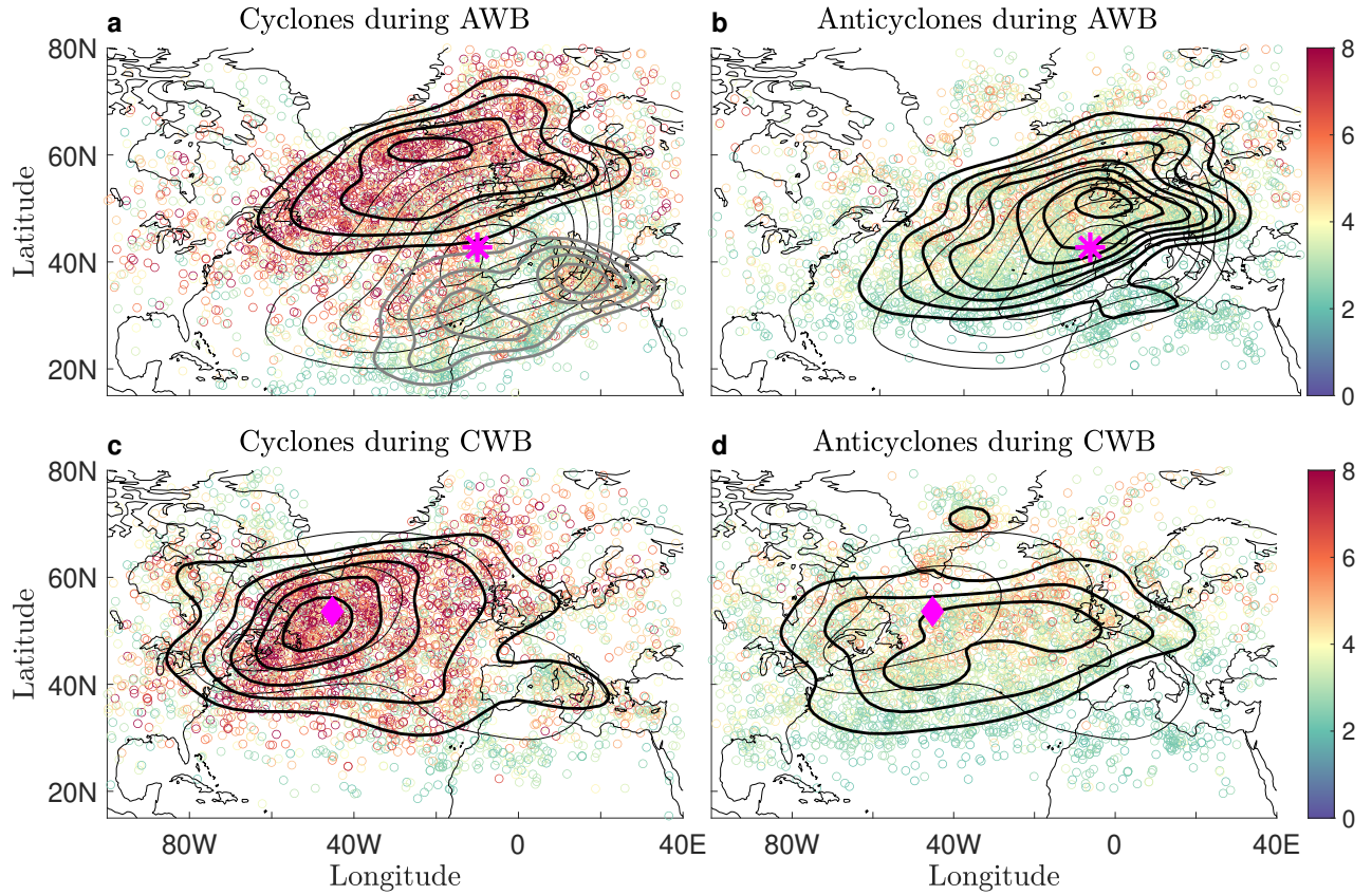
Figure 4. The actual spatial distributions of cyclones (a,c) and anticyclones (b,d) during AWB (first row) and CWB (second row), where color indicates the intensity of the system (in absolute value) in units of 10^{-5}\text{s}^{-1} , and only systems with intensities larger than 2 \cdot 10^{-5}\text{s}^{-1} are plotted. Thick black contours denote the PDFs of the weather system counts (calculated using a kernel density estimator and multiplied by the number of systems), showing the locations where the weather systems are mostly found. In panel (a), the PDFs are separated into cyclones residing to the north of the AWB center (black thick contours) and cyclones residing to the south of the AWB center (gray thick contours). The lowest contour is equal to 0.6 and the contour intervals are 0.25. For reference, the thin black contours show the PDFs of AWB (panels a,b) and CWB (panels c,d) as in Fig. 1c,d, with lowest contour is equal to 0.4 and contour intervals equal to 0.25. The magenta star (diamond) denotes the location where AWB (CWB) centroids are most frequently found. The PDF values denote the number of events per bin area (which is 4^\circ in longitude and 1^\circ in latitude in this case). Overall, there are 5,106 cyclones during AWB, of which 2,922 to the north and 2,184 are to the south of the AWB center (panel a). In addition, there are 4,216 cyclones during CWBs (panel c), 4,131 anticyclones during AWB (panel b), and 3,681 anticyclones during CWB (panel d). The same systems and RWB events are used to produce Fig. 3.
