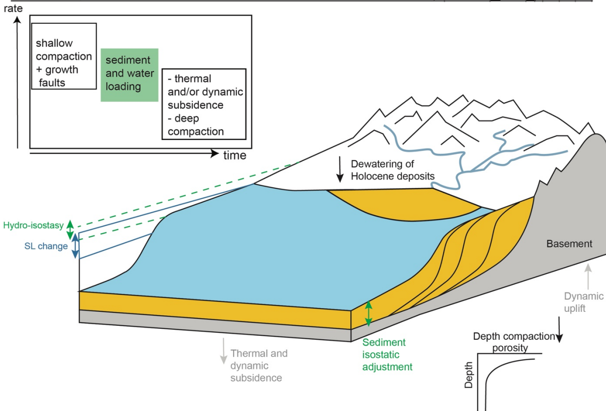
Figure 1. Conceptual diagram showing the components of vertical motions in passive margins with deltaic deposenters at different spatio-temporal scales. Rates of vertical motions are from Allen and Allen (2005); Jouet et al., (2008) and Frederick et al., (2019). Processes that can result in both uplift or subsidence, referred to as bidirectional, are shown in green. Sea-level change produces hydro-isostatic adjustments that affect both the landward portion of the continental margin and the ocean basin.
