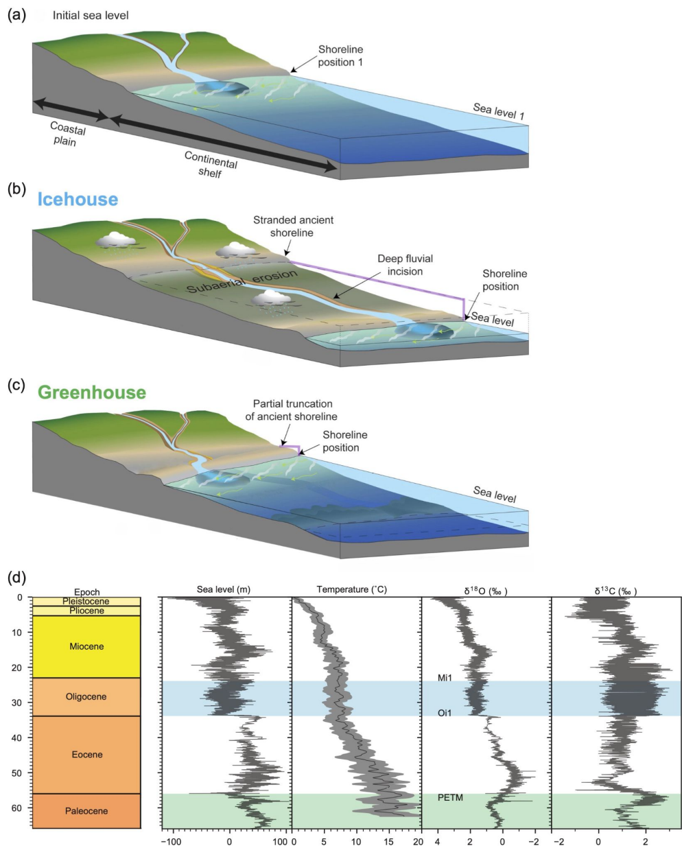
545 Figure 3. Conceptual model for the evolution of (a) deltaic depocenters in response to sea level changes during (b) icehouse and (c) greenhouse periods. The frequent and large amplitude variation of the sea-level (purple line) during icehouse periods results in the exposure of the continental shelf and deep fluvial incision and sediment loads being deposited deep into the basin. In contrast, during greenhouse periods the smaller amplitude of the sea-level variation (purple line) results in sediment being deposited closer to the continent. We test the flexural isostatic response of the aforementioned water and sediment partitioning. Figure modified from https://pubs.usgs.gov . (d) Evidence of the coupling between climate and global sea-level change that reflects global changes in ice volumes. The coupling is particularly strong in ice-free (ca. 66-56 Ma, greenhouse) and ice-dominated (ca. 33.9-23.9 Ma, icehouse) periods, which are the focus of this study. Data sources: sea level (Miller et al., 2020), temperature estimates based on Mg/Ca values (Cramer et al., 2011), benthic foraminiferal \delta^{18}\text{O} (Miller et al., 2020) and carbon isotope record \delta^{13}\text{C} (Zachos et al., 2001). 550
