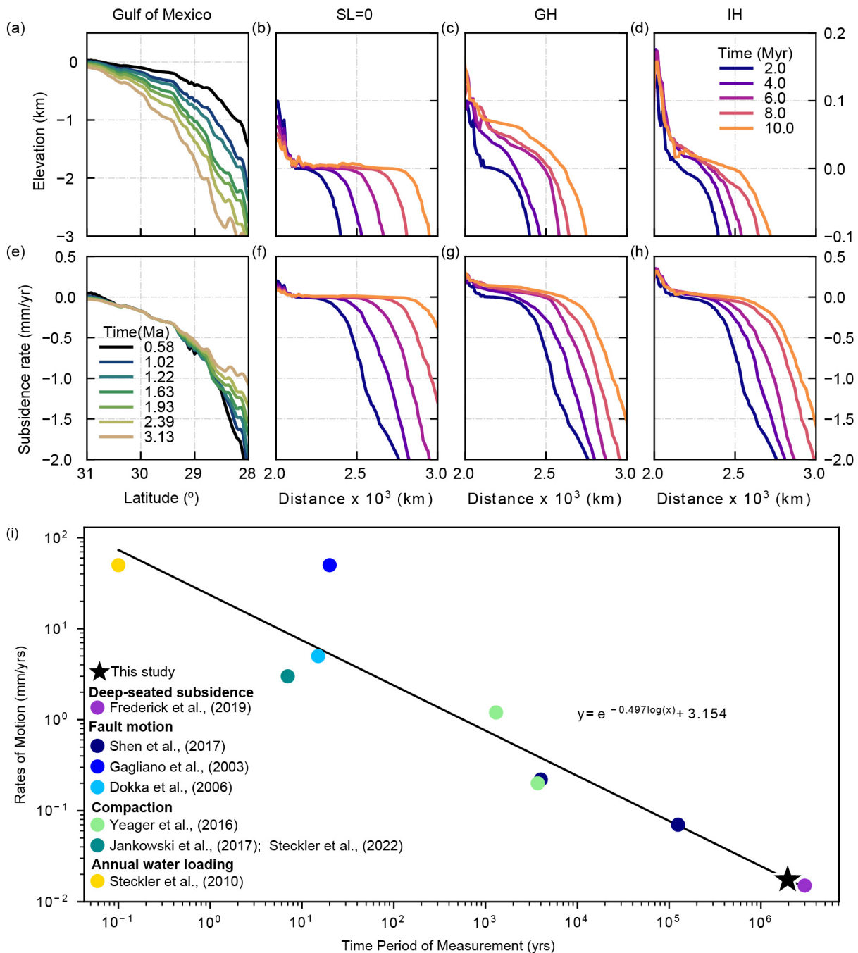
640 Figure 11. Elevation-bathymetry (top) and associated subsidence rates (bottom) from the Gulf of Mexico (a-e) and from simulations with no sea level change (SL=0, b, f) green house (GH c, g) and ice house (IH d, h). (i) Vertical rates of motion measured over different time scales, illustrating a “Sadler” type rate decrease as a negative log-log relationship with time scales of measurement.
