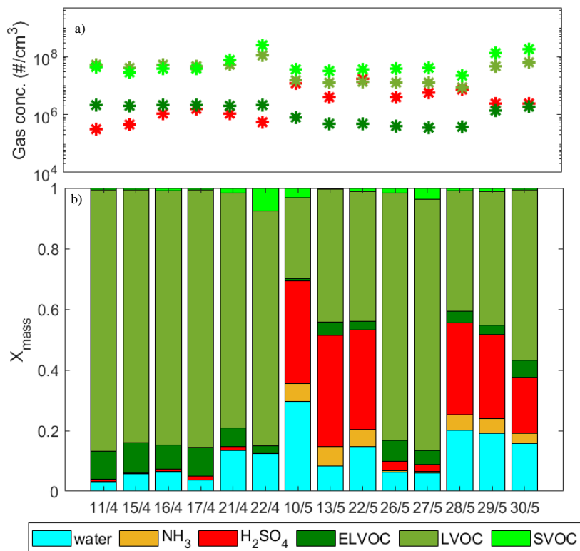
Figure 2. a) Mean vapor concentrations of sulfuric acid and organics and b) mass fractions of different compounds in the 340 nm particle in the model simulation for each analyzed day of NPF.
