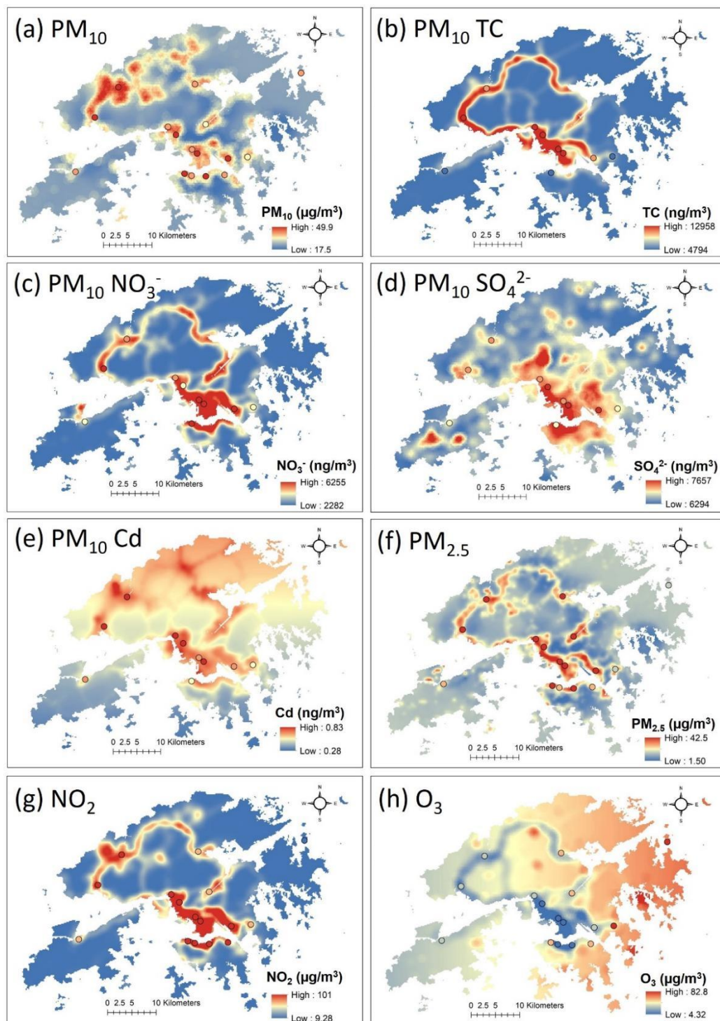
Figure 2. LUR model-derived spatial distribution maps of annual-average ambient PM_{10} , PM_{10} TC, PM_{10} NO_3^- , PM_{10} SO_4^{2-} , PM_{10} Cd, PM_{2.5} , NO_2 , and O_3 concentration in Hong Kong. The colored circles represent observations at AQMSs.
