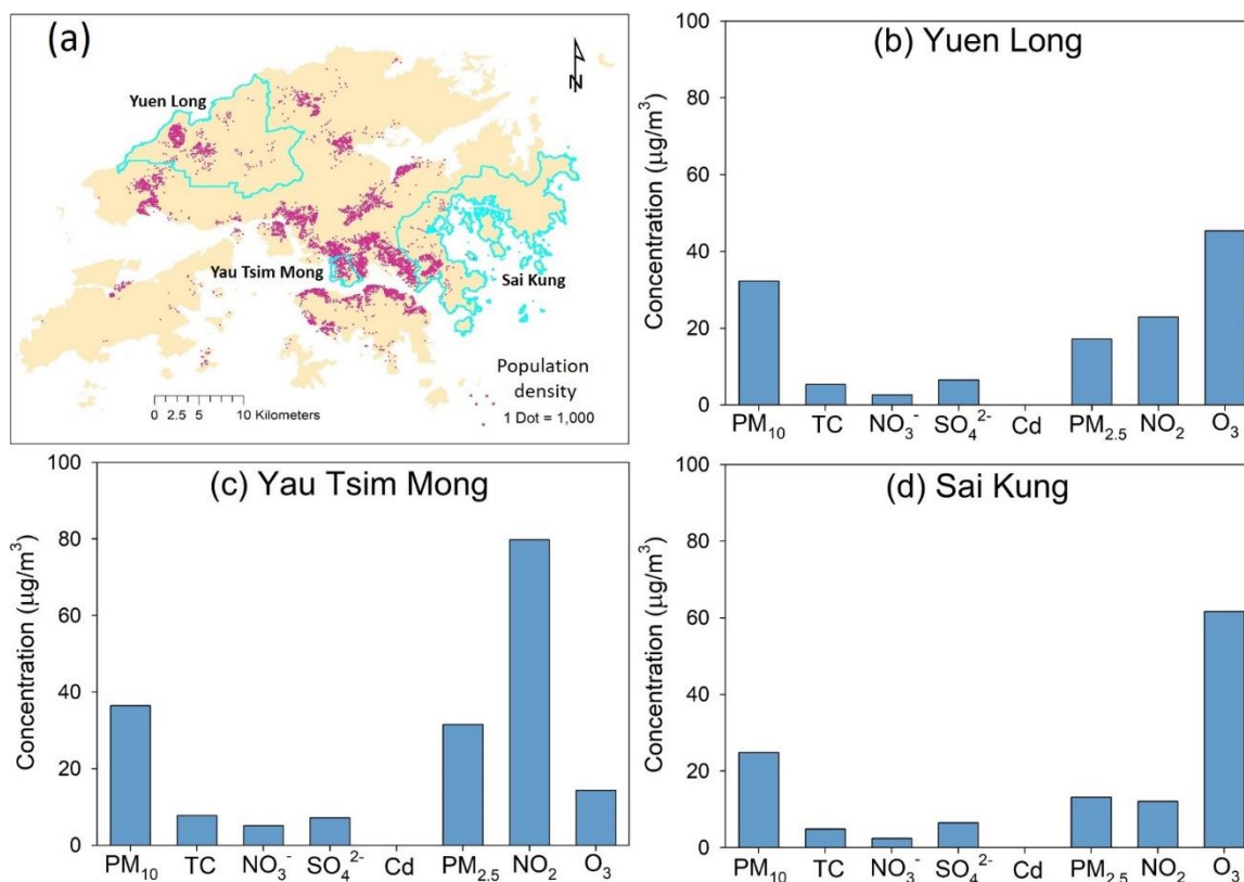
490 Figure 3. The average LUR estimated ambient PM 10 , PM 10 TC, PM 10 NO 3 - , PM 10 SO 4 2- , PM 10 Cd, PM 2.5 , NO 2 , and O 3 concentration in three representative districts in Hong Kong. (a) The distribution of Yuen Long, Yau Tsim Mong, and Sai Kung districts in Hong Kong with the population density shown. (b) Yuen Long (a district more influenced by the transboundary pollution). (c) Yau Tsim Mong (a high-density district more influenced by vehicular emissions). (d) Sai Kung (a rural district).
