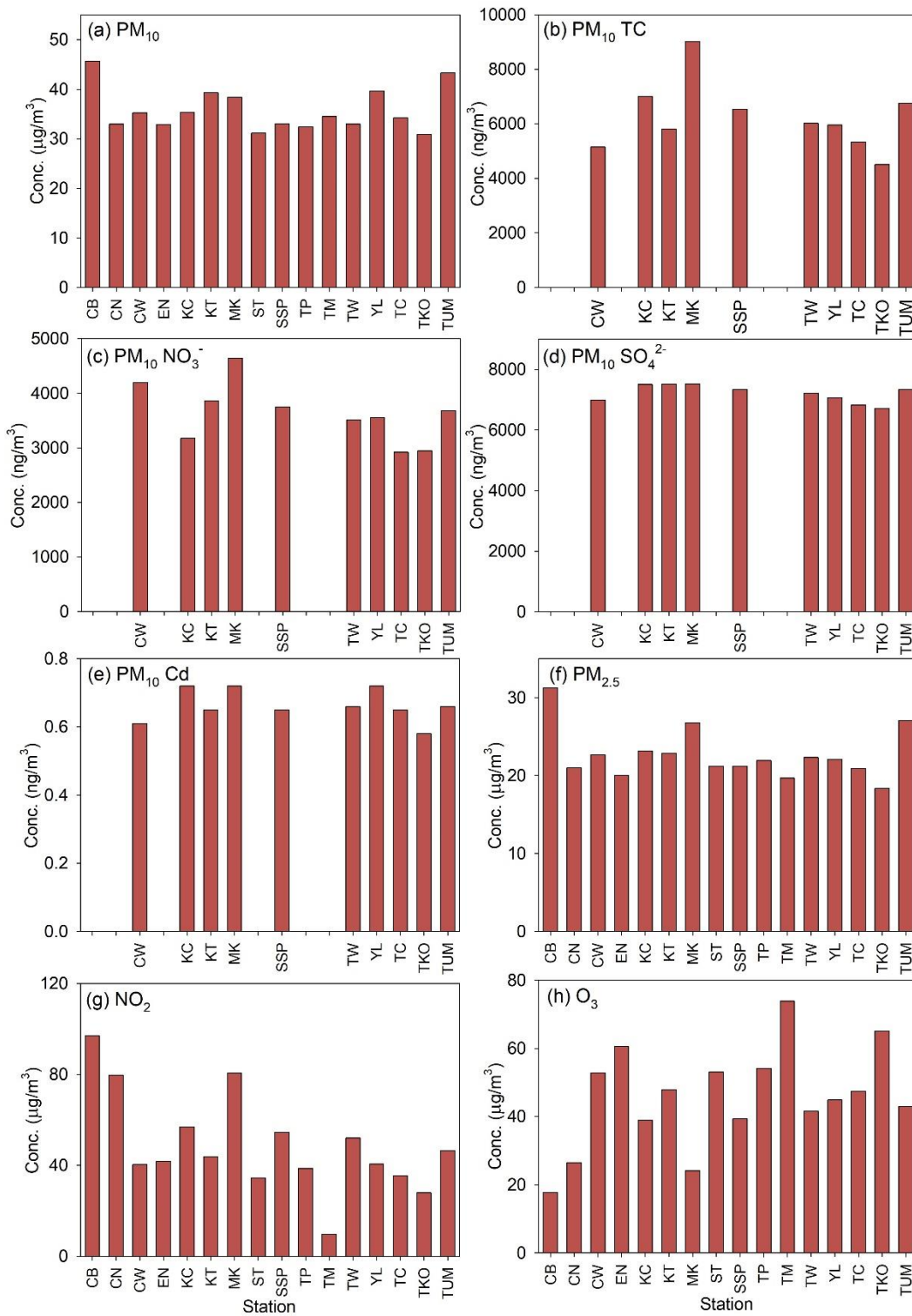
90 Figure S3. Annual-average concentration of PM_{10} , PM_{2.5} , NO_2 , O_3 , and four major PM_{10} chemical species at general and roadside stations.
