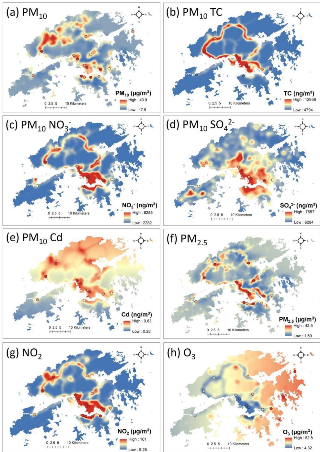
Figure 3. LUR model-derived spatial distribution maps of annual-average ambient PM_{10} , PM_{10} TC, PM_{10} NO_3^- , PM_{10} SO_4^{2-} , PM_{10} Cd, PM_{2.5} , NO_2 , and O_3 concentration in Hong Kong. The colored circles represent observations at AQMSs.
