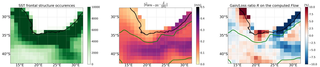
Figure 9. Geographical distribution of: the frontal structure occurrences during the ten years of comparison (left), the averaged BFN-QG currents crossing the SST fronts (middle) and the gain/loss ratio R on the computed Flow (as for figure-Figure 3 , negative/blue values indicate better performances for the BFN-QG method compared to DUACS). The green contour is the 200 \text{ cm}^2 SSH variance contour.
