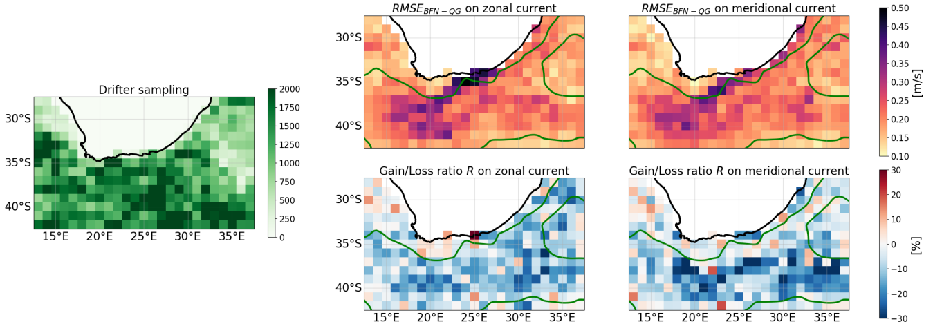
Figure 6. Geographical statistics of the V-mapping-Velocity-mapping performances for the ten years (from 2010 to 2019). On the left panel: independent drifter sampling. On the right panels: RMSE of the BFN-QG (top) and the gain/loss ratio R with respect to DUACS (bottom) for the zonal (left) and meridional (right) currents. Negative values (blue) indicate better performances for the BFN-QG method compared to DUACS. The green contour is the 200 \text{ cm}^2 SSH variance contour.
