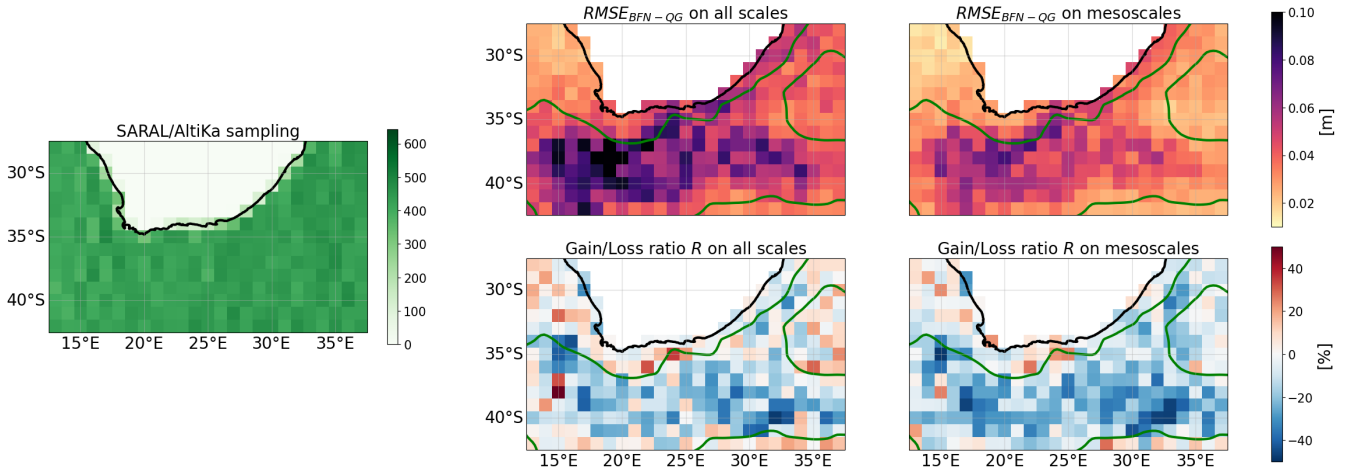
Figure 3. Geographical statistics of the SLA-mapping performances for the year 2019. On the left panel: number of independent SARAL/AltiKa altimeter sampling data available . On the right panels: RMSE of the BFN-QG (top) and the gain/loss ratio R with respect to DUACS (bottom) for all spatial scales (left) and mesoscales (right). Negative values (blue) indicate better performances for the BFN-QG method compared to DUACS. The green contour is the 200 \text{ cm}^2 SSH variance contour.
