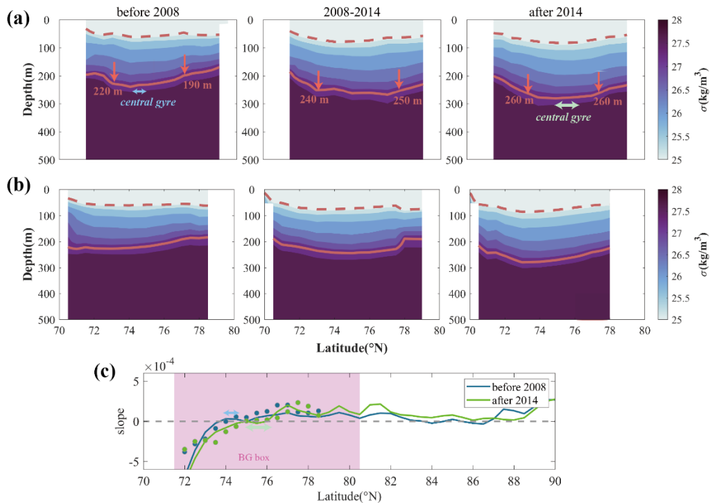
270 Figure 4. Vertical transects along (a) 150°W and (b) 140°W of interannual mean potential density using data from CTD measurements in 2004–2007 (before 2008), 2008–2014, and 2015–2021 (after 2014). The dashed (solid) lines indicate the depth of \sigma = 25 ( 27.4 ) \text{kg}\cdot\text{m}^{-3} representing the the halocline top (base). The depths of halocline base on either side of that is at least 120 km from central gyre are marked in the upper panel. (c) Meridional slope of isopycnal \sigma = 27.4 \text{kg}\cdot\text{m}^{-3} in first and last periods from SODA (solid line) and CTD (dot).
