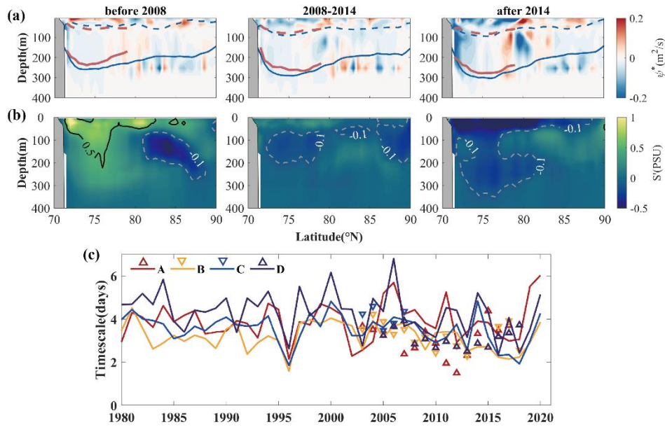
Figure 11. Transects of (a) eddy stream function and (b) salinity anomaly relative to the whole term averaged in 2004–2007 (before 2008), 2008–2014, and 2015–2020/2021 (after 2014), calculated from SODA simulated now until 2020 and CTD observed until 2021. The dashed (solid) lines indicate the processed annual mean depth of isopycnal surface \sigma = 25 (27.4) \text{kg}\cdot\text{m}^{-3} representing the halocline top (base) from SODA (blue lines, selected data are from September to October, which is mostly consistent with the observed data for CTD deployment) and CTD (red lines) during three periods. (c) Annual mean time series of the Eady timescale calculated from SODA (solid line) and MMP (triangle) at four moorings.
