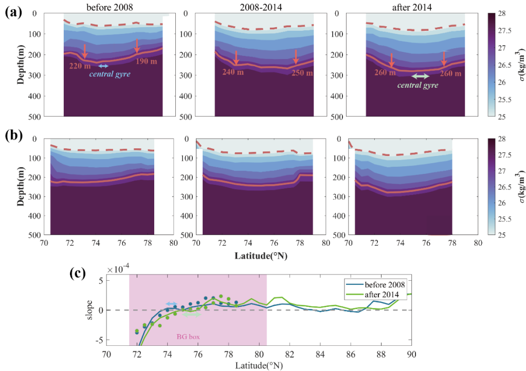
Figure 4. Vertical transects along (a) 150°W and (b) 140°W of interannual mean potential density using data from CTD measurements in 2004–2007 (before 2008), 2008–2014, and 2015–2021 (after 2014). The dashed (solid) lines indicate the depth of \sigma = 25 ( 27.4 ) \text{kg}\cdot\text{m}^{-3} representing the the halocline top (base). The depths of halocline base on either side of central gyre are marked in the upper panel. (c) Meridional slope of isopycnal \sigma=27.4\text{ kg}\cdot\text{m}^{-3} in first and last periods from SODA (solid line) and CTD (dot).
