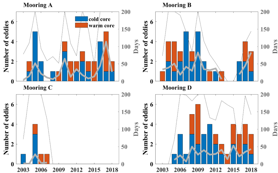
330 Figure 5. Interannual evolution of the days of existing eddies (thick grey line) and number of eddies (bar) for four moorings. The blue and red bars indicate the counts of cold-core and warm-core eddies, respectively. Thin grey lines signify the days of recording valid observations in every year.
