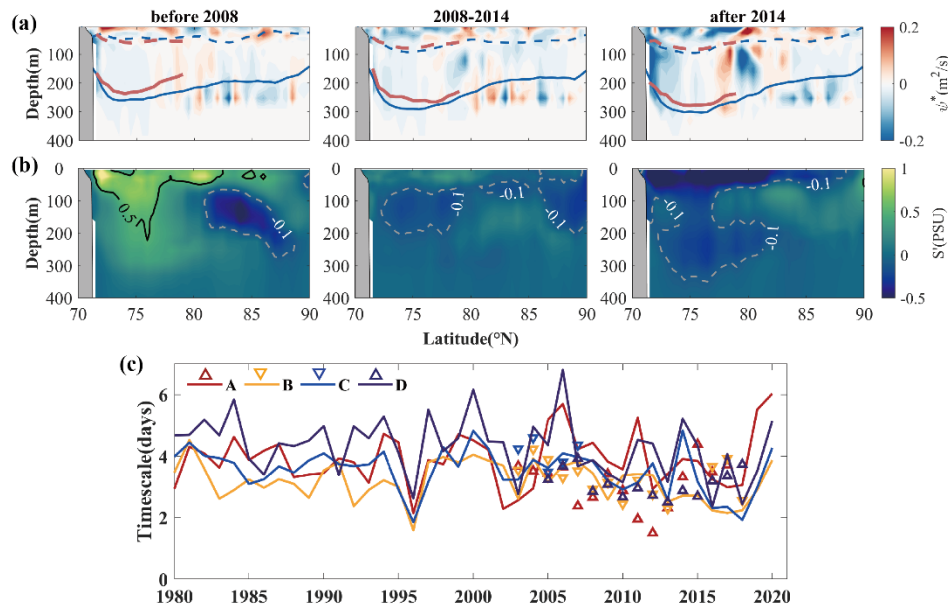
470 Figure 11. Transects of (a) eddy stream function and (b) salinity anomaly relative to the whole term averaged in 2004–2007 (before 2008), 2008–2014 and 2015–2020/2021 (after 2014), calculated from SODA simulated now until 2020 and CTD observed until 2021. The dashed (solid) lines indicate the processed annual mean depth of isopycnal surface \sigma = 25 (27.4) \text{kg} \cdot \text{m}^{-3} representing the halocline top (base) from SODA (blue lines, selected data are from September to October, which is mostly consistent with the observed data for CTD deployment) and CTD (red lines) during three periods. (c) Annual mean time series of the Eady timescale calculated from SODA (solid line) and MMP (triangle) at four moorings.
