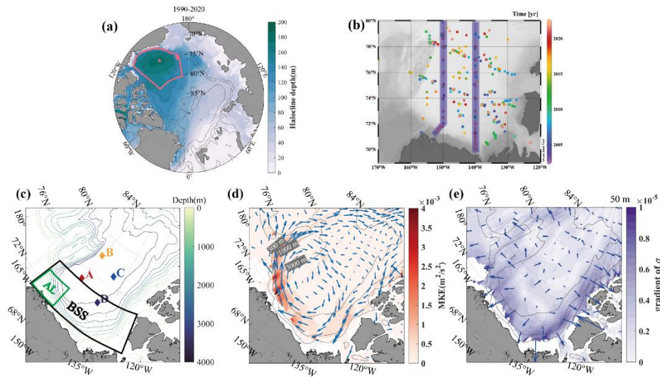
125 Figure 1. (a) A map of climatology halocline depth. Pink box and star indicate the BG area and center , referring to Regan et al. (2020). This BG box is defined as the region between 70.5–80.5°N and 170–130°W, bounded by the 300 m bathymetry. The 130 center of the mean gyre from 1990 to 2014 is situated at 74.74°N and 150.62°W. (b) The positions of in situ sites of CTD measurement from BGEP in certain months during 2004–2021. The purple bars indicate two meridional transects with a width of 36 km mostly along 150°W and 140°W. (c) A map of the Canada Basin and the bathymetric contours above the 4000 m isobath. Coloured diamonds denote the locations of four BGEP moorings. The two chosen regions are shown by green (AL, Alaskan coast) and black (BSS, Beaufort Sea slope) boxes. (d) The distribution of mean kinetic energy (MKE) at 50 m. Vectors denote the direction of mean currents. Grey lines denote the 300 m, 1000 m, and 3000 m bathymetry. (e) The distribution of horizontal gradient of potential density (shading) at 50 m. Vectors point in the direction of increasing potential density. The results of (a), (d), and (e) are calculated from the 1990–2020 WOA climatology.
