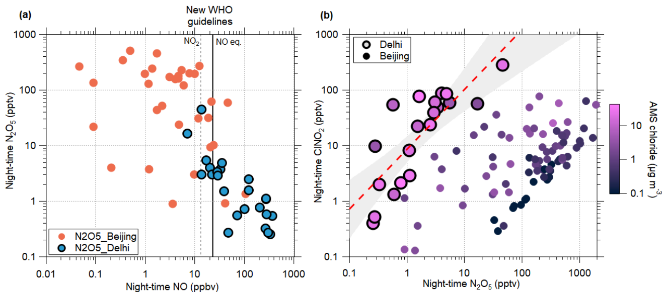
385 Figure 5: Relationships between night-time CINO_2 , N_2O_5 and NO during the study period. (A) Average nocturnal concentrations of N_2O_5 plotted against average nocturnal concentrations of NO, for our campaign results from Delhi and from measurements in Beijing from 2020. The new 24-hour WHO guideline for NO_2 concentrations is displayed by the dashed grey line, with the calculated NO equivalent shown by the solid black line. (B) Relationship between nocturnal CINO_2 and N_2O_5 . Colouring shows the average particulate chloride concentration, as measured by the AMS. The red dashed line shows the least-squares regression line for the Delhi dataset, with 95% confidence intervals shown in grey. The equation for the line is given by the equation \ln(CINO_2 (pptv)) = 1.08 \ln(N_2O_5 (pptv)) + 2.16 . Data points from between 20:00 and 05:00 the following morning are included.
