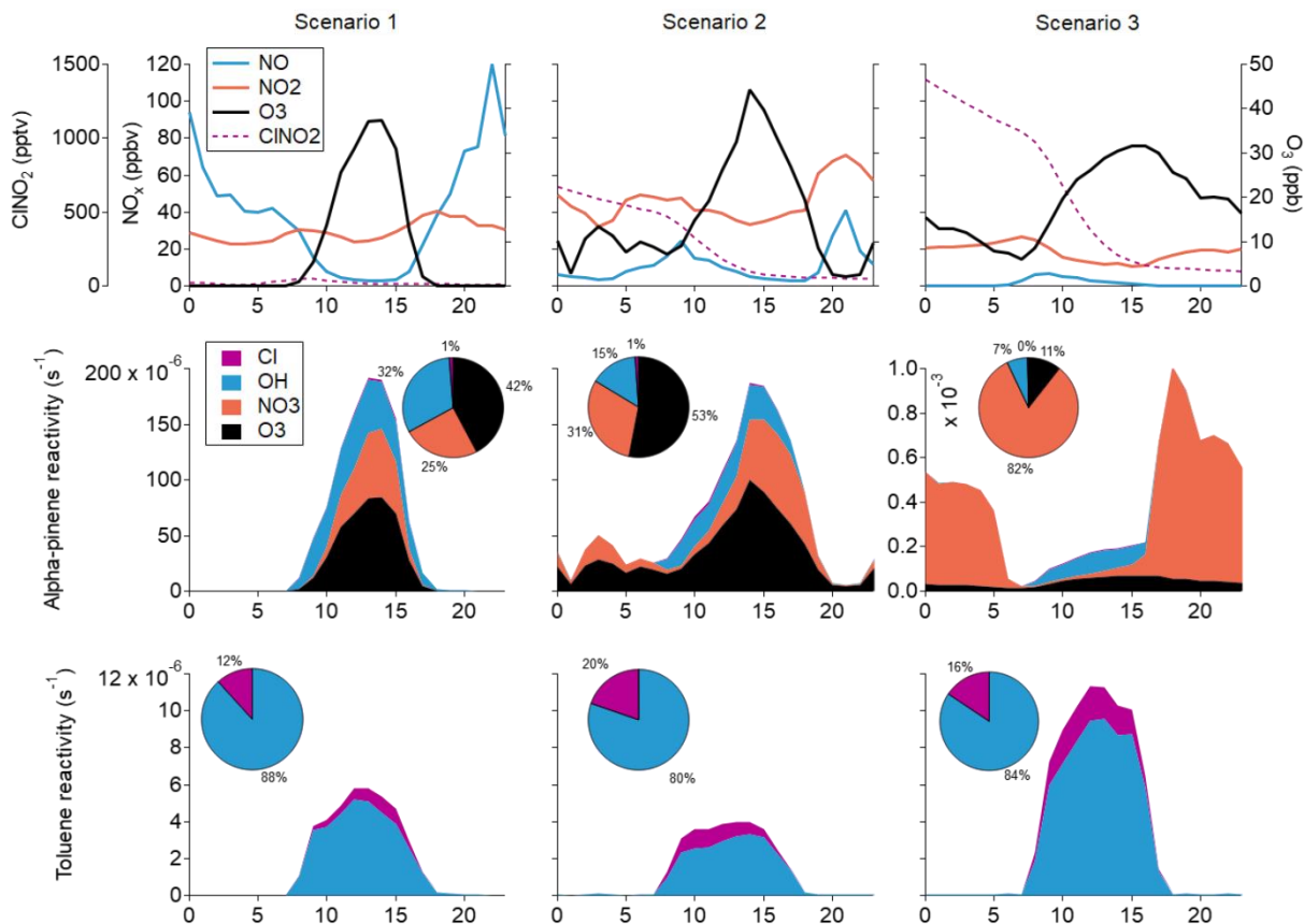
Figure 6: The reactivity of toluene and alpha-pinene under three simulated scenarios. (A), (B) and (C) show the NO, NO 2 , O 3 and CINO 2 concentrations for scenarios 1, 2 and 3, respectively. In all three cases, NO and NO 2 values in the model are held to the measurements, as is O 3 in scenarios 2 and 3. For CINO 2 , the initial value is fixed and evolves throughout the model run for scenarios 2 and 3. (D), (E) and (F) indicate the reactivity of alpha-pinene in scenarios 1, 2 and 3 respectively, and (G), (H) and (I) the reactivity of toluene.
