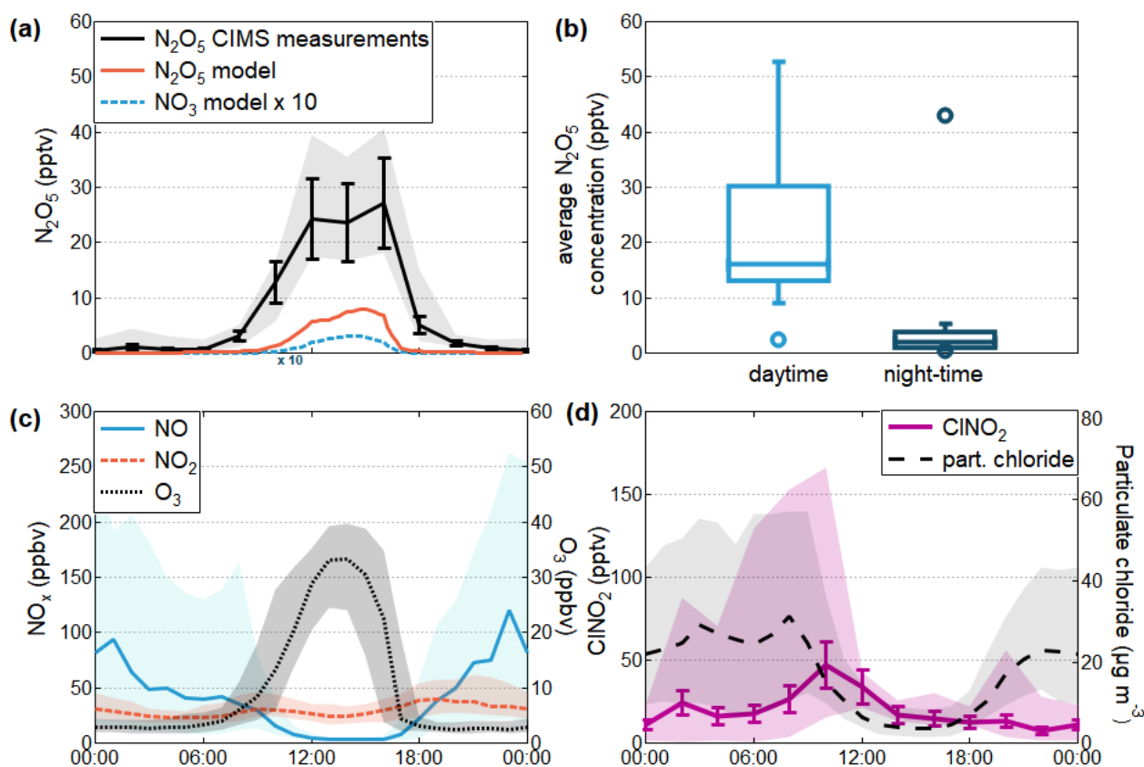
Figure 3: Median diel patterns during the period from 11 Jan – 5 Feb 2019, for the key compounds explored in this study. (a) The median diel cycle of \text{N}_2\text{O}_5 measured by the FIGAERO-CIMS with the interquartile range shaded, alongside the \text{N}_2\text{O}_5 and \text{NO}_3 simulations from the 0D box model. Error bars indicate a potential 30% error in the estimated calibration constant. (b) Box plots showing the average \text{N}_2\text{O}_5 concentrations throughout the campaign during the day and the night as measured by the FIGAERO-CIMS, indicating that there is a distinct and consistent decrease in \text{N}_2\text{O}_5 concentrations at night. (c) The observed median diel
