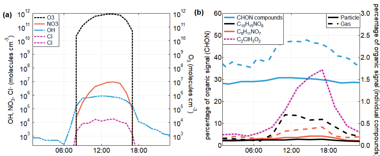
305 Figure 4: The diel cycles of key oxidants and oxidation products in Delhi during the study period. (a) The diel cycle of four key oxidants, O 3 , Cl, NO 3 and OH. The Cl concentration has been estimated from chlorine-containing species observed by the FIGAERO-CIMS (Methods). Estimated concentrations of the other three oxidants are calculated using the Framework for 0-D Atmospheric Modelling (F0AM) chemical box model (Wolfe et al., 2016) (Methods). (b) The diel cycles of total N-containing organics in the gas and particle phases (blue) with selected compounds C 8 H 11 NO 7 (orange) and C 10 H 15 NO 6 (black) also displayed in both the gas and particle phases. These two compounds, both associated with NO 3 oxidation, are most prevalent during the day when the NO 3 concentration peaks, while compounds associated with biomass burning are more prevalent at night (Fig. S6). The diel cycle of C 2 H 3 O 2 Cl, a known tracer of Cl chemistry, is shown in pink. These compounds were not calibrated, so here the percentage contribution of each compound or group of compounds towards the total organic signal is displayed on the y-axes. 310
