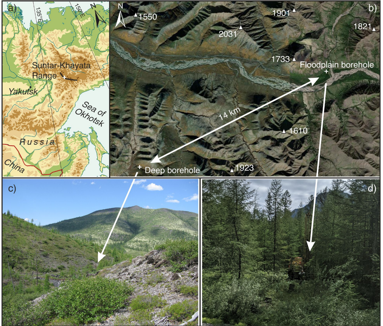
299 Figure 1. Study area description and picture of sites environment. In (a) a modified physical map of the location of the study 300 area in eastern Siberia is shown (Map source: © GEOATLAS 1998). (b) MAXAR image of Vostochnaya Khandyga basin 301 with altitudes of peaks. (c) Deep borehole site at V-shaping valley. (d) Shallow borehole site at river plain.
