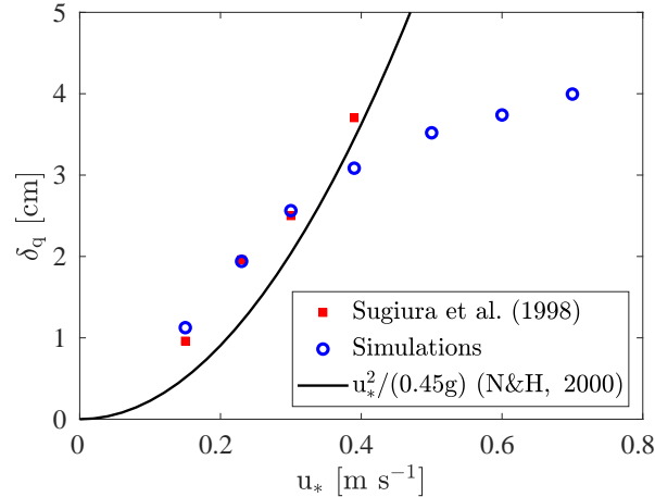
Figure 4. Decay height obtained by fitting the mass flux profiles presented in Fig. 3 with Eq. (4). The values reported by Sugiura et al. (1998) and the expression proposed by Nishimura and Hunt (2000) (N&H, 2000) are also presented for comparison.
