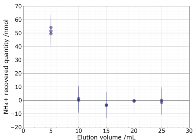
Figure 4: 50 nmol NH 4 + recovered quantity after 5 mL elution fractions with measurement uncertainty shown by vertical bars.
