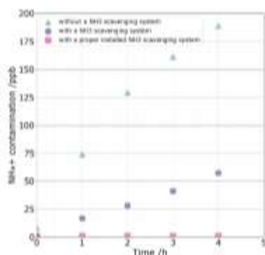
320 Figure 3: \text{NH}_4^+ contamination levels reported every hour under standard fume hood (green triangle), and under the \text{NH}_3 scavenging fume hood after installation (purple circle), and after changing the filter (pink square).
