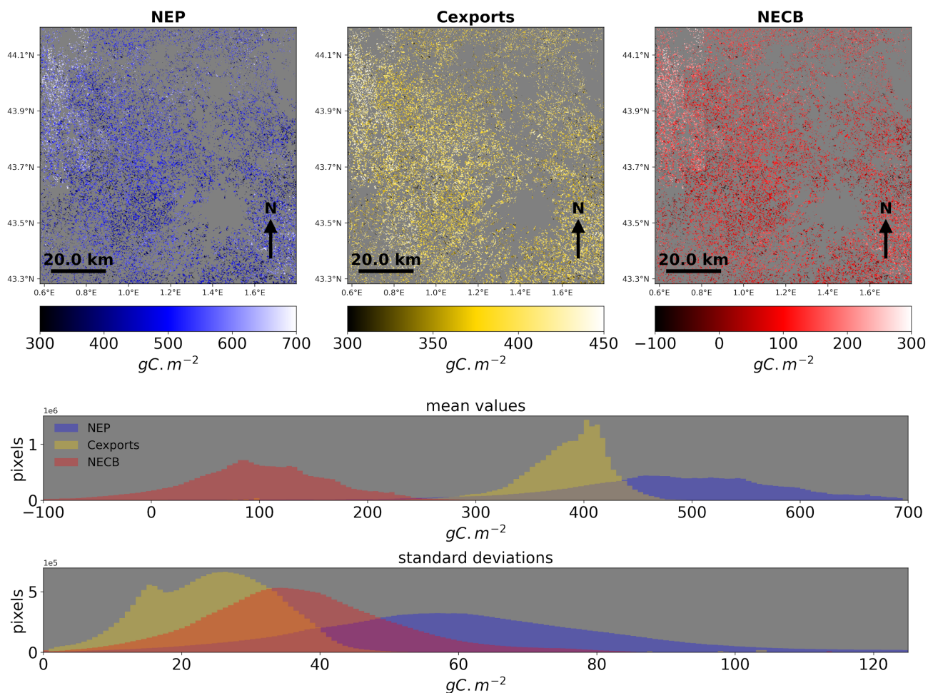
Figure 6. Regional scale carbon budget outputs from AgriCarbon-EO assimilation using S2 and L8. In "A": From left to right, NEP , Cexports (yield), and NECB for the winter wheat fields for the 2016-2017 cropping season. In "B": the histogram of the posterior mean and standard deviation of the same variables on top and bottom, respectively. Note that NEP and NECB are presented in the soil-oriented convention. Positive values of NEP and NECB thus correspond to net annual CO_2 sinks and soil organic carbon storage, respectively.
