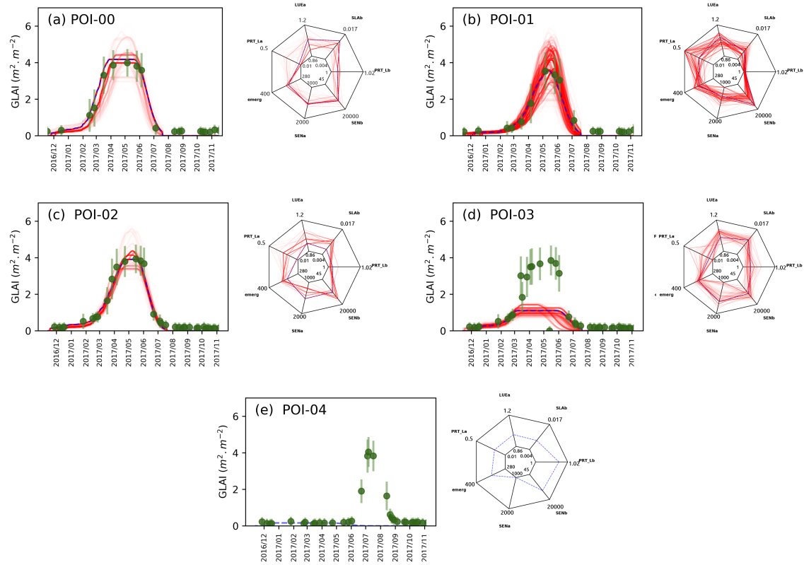
Figure 7. Time series of GLAI , and radar plots containing the free parameters of SAFYE-CO 2 . Simulations are represented in red with a transparency proportional to their relative likelihood and the maximum likelihood simulation is represented in blue dashed lines. POI-00 (a) and POI-01 (b) are located in the same field. POI-02 (c) and POI-03 (d) are adjacent pixels where a cloud date is not filtered in (d). POI-04 (e) illustrates either an error in the CAP declaration or a failed wheat crop followed by a summer crop .
