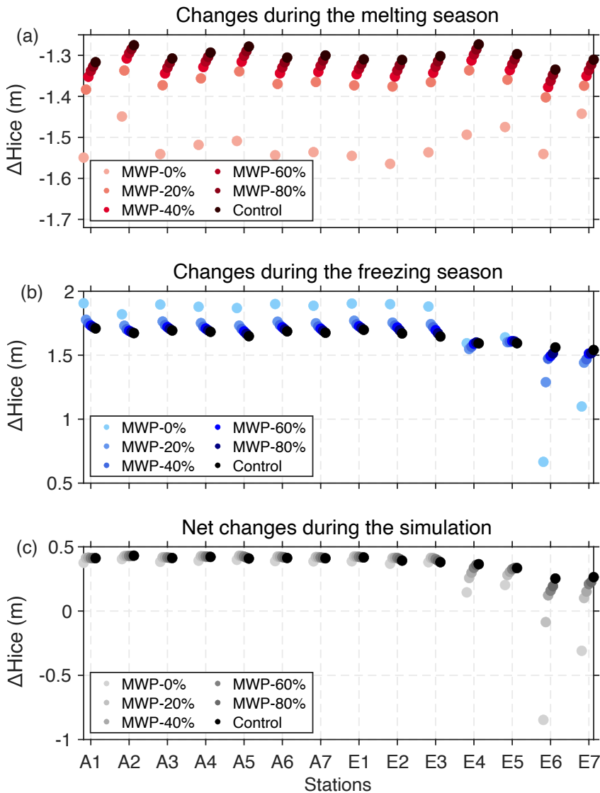
330 Figure 11: Ice thickness change during model simulation for all stations. (a) Effective ice thickness change during the melting season. The melting season for each experiment is defined as the period from maximum thickness in May to minimum thickness in September. (b) Effective ice thickness change during the freezing season. The freezing season for each experiment is defined as the period from minimum thickness in September until the end of the simulation.
