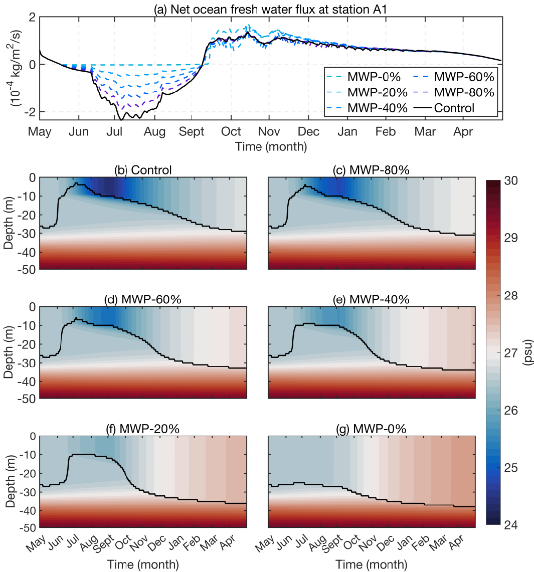
190 Figure 3: Simulated net ocean fresh water flux and time series of upper 50 m salinity at station A1. (a): Time series of net fresh water flux at sea surface (the sum of freshwater fluxes caused by ice melting/freezing and surface freshwater forcing). The negative values represent the freshwater entering the ocean. In the legend, ~% refers to the magnitude of the melt water input anomaly in the MWP runs. (b): Time series of the upper 50 m salinity for the control run at station A1. (c)-(g): Time series of upper 50 m salinity for MWP runs at station A1. The black lines in (b)-(g) indicate the MLDS.
