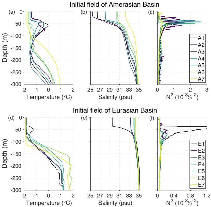
145 Figure 2: The observed temperature (a, d) and salinity (b, e) profiles obtained from ITPs in the Arctic Ocean, which are used as the initial profiles in the model. The corresponding buoyancy frequency values (c, f) for each station are also displayed. The time of observation for each station is shown in Table 1.
